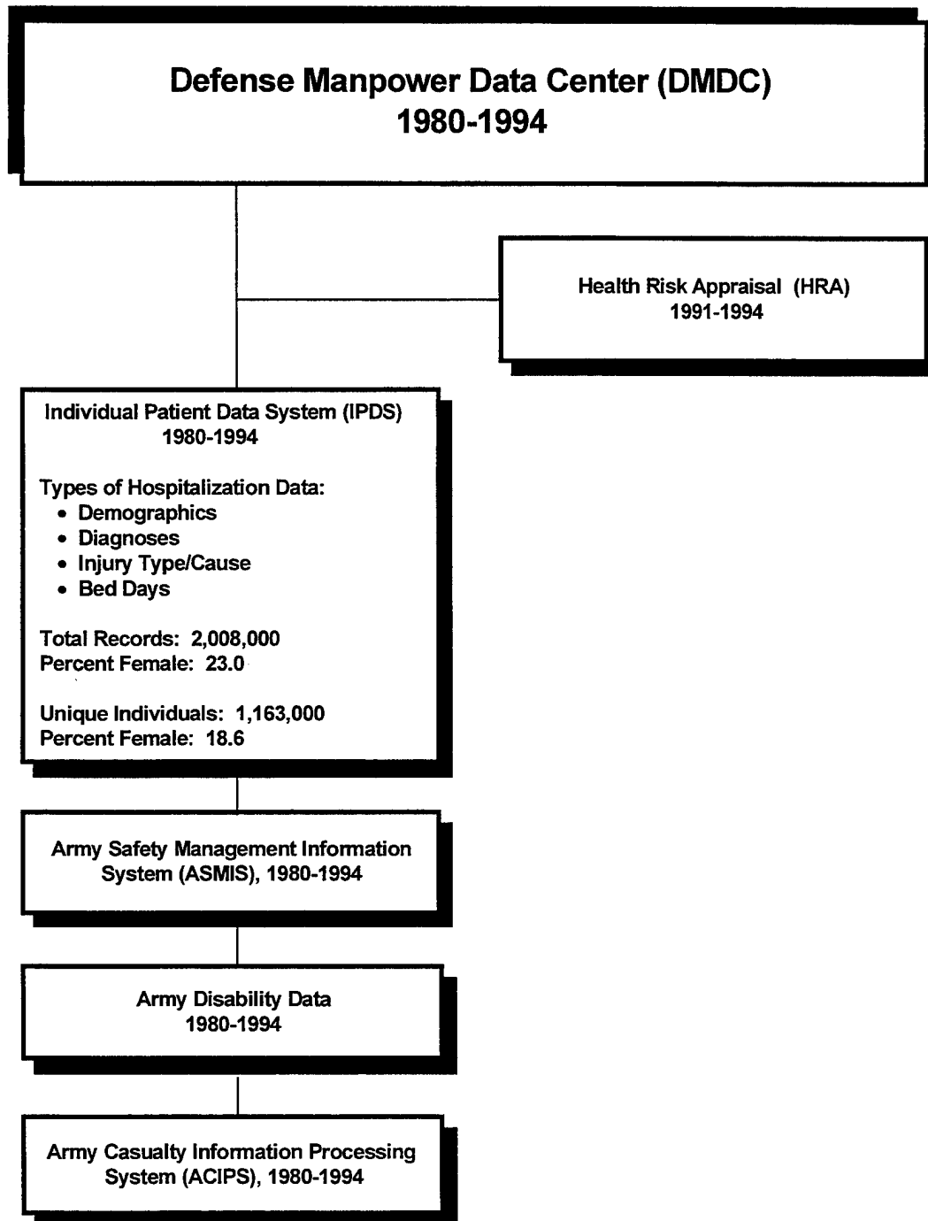
FIGURE 3 HOSPITALIZATION DATA
