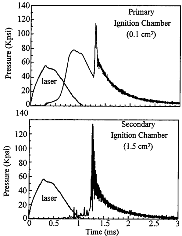
Figure 5. Pressure-time records from initiator when two stages are ignited.
