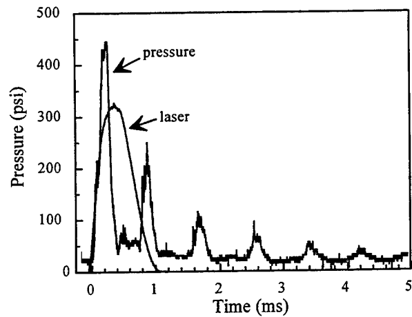
Figure 7. Water doped with graphite in 5-cm 3 chamber.
