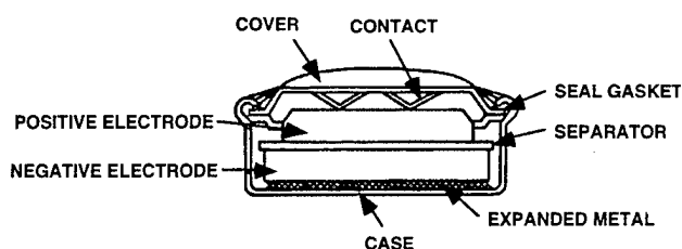
Figure 6-9. Button Cell Configuration
