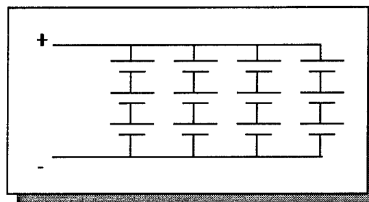
Figure 6-3. Battery Cells in Series-Parallel
