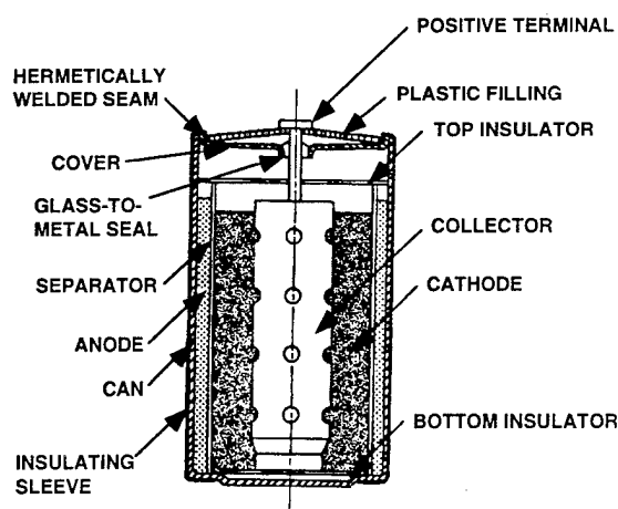
Figure 6-8. Cylindrical Cell Bobbin Configuration
