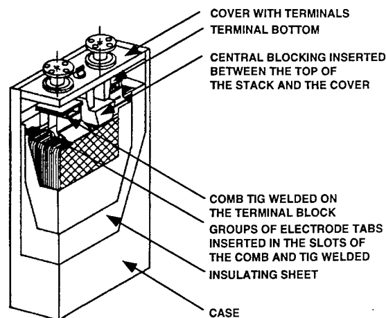
Figure 6-10. Prismatic Cell Configuration
