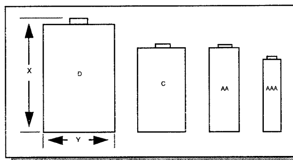
Figure 6-6. Cylindrical Cell Configurations
