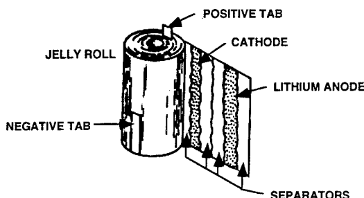
Figure 6-7. Cylindrical Cell Assembly
