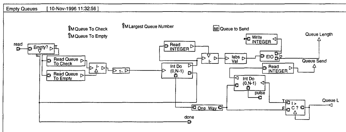
Figure 3.13 Empty Queues
