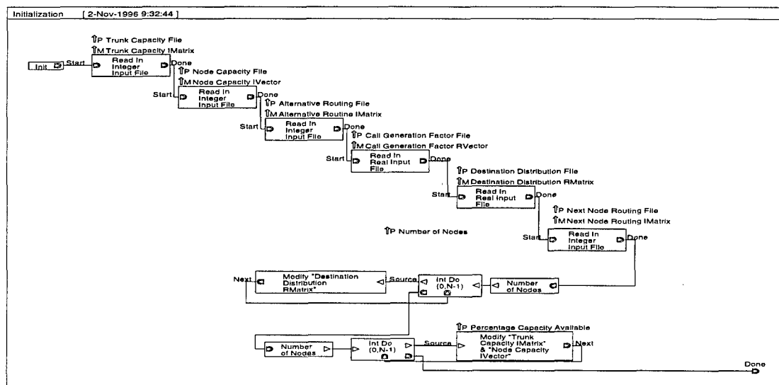
Figure 3.4 Initialization Block
