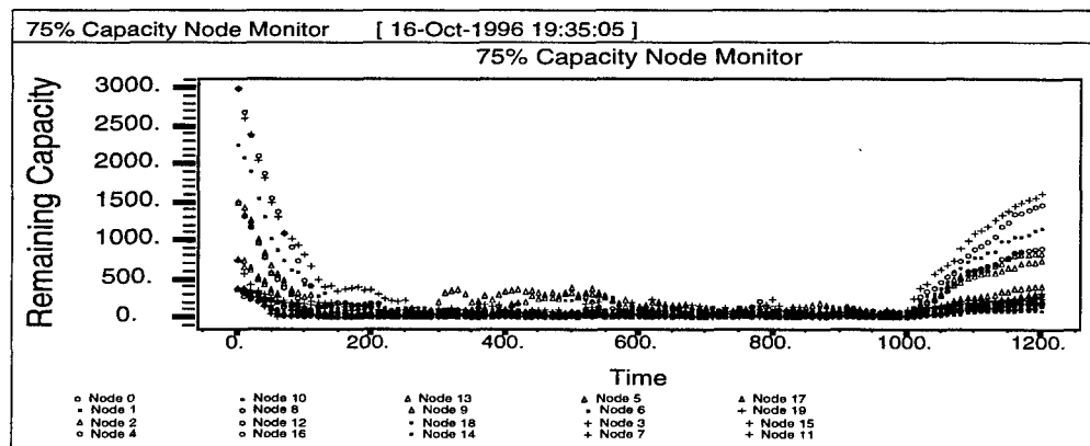
Figure 3.23 Node Monitor
