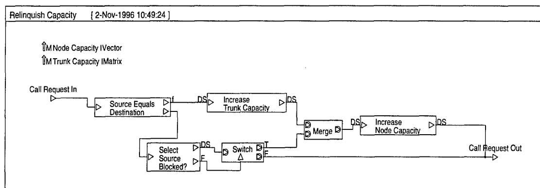
Figure 3.9 Relinquish Capacity
