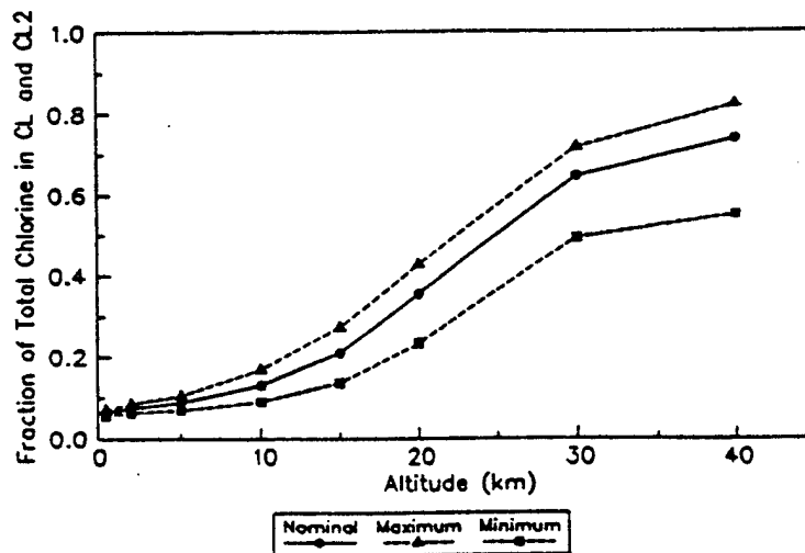
Figure 2-3. Effects of chemical rate constant variations on Cl and Cl 2 Production (10:14)
