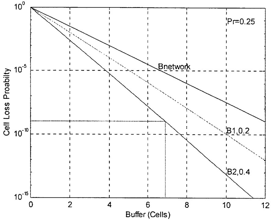
Figure 13. Buffer allocations for normalized loads 0.2 and 0.4.
