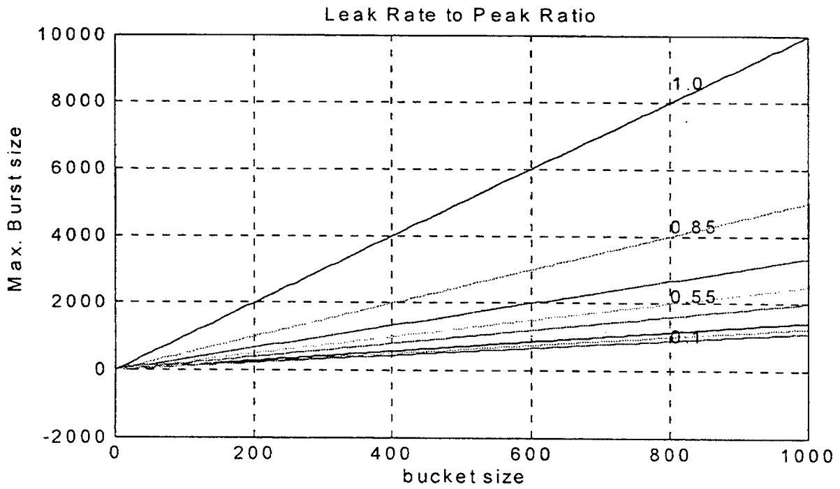
Figure 8. Effect of maximum burst size on leaky bucket parameters.
