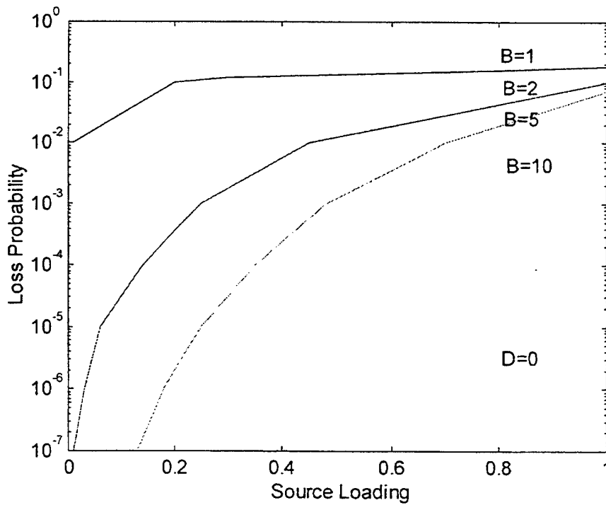
Figure 4. Source loading vs. CLP for zero data buffer.
