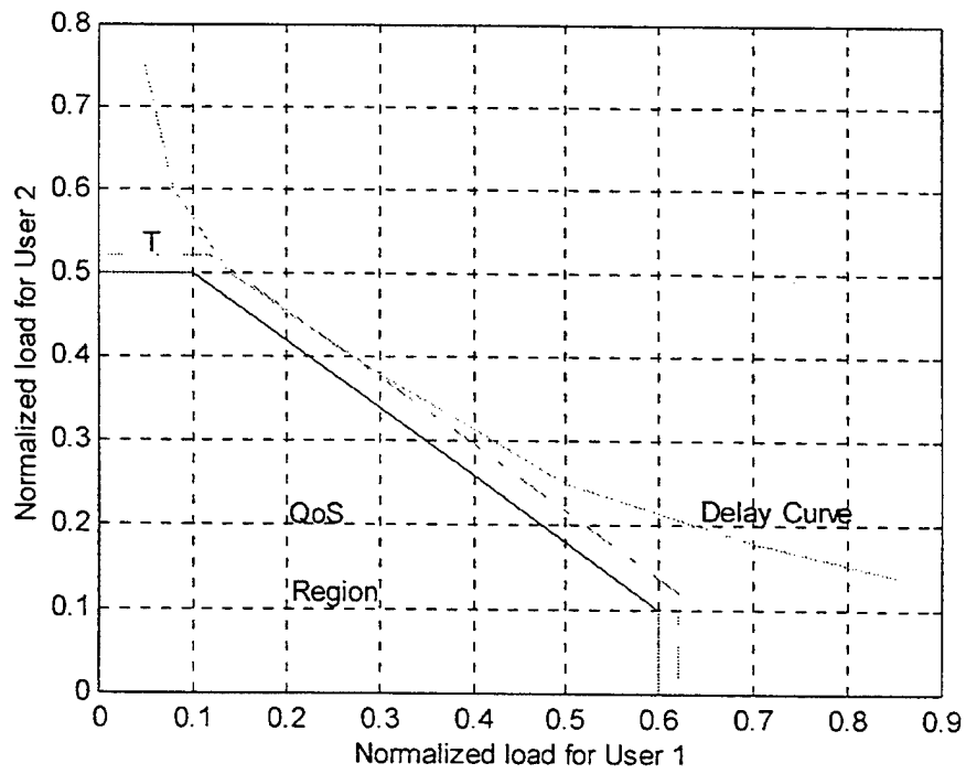
Figure 12. Disjoint region between capacity and QoS.
