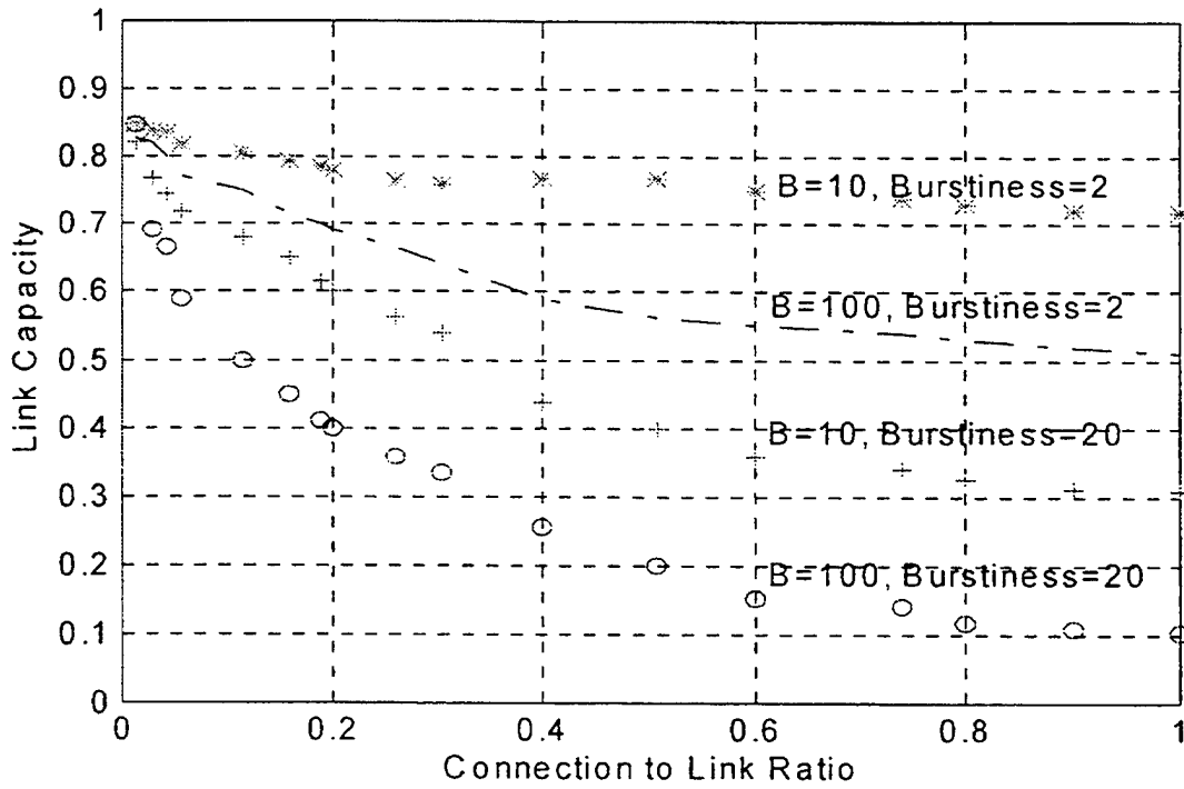
Figure 10. Admission control example.
