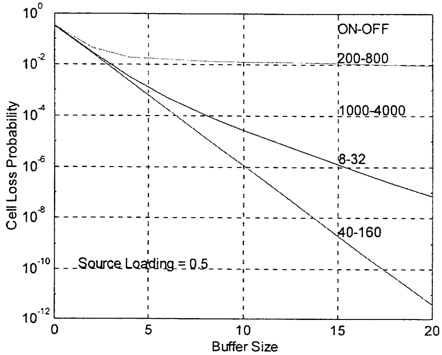
Figure 9. Effects of ON-OFF period.
