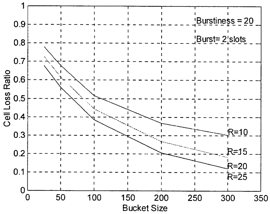
Figure 6. Trade-off between bucket size and leak rate.
