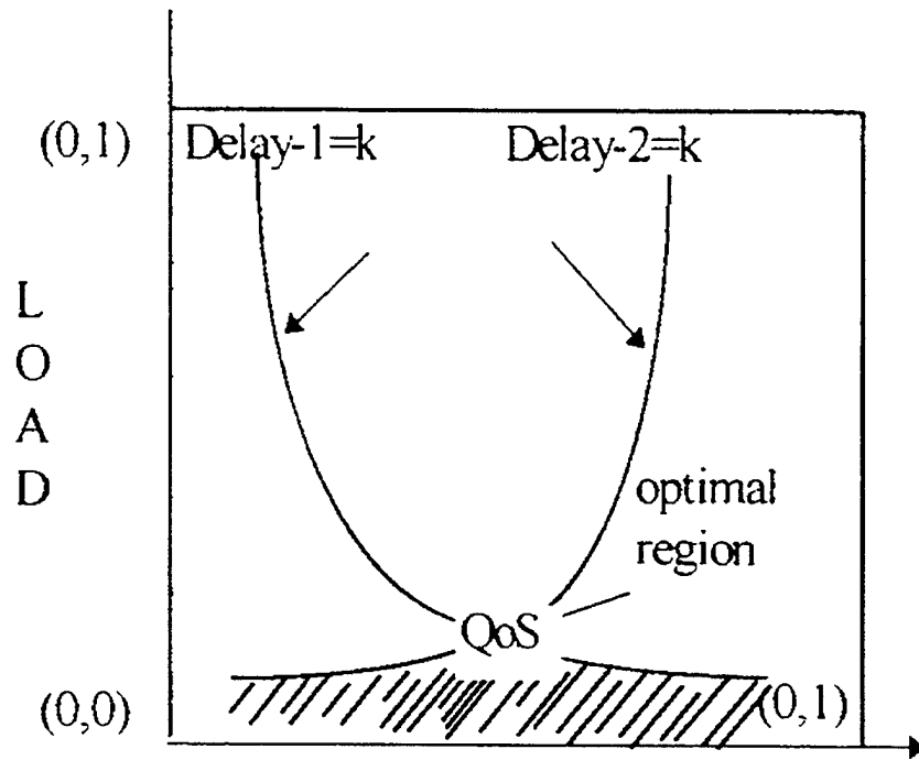
Figure 11. Load delay plane.
