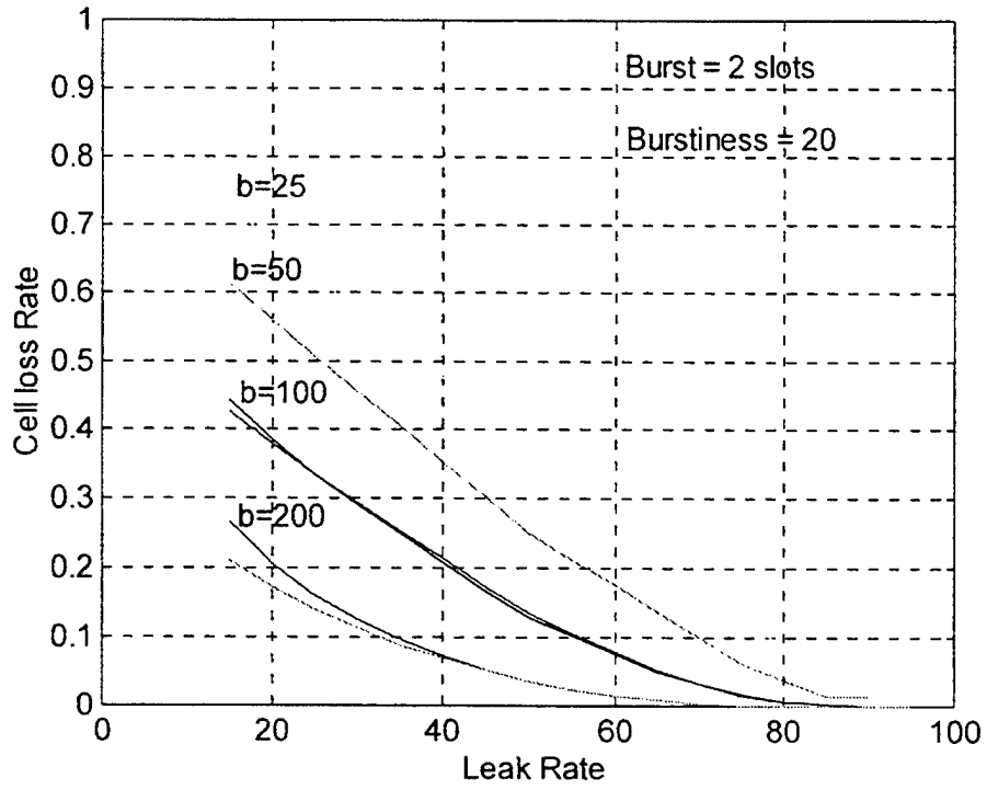
Figure 5. Analysis and simulation results.
