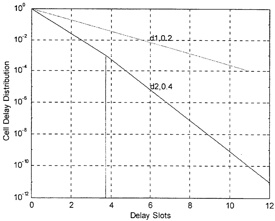
Figure 14. Delay requirements for normalized loads 0.2 and 0.4.
