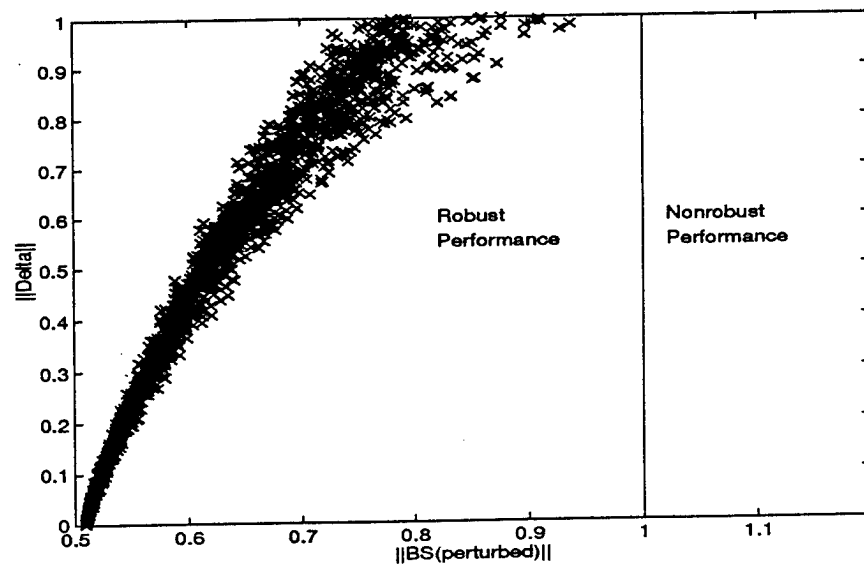
Figure 4: \|BS_{\text{perturb}}\| for perturbations \Delta . The robust performance region is the area to the left of the line segment at \|BS_{\text{perturb}}\| .
