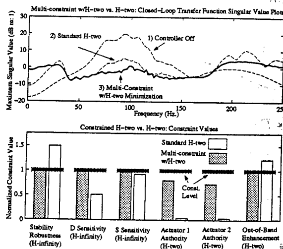
Figure 4: Multi-constraint H^2/H^2 , with H^2 -minimization, compared to standard H^2 controller synthesis. The singular value plot shows disturbance-to-regulated-output transfer functions, and the bar chart shows the normalized values of the constrained transfer functions.
