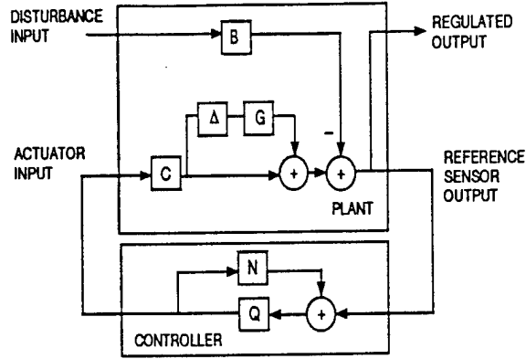
Figure 1: SISO disturbance-rejection configuration. The blocks are a simplification of our standard E, S, D, C representation. B is a performance weighting transfer function; C is the nominal coupling, and multiplicative variability in C is represented by the two blocks, \Delta and G . G is a constant variability weighting matrix, and \Delta is unknown but bounded. The controller is represented as a Q -parameterization.
