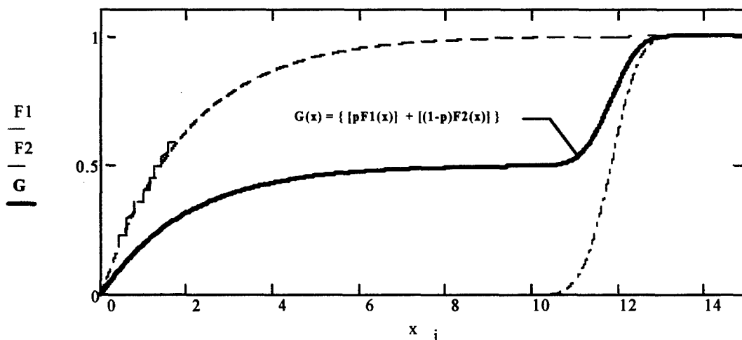
Figure 3. Mixed Weibull Cumulative Density Function
