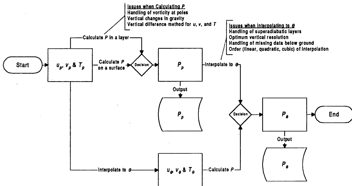
FIG. 1. Flow diagram of major issues and decisions addressed during IPV ( P ) algorithm development and implementation. u, v, and T are the horizontal wind components and temperature, respectively. Subscripts p and \theta represent isobaric and isentropic data, respectively.
