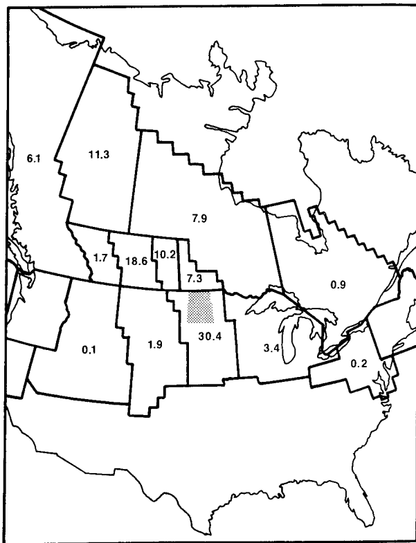
Fig. D-33. Percent derivation of the mallard harvest in Eastern North Dakota (shaded) from major breeding reference areas.
