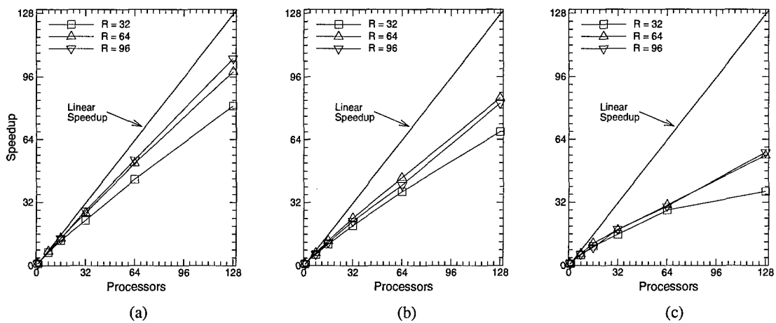
Figure 4.12: Three-Dimensional Speedups: a) T3D, b) Paragon, c) SP2
