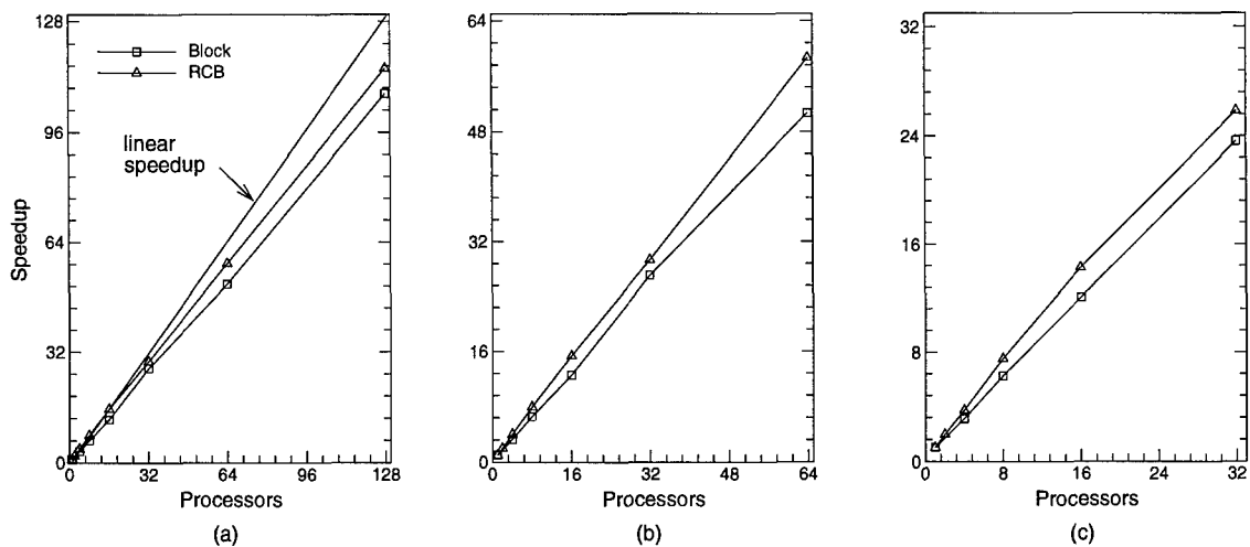
Figure 5.7: Speedup Results: a) Paragon, b) T3D, c) SP2
