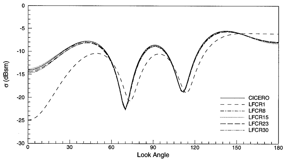
Figure 6.5: Sample LFCR RCS Results (VV polarization)
