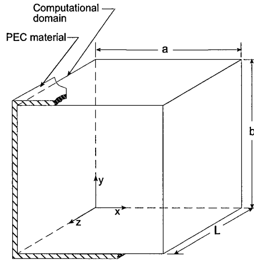
Figure 4.4: Rectangular Waveguide Geometry
