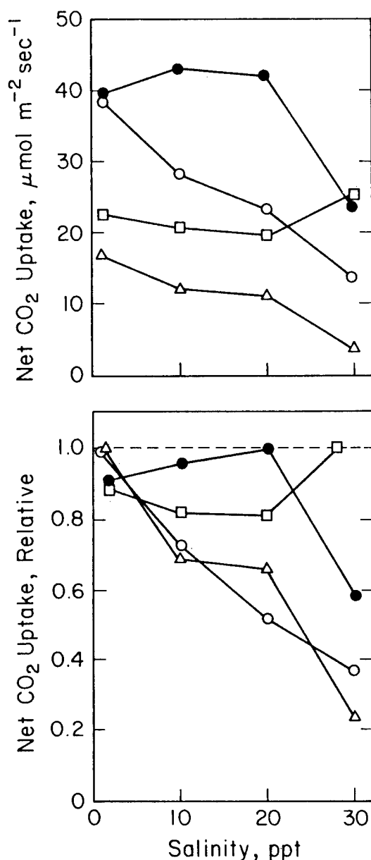
Figure 41. TOP: Effect of salinity on mean \text{CO}_2 uptake for various marsh plants. Filled circle = Pacific cordgrass; open circle = alkali bulrush; open square = pickleweed; open triangle = brass buttons. BOTTOM: Relative photosynthetic \text{CO}_2 uptake as a function of salinity. Rates plotted relative to the maximum rate for each species. Measurements made at 320 \mu\text{bars} \text{CO}_2 pressure, photon flux densities of 1.7–2.0 \text{mmol}/\text{m}^2/\text{sec} , leaf temperatures of 30°C and VPD of 5–10 mbar. Each point represents mean of 2–8 leaves. From Pearcy et al. 1981.
