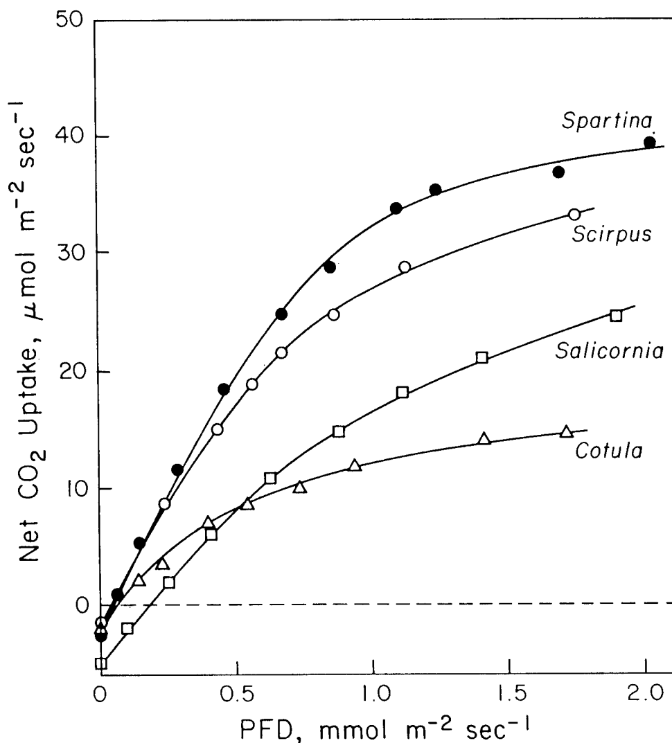
Figure 40. Photosynthetic CO 2 uptake as a function of light intensity. Measured at 30°C leaf temperatures, 320 μbar CO 2 pressures, and a vapor pressure differential of 5–10 ubar (from Pearcy et al. 1981).
