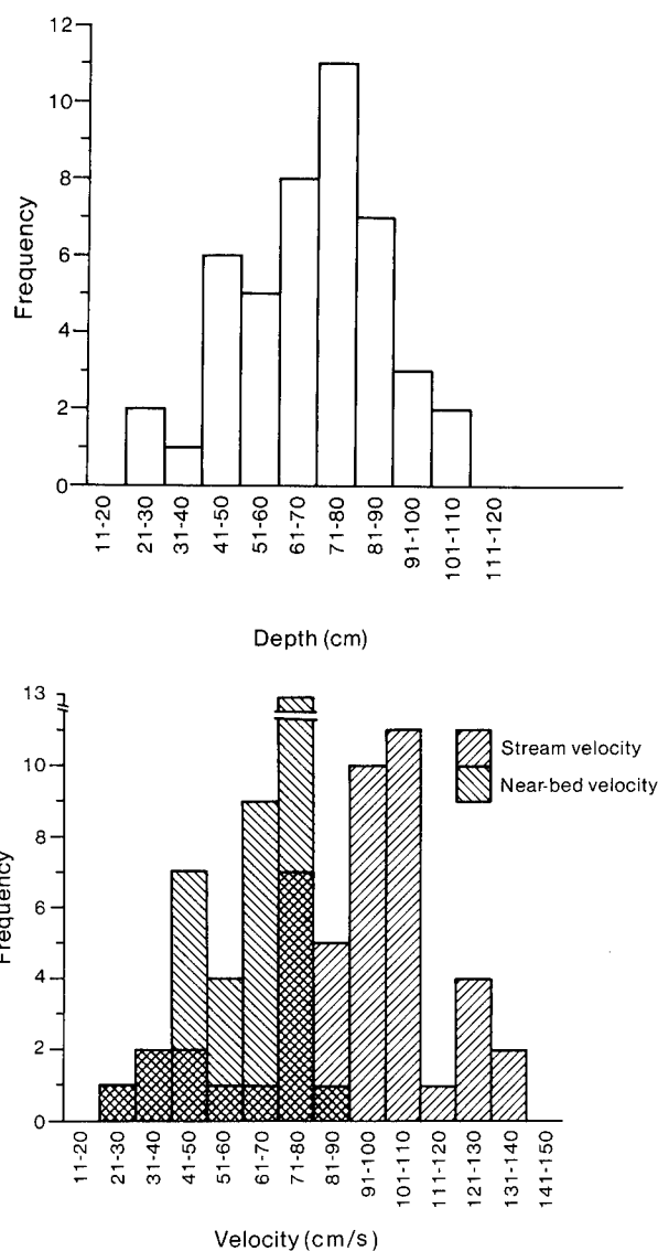
Fig. 6. Frequency of use of spawning sites as a function of stream depth, stream velocity, and near-bed velocity, 1982-84.
