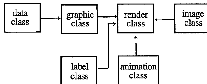
Figure 5. Class relationships.
