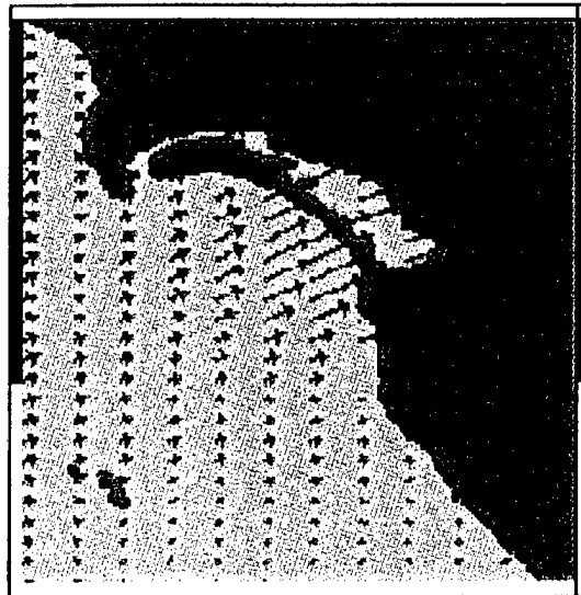
Wind Stress
