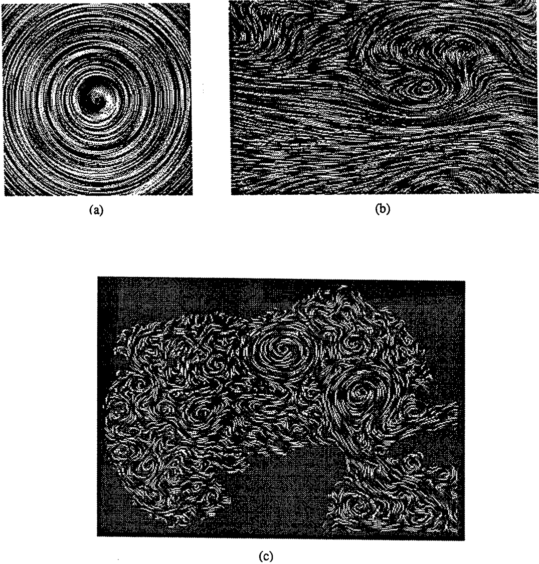
Figure 8. FM Texture mapping: a) a synthetic circular flow field of 280 x 280, b) a horizontal wind field of 264 x 210, and c) an ocean circulation field of 194 x 146.
