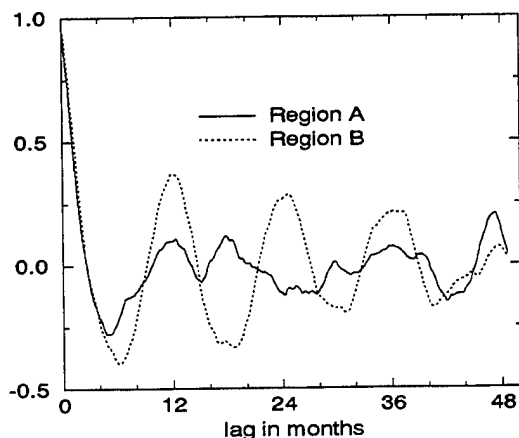
Figure 3. Auto-correlation function of the time sequences of the number of tracked eddies.
