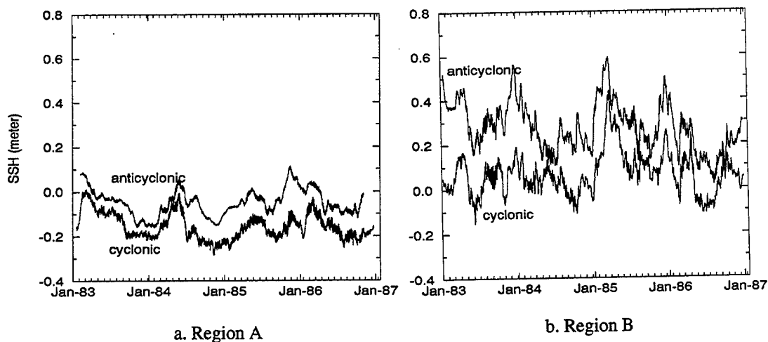
Figure 4. Sea-surface height at the eddy centers.
