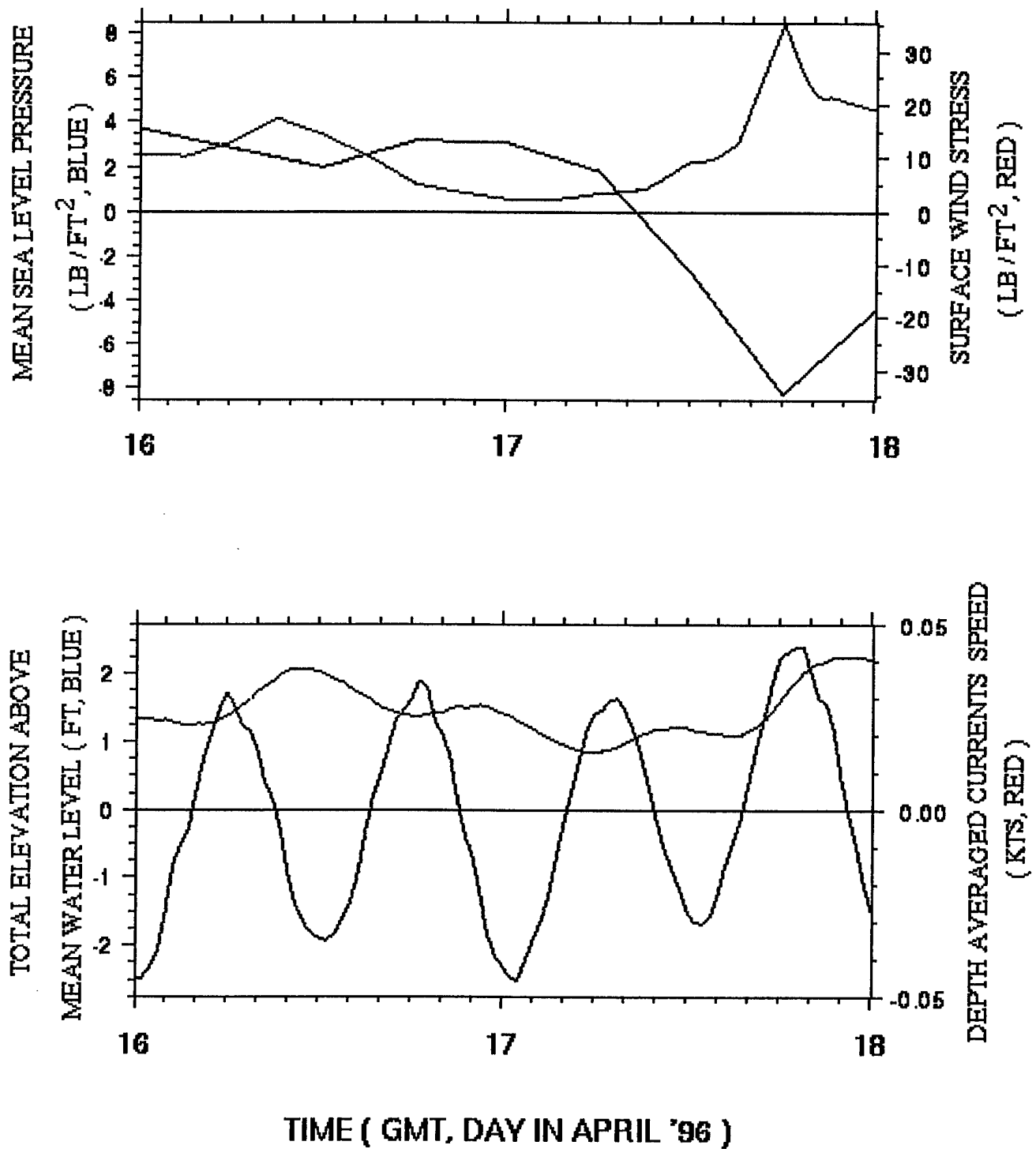
Figure 6. Time Series plots for Monrovia ( Coarse Grid )
