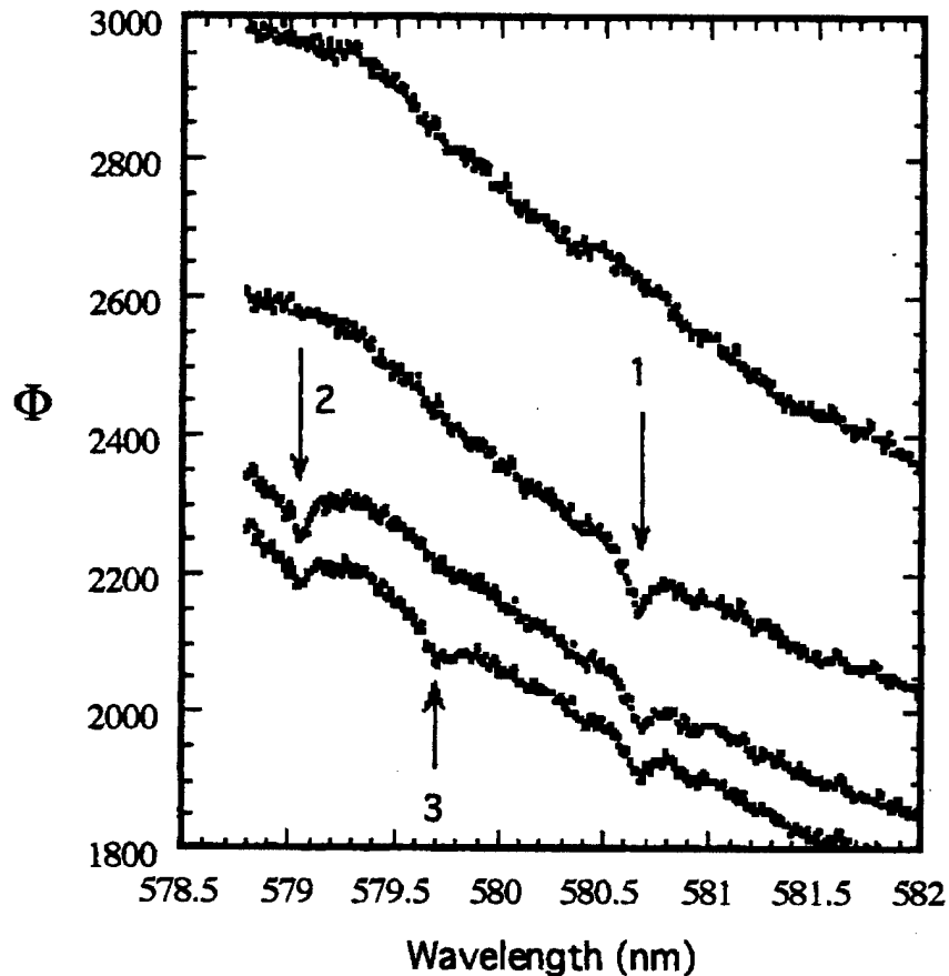
Fig. 1 Successive hole-burning fluorescence excitation spectra for a 2-D layer of polystyrene particles 5\mu\text{m} in radius.
