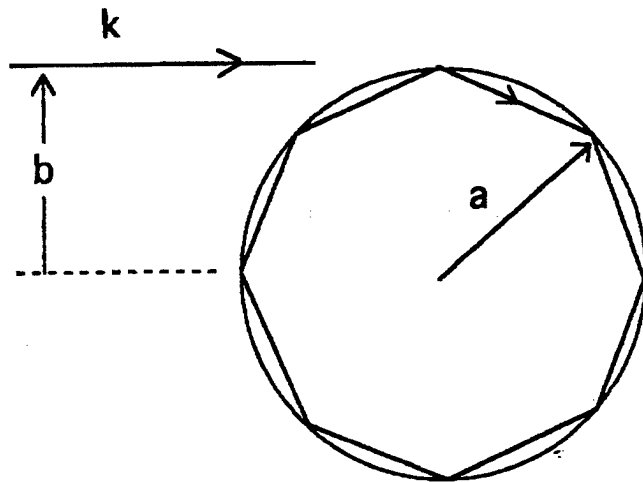
Fig. 4 Stimulation of a "geometrical" resonance by an external ray.
