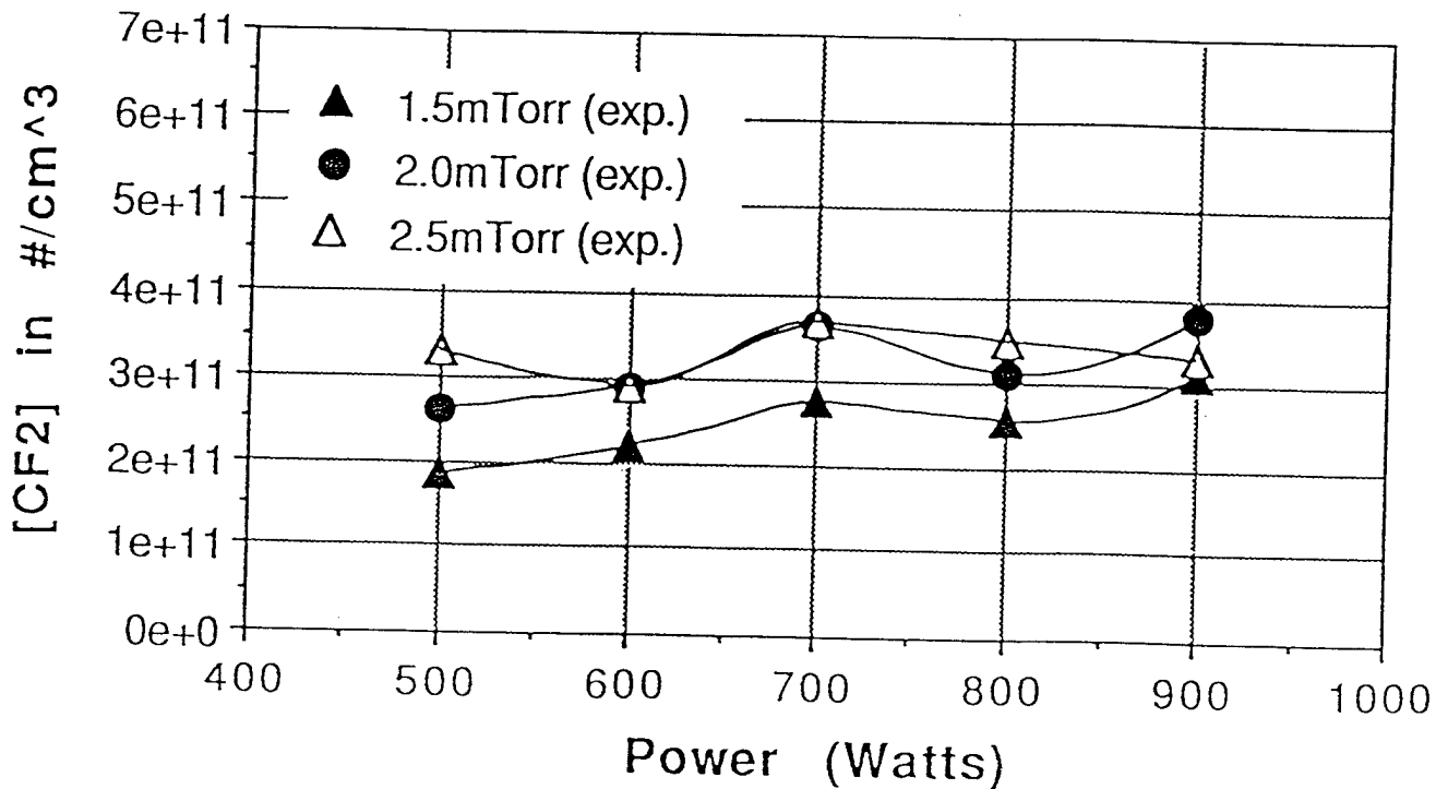
Fig. 4.2 F and CF_2 densities in an ECR CF_4 discharge measured by K. Ashtiani.
