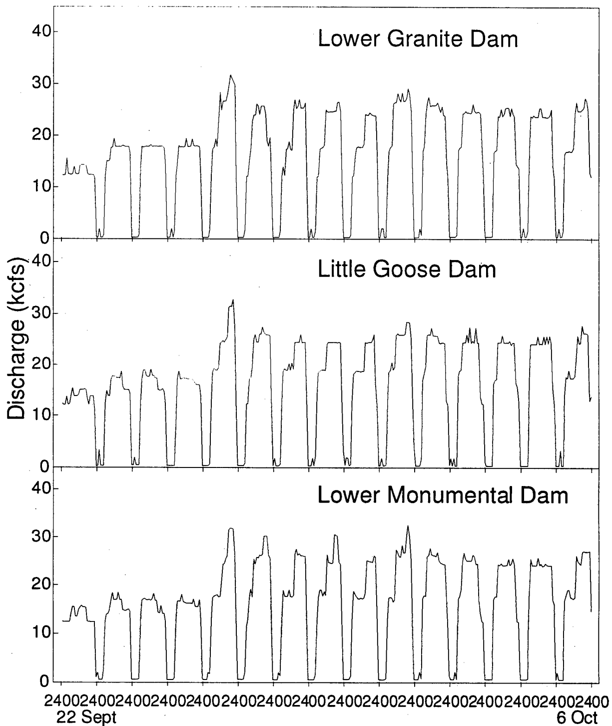
Figure 46. Discharges from the three upper dams in the lower Snake River during the two-week period from 22 September to 6 October 1992 when flows were reduced to near zero from about 2300 to 0600 hr each night.
