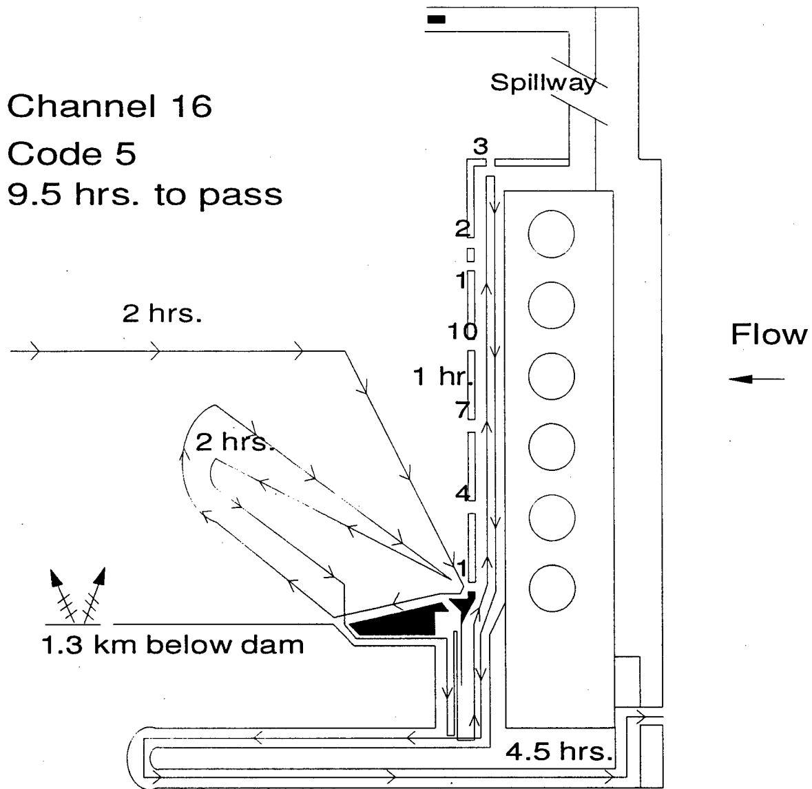
Figure 37. Diagram of Lower Granite Dam with an illustration of the types of movements made by some steelhead in the fall of 1992 when approaching the dam and passing through the fishway.
