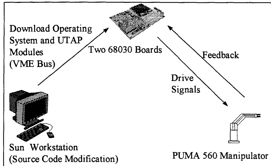
Figure 1: Laboratory Hardware
