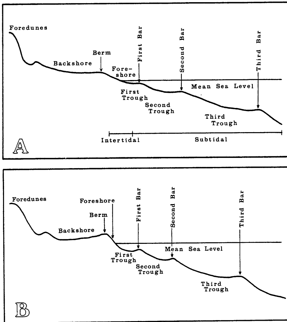
Figure 2. Profile of typical beach bar-trough system (A) and that found in the Big Shell area (B).
