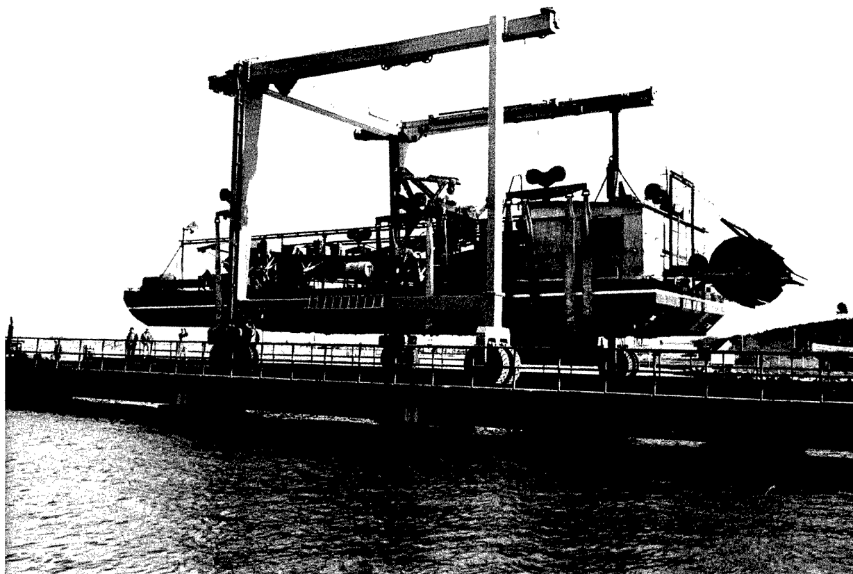
Fig. 6.1. Marine lift in South Humboldt Bay launching a commercial oyster dredge.
