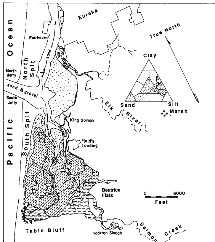
Fig. 2.3. Sediment distribution in South and Entrance bays (Thompson 1971).
