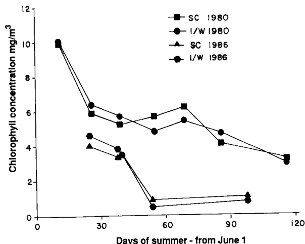
Fig. 2.15. Chlorophyll concentrations before (1980) and after (1986) cessation of wastewater discharge into Arcata Bay (Pequegnat 1988).
