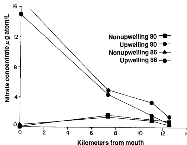
Fig. 2.13. Nitrate concentrations in Humboldt Bay waters during periods of upwelling and nonupwelling (Pequegnat 1988).
