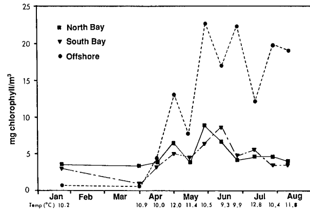
Fig. 2.14. Chlorophyll concentrations and water temperatures for offshore, North Bay (Arcata Bay), and South Bay during an 8-month period in 1979 (Pequegnat and Butler 1982).
