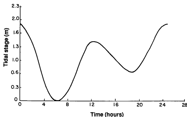
Fig. 2.8. Mean tide curve for South Jetty, Humboldt Bay (Costa 1982).
