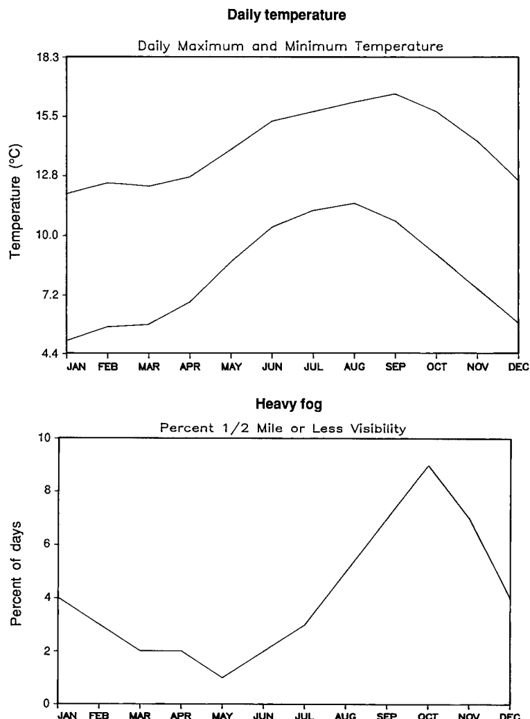
Fig. 2.5. Average daily maximum and minimum air temperatures, by month, and mean percent days of heavy fog (visibility 1/2 mile or less), by month, Eureka, California, 1941-70 (from USDC 1977).
