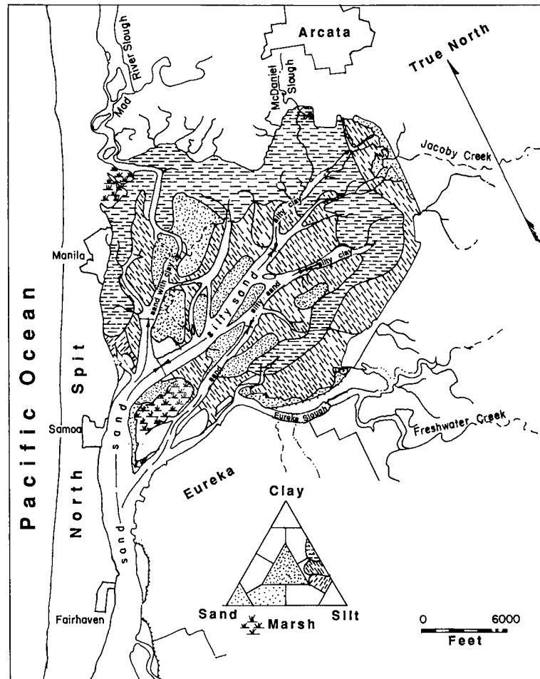
Fig. 2.2. Sediment distribution in Arcata Bay (from Thompson 1971).
