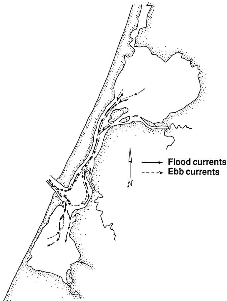
Fig. 2.9. Ebb and flood tidal current patterns for the major channels in Humboldt Bay (from Costa 1982).
