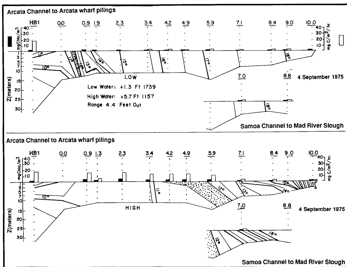
Fig. 2.11. Temperature, chlorophyll (black bar), and productivity distribution (white bar) at low and high tides in channels from Humboldt Bay entrance into Arcata Bay, 4 September 1975. Station HB1 is marker buoy 1 nmi off shore; station 0.0 is at mouth of Humboldt Bay; and all other stations are indicated by distance in nautical miles up bay from mouth (Pequegnat and Butler 1982).
