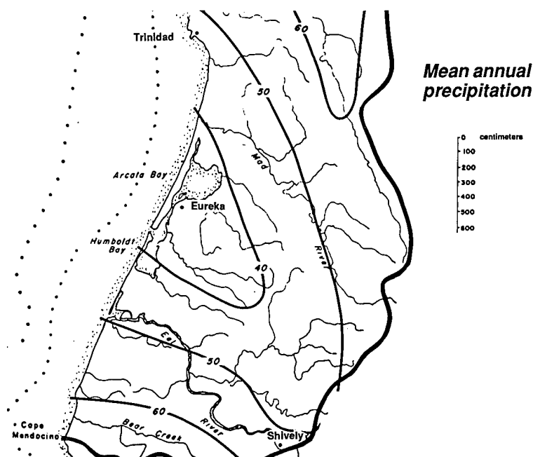
Fig. 2.7. Mean annual precipitation (inches), Humboldt Bay environs (from Proctor et al. 1980).
