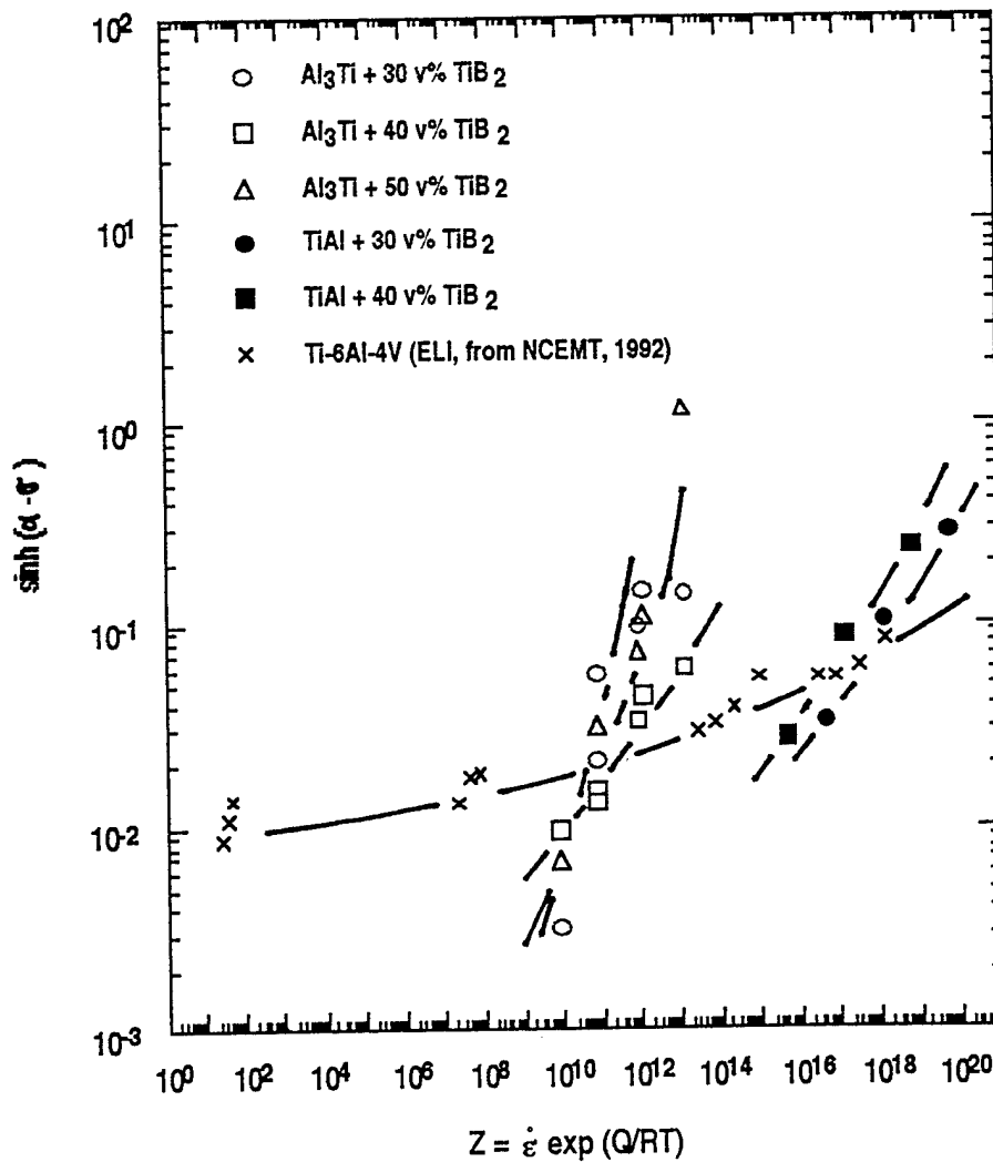
Figure 3-2. High temperature deformation of Ti-6Al-4V, and Al_3Ti and TiAl with 30, 40 and 50 v% TiB_2 .
