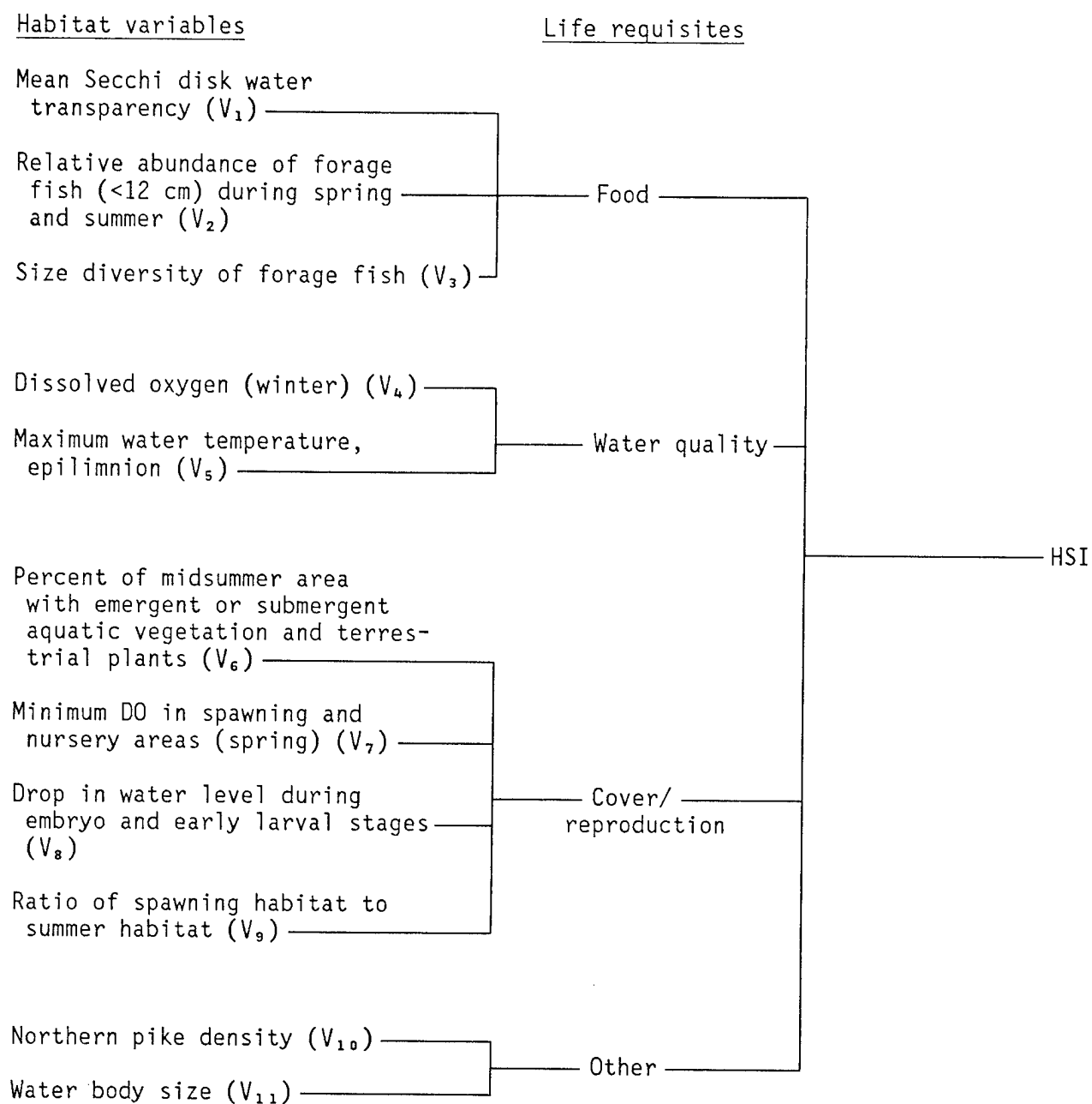
Figure 1. Tree diagram illustrating relationships between model variables, model components (life requisites), and HSI for the muskellunge in lacustrine environments.
