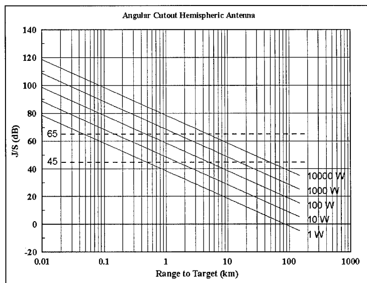
Figure 14. J/S ratio vs. range-to-go
