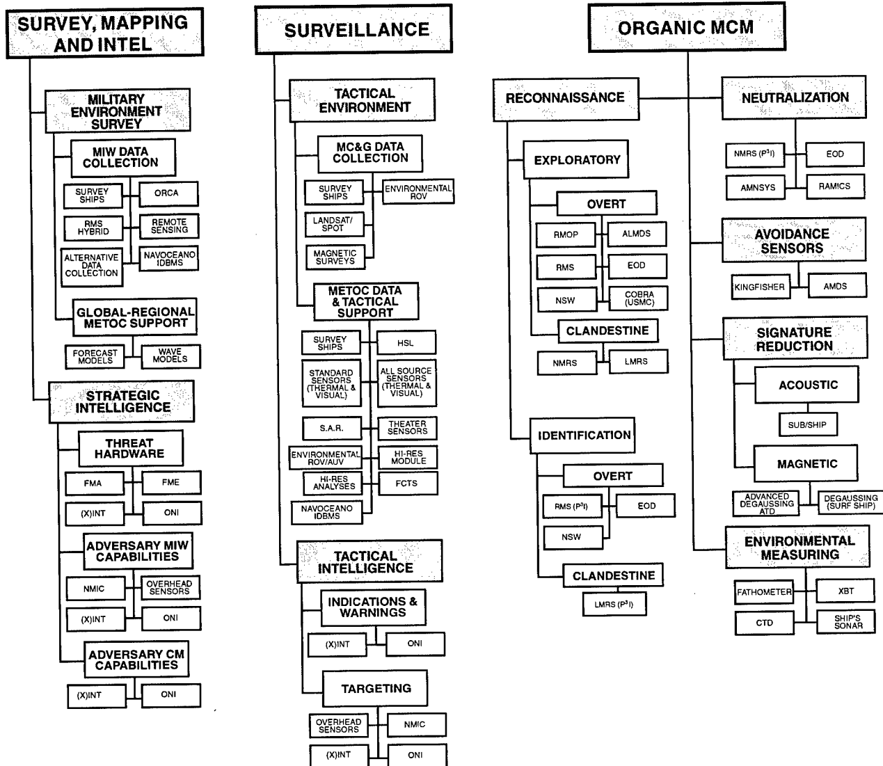
Figure 9. Allocation of MCM components and systems
