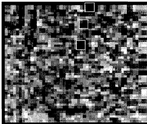
Figure 6. Small box fractal dimension
