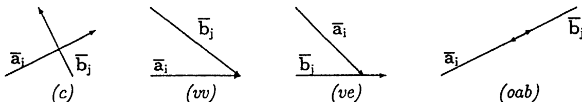
Figure 3. Various types of meetings of two edges
