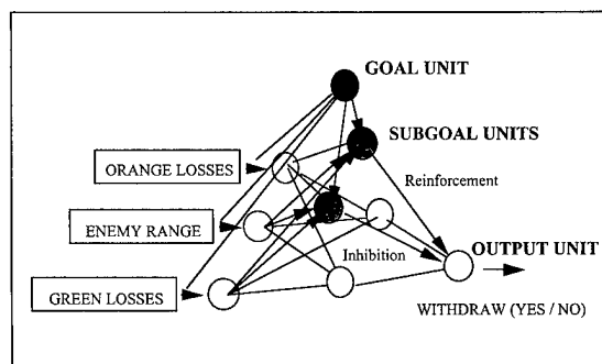
Figure 11. Adaptive Network
