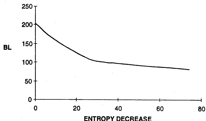
Figure 11. Plot of median Blue Losses (BL) versus cumulative entropy decrease.
