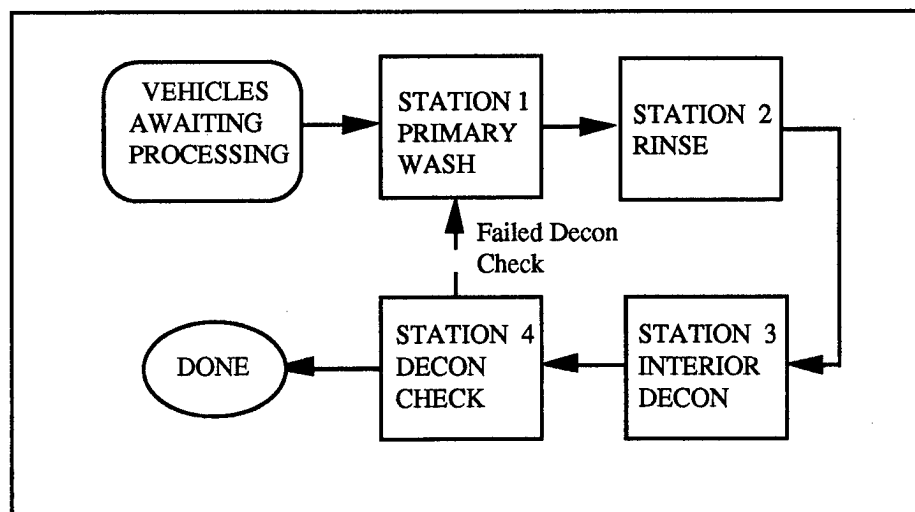
Figure 2. Flow Diagram of Detailed Nuclear Equipment Decontamination
