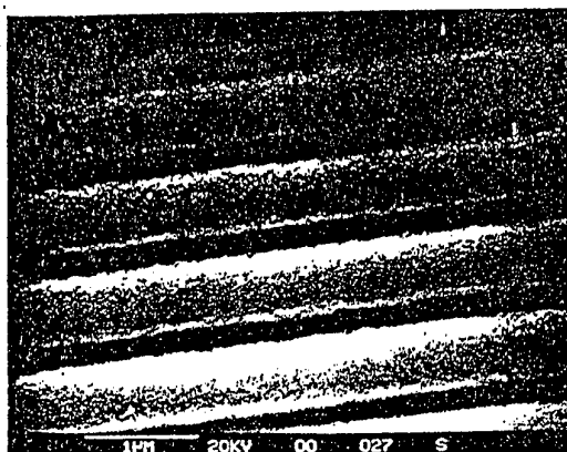
Figure D. Sol-gel silica replicated diffractive grating (line spacing is 0.9 μm).
