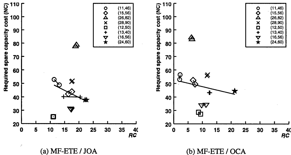
Figure 3-9. The effect of bandwidth reclaiming on required spare capacity cost
