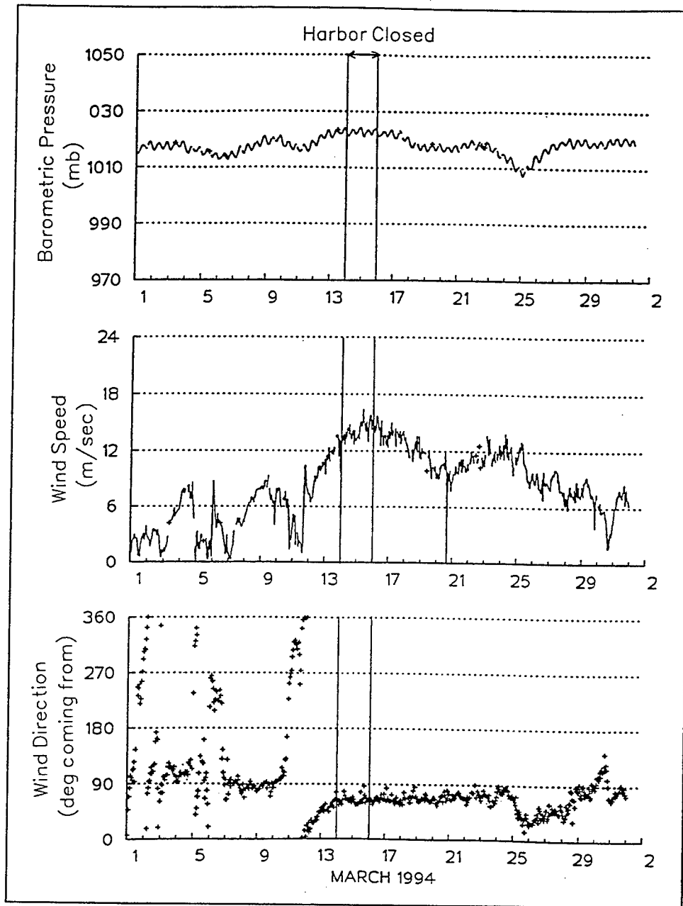
Figure 28. Harbor closing event; NDBC buoy meteorological parameters
