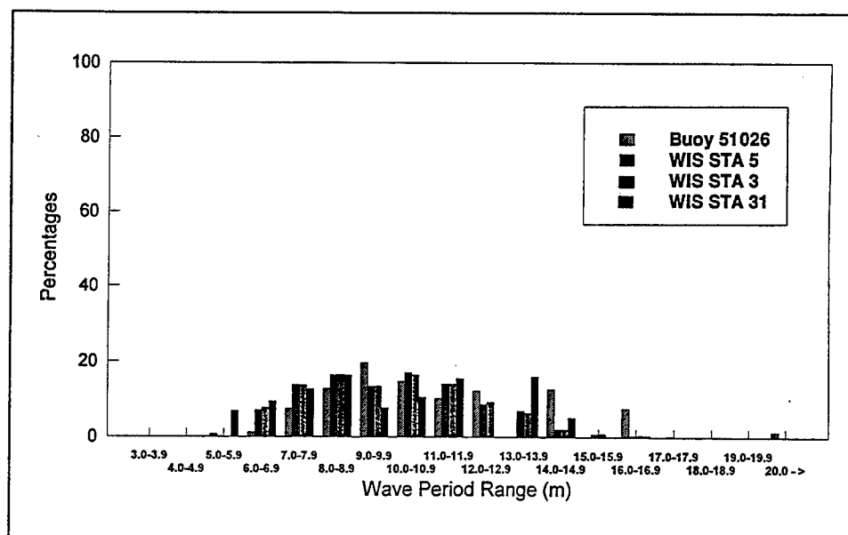
Figure 32. Deepwater wave climate comparison, T_p
