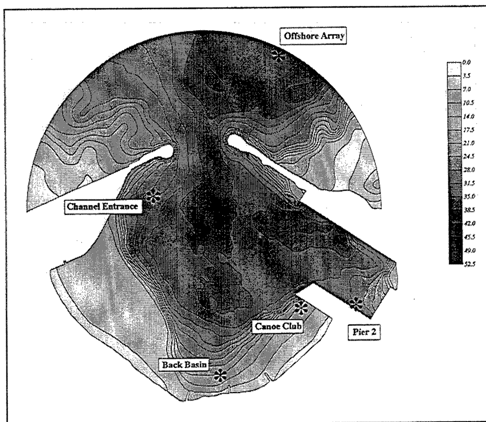
Figure 10. Field gage locations and bathymetry, in feet
