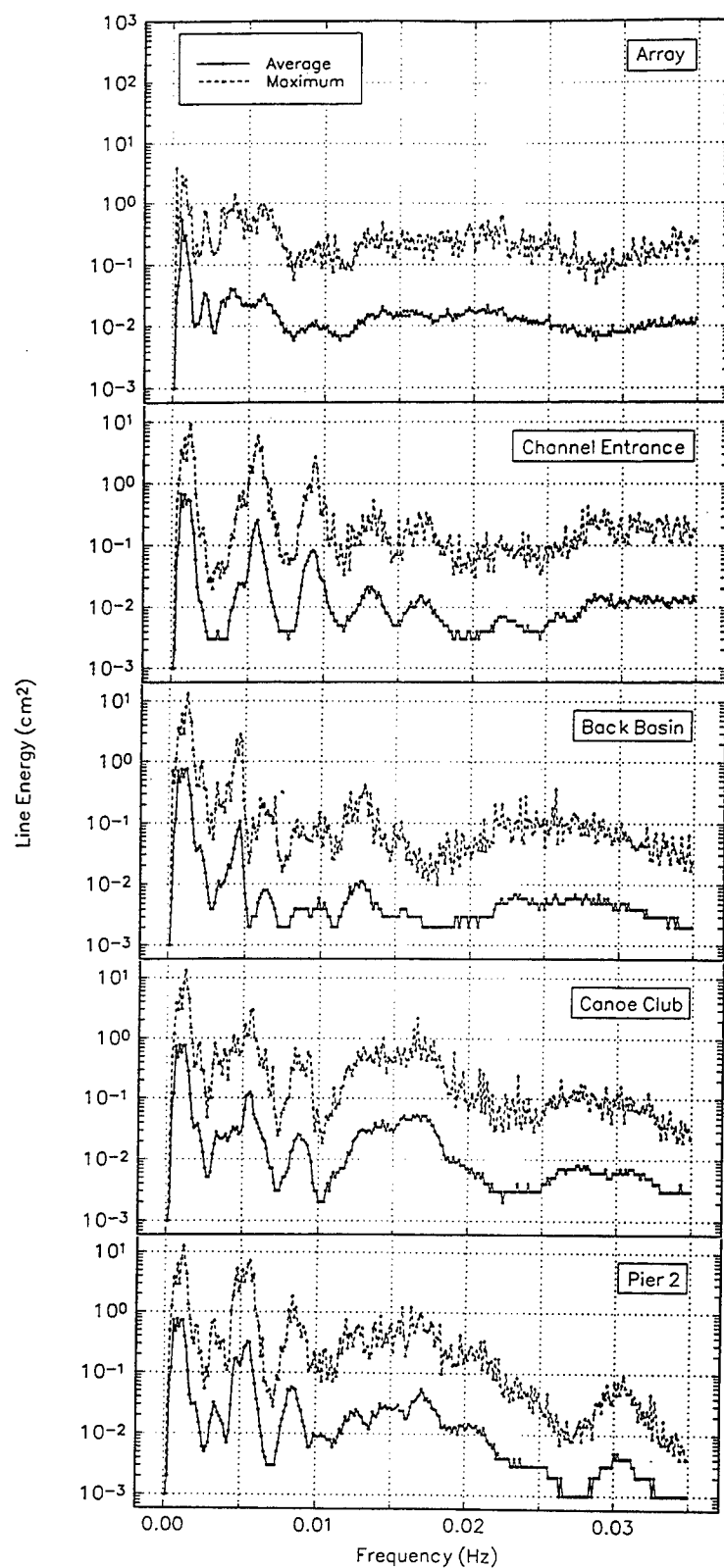
Figure 20. Average and maximum long wave spectra, Jan 94
