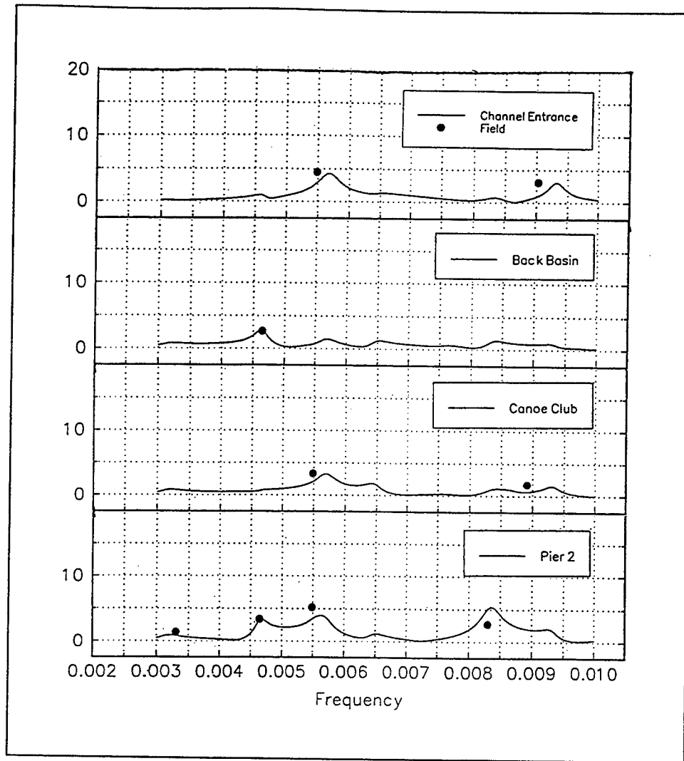
Figure 43. Model long wave calibration
