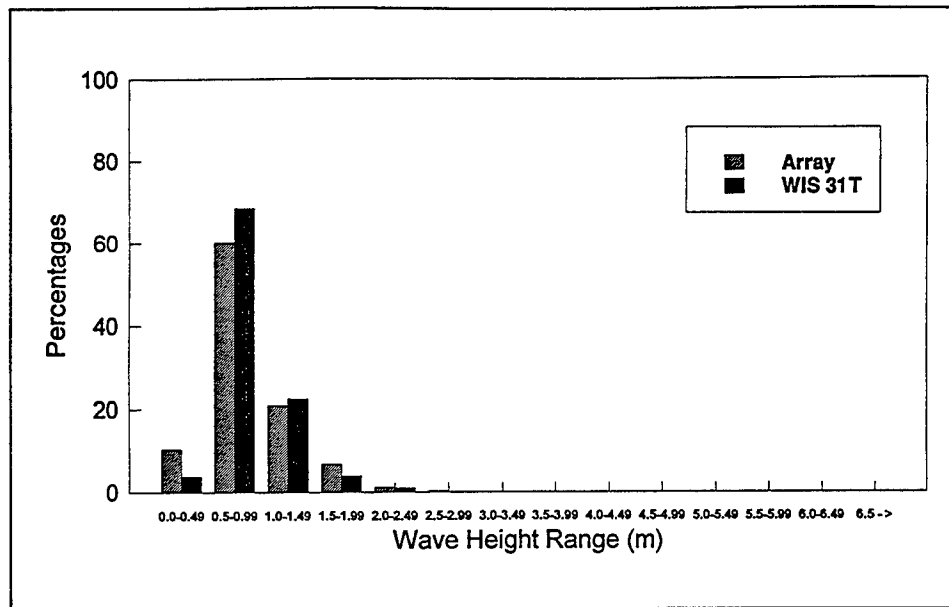
Figure 34. Harbor entrance wave climate comparison, H_s
