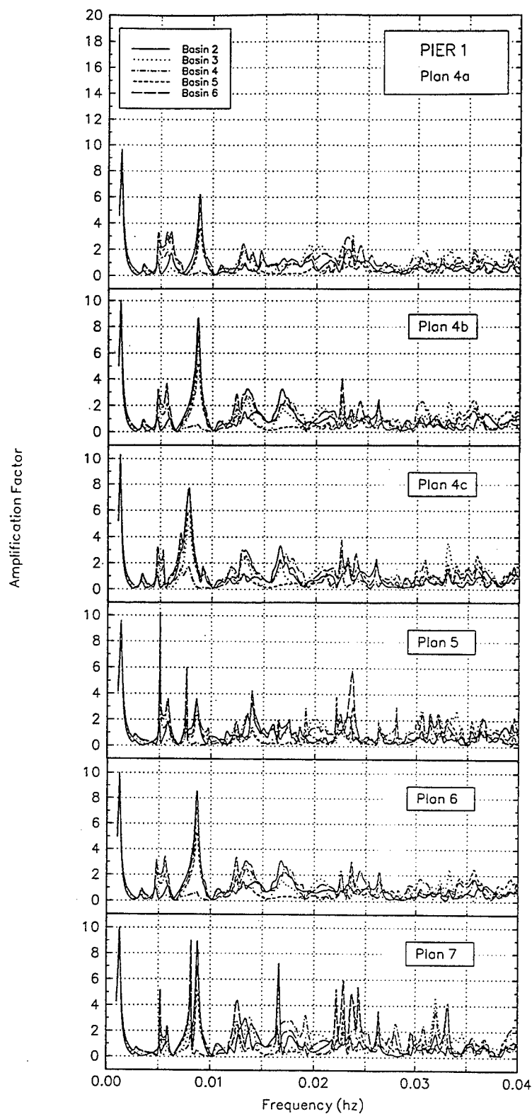
Figure G1. (Concluded)
