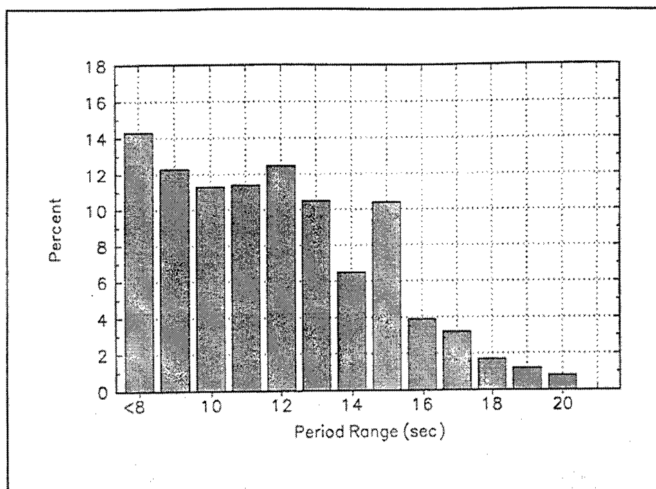
Figure 18. Probability distribution of (T_p)_{array} ; Nov 93-Sep 94, 1,785 observations
