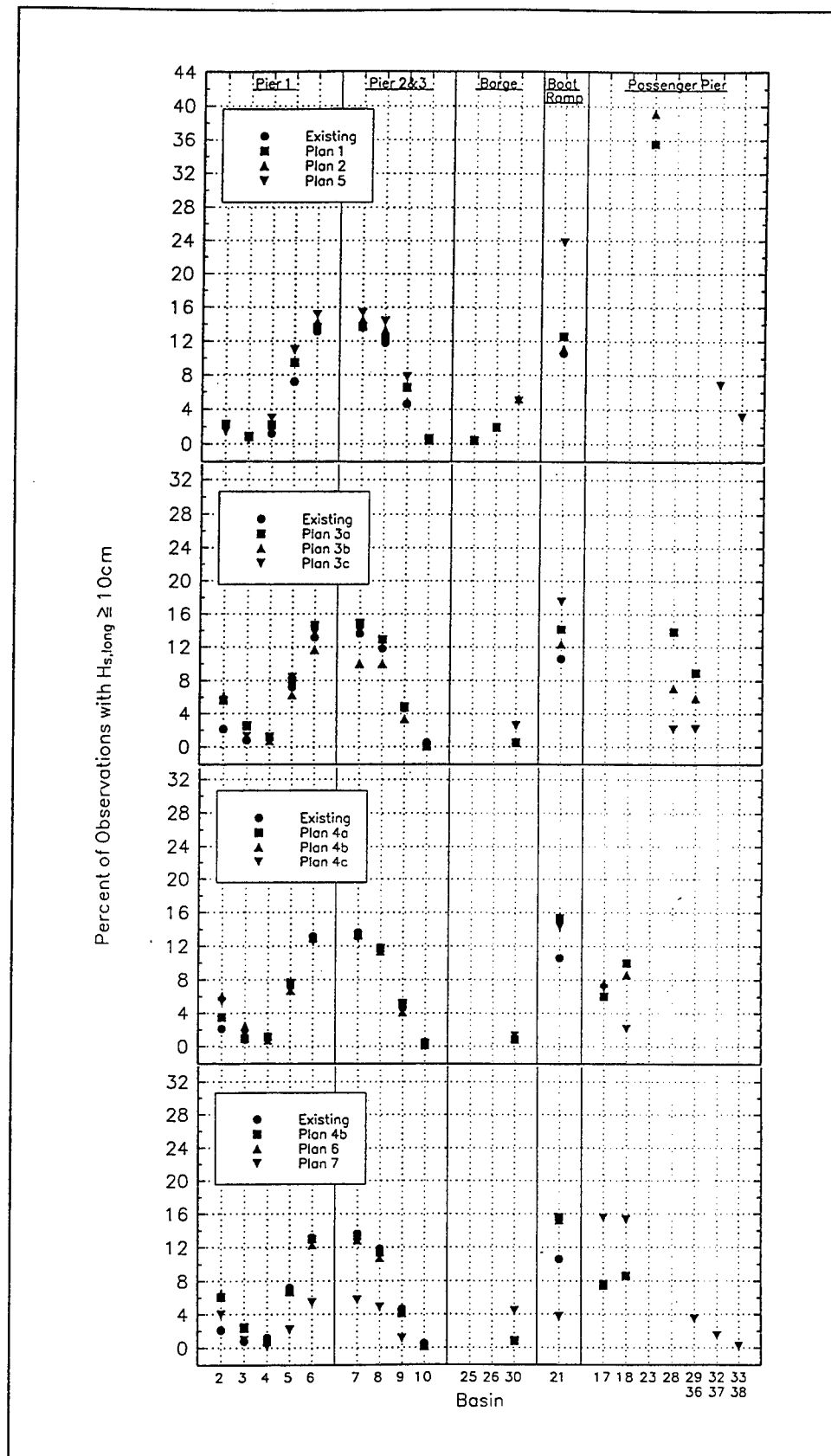
Figure 57. Percent occurrence of H_{s, long} \geq 10 cm at piers, T=100-400 sec
