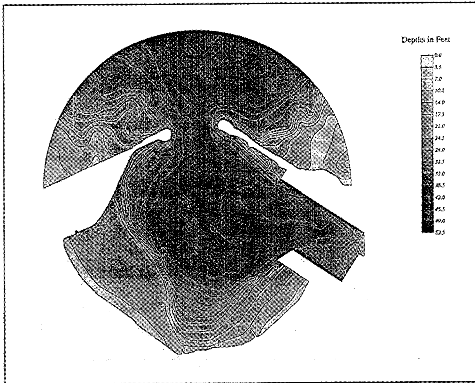
Figure 39. Bathymetry, existing harbor
