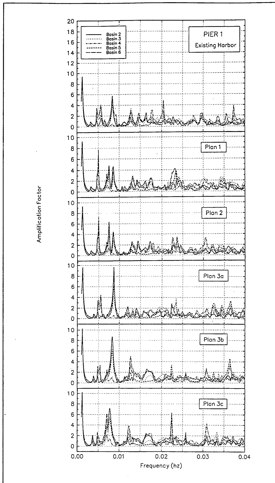
Figure G1. Long wave response, Pier 1 (Continued)
