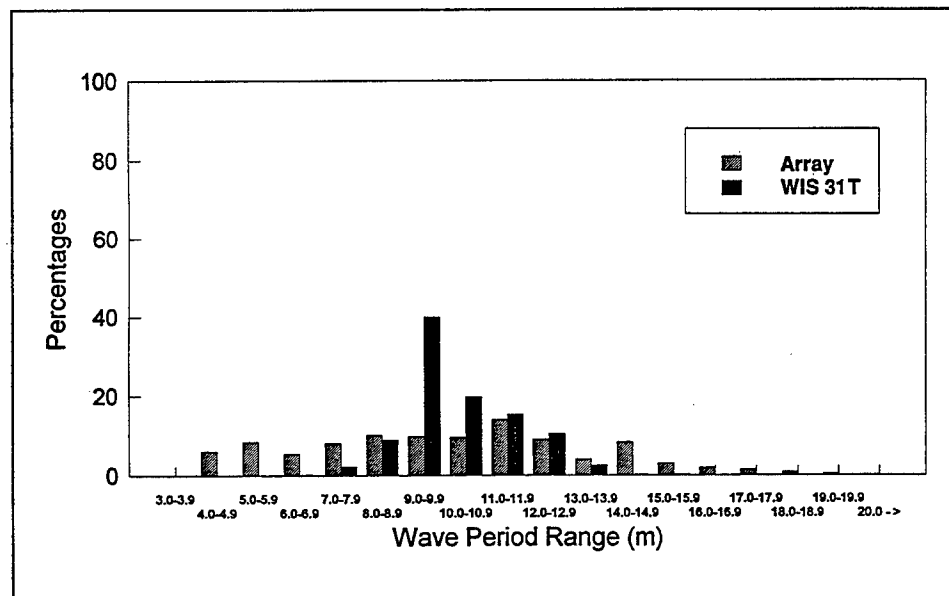
Figure 35. Harbor entrance wave climate comparison, T_p
