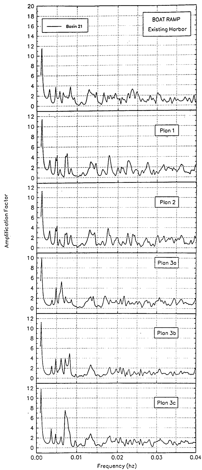
Figure G5. Long wave response, boat ramp (Continued)
