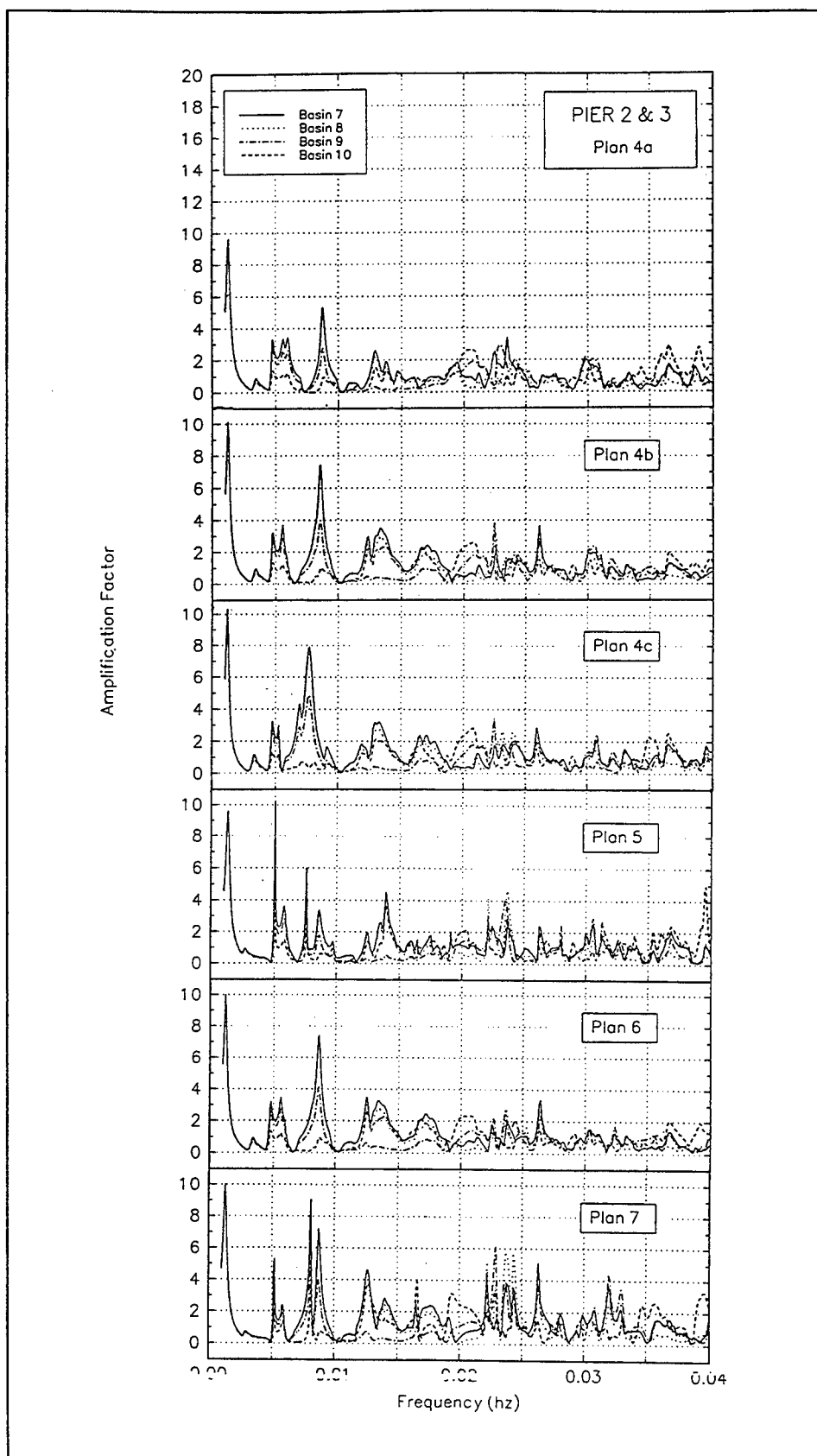
Figure G2. (Concluded)
