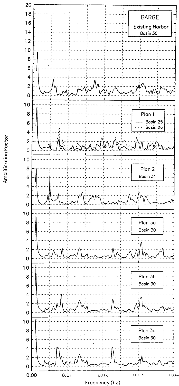
Figure G3. Long wave response, barge pier (Continued)
