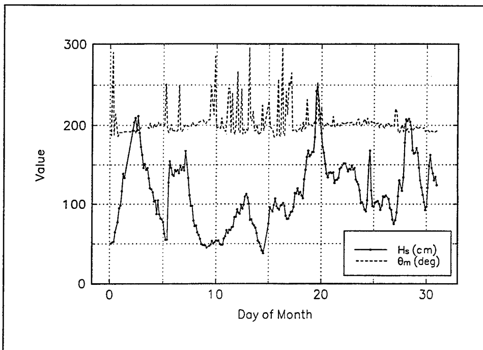
Figure 15. Time-history of H_s and \theta_m (deg, going toward); array, Jan 94
