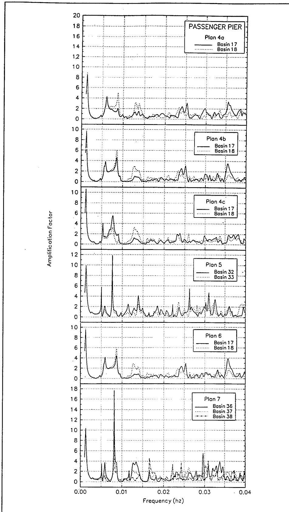
Figure G4. (Concluded)
