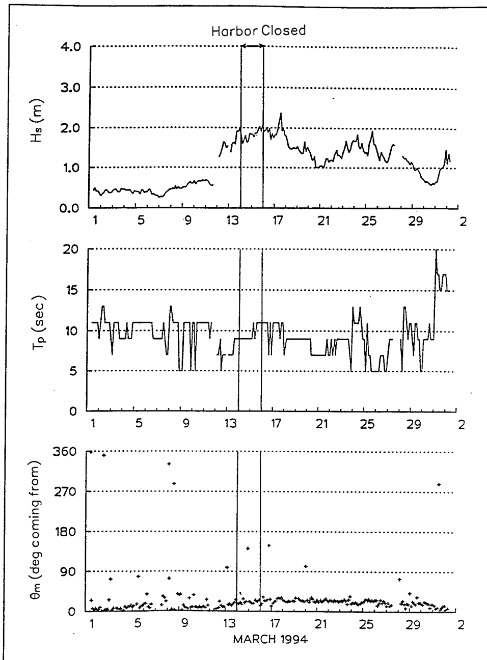
Figure 26. Harbor closing event; array parameters
