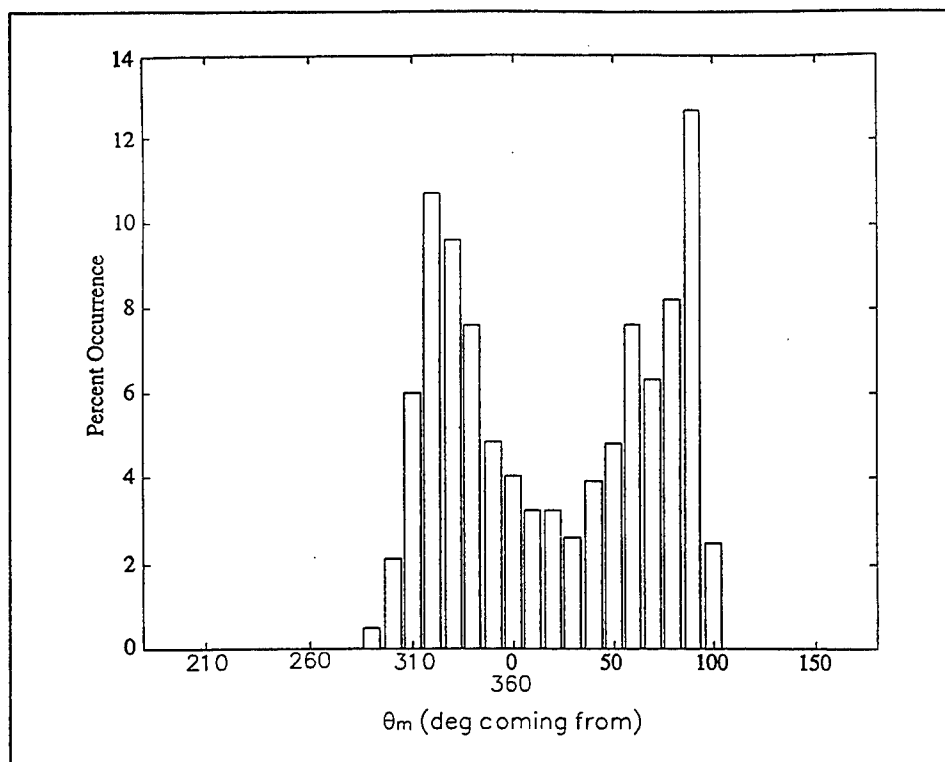
Figure 24. Probability distribution of (\theta_m)_{\text{buoy}} , from NDBC buoy 51026, N. Molokai, Oct 93-Mar 95 (from Merrifield and Okihiro (1996))
