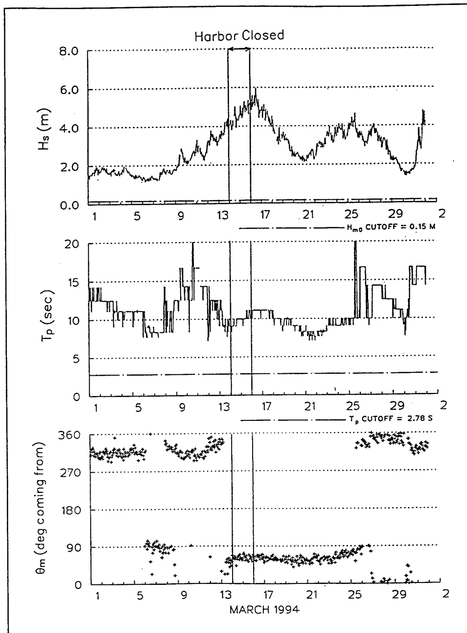
Figure 27. Harbor closing event; NDBC buoy wave parameters
