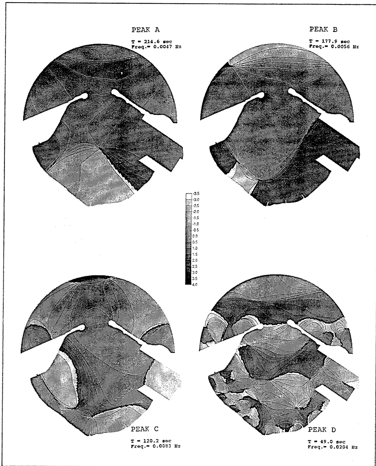
Figure 55. Resonant long wave phase contours, existing harbor
