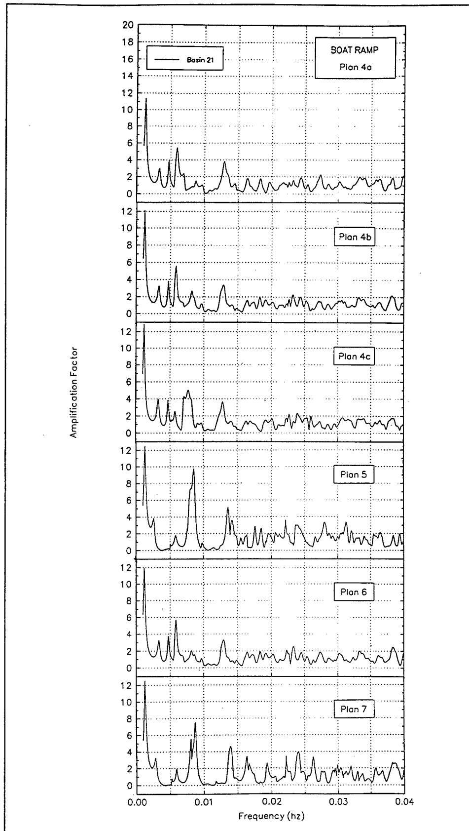
Figure G5. (Concluded)
