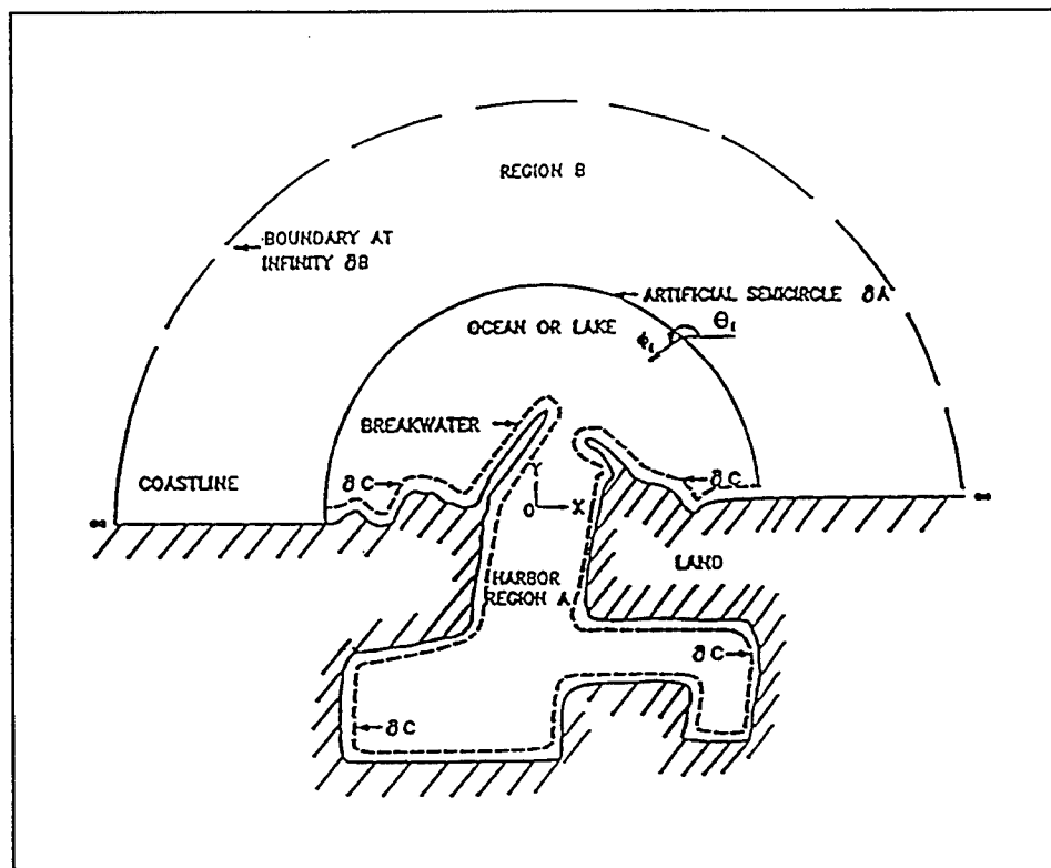
Figure 37. Representation of HARBD domain
