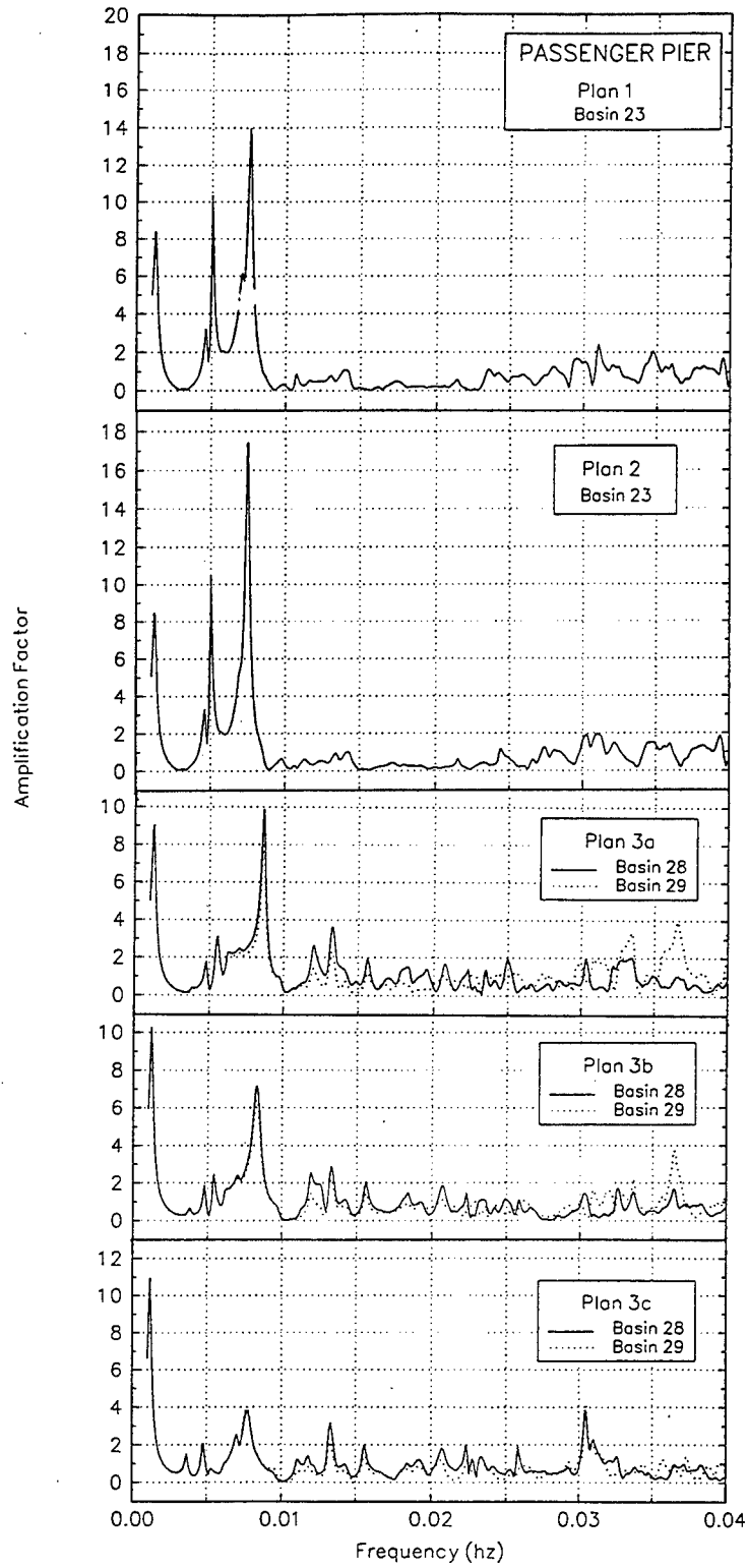
Figure G4. Long wave response, passenger pier (Continued)
