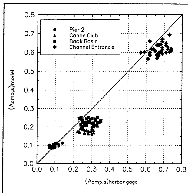
Figure 42. Model short wave validation to 11 months of gage data
