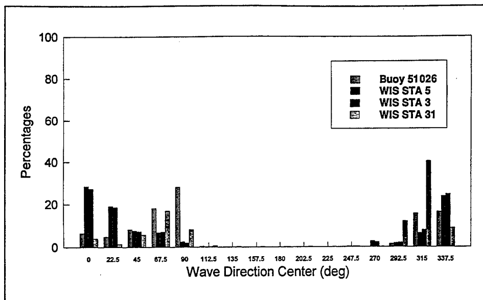
Figure 33. Deepwater wave climate comparison, \theta_m (deg, coming from)
