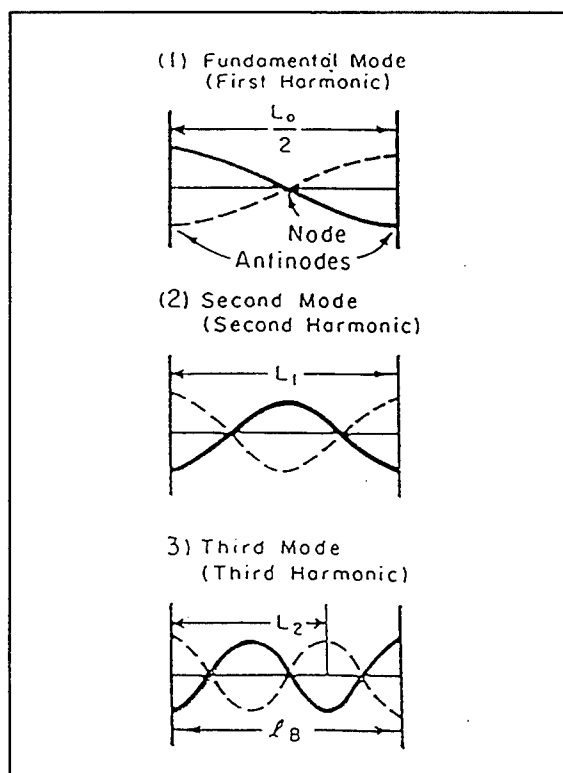
Figure 52. Harbor oscillation definitions
