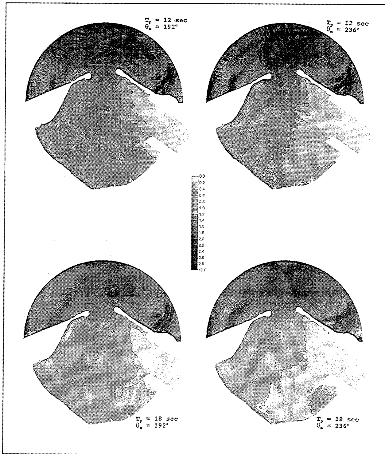
Figure 48. Example swell amplification factor contours, existing harbor
