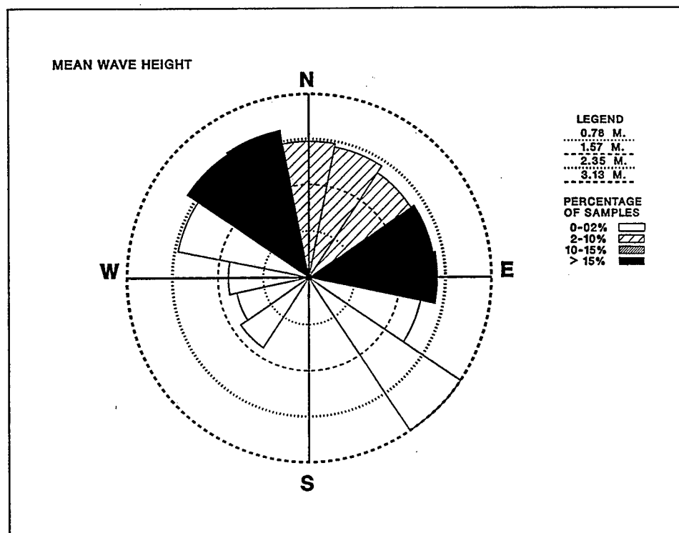
Figure 11. Wave rose, NDBC buoy 51026, N. Molokai
