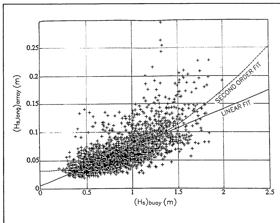
Figure 25. Scatter plot of (H_{s, \text{long}})_{\text{array}} versus (H_s)_{\text{buoy}} (from Merrifield and Okihiro 1996)
