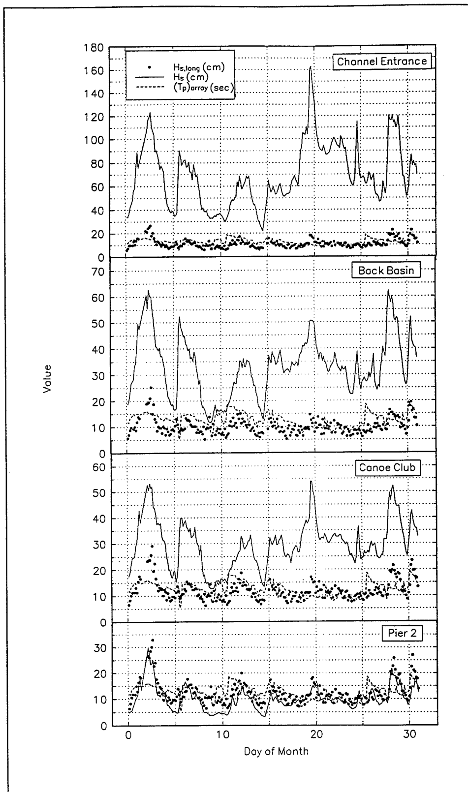
Figure 16. Time-history of H_{s, long} , H_s , and (T_p)_{array} ; harbor gages, Jan 94
