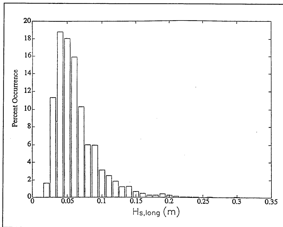
Figure 23. Probability distribution of (H_{s,long})_{array} , Oct 93-Mar 95 (from Merrifield and Okihiro (1996))
