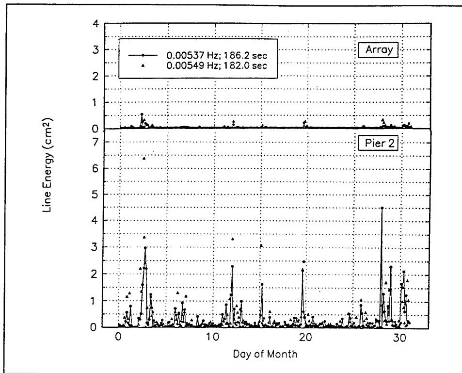
Figure 22. Time-history of amplification of specific resonant peak frequencies, Jan 94
