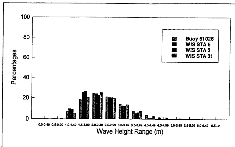
Figure 31. Deepwater wave climate comparison, H_s
