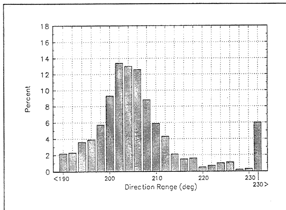
Figure 19. Probability distribution of (\theta_m)_{array} ; Nov 93-Sep 94, 1,785 observations
