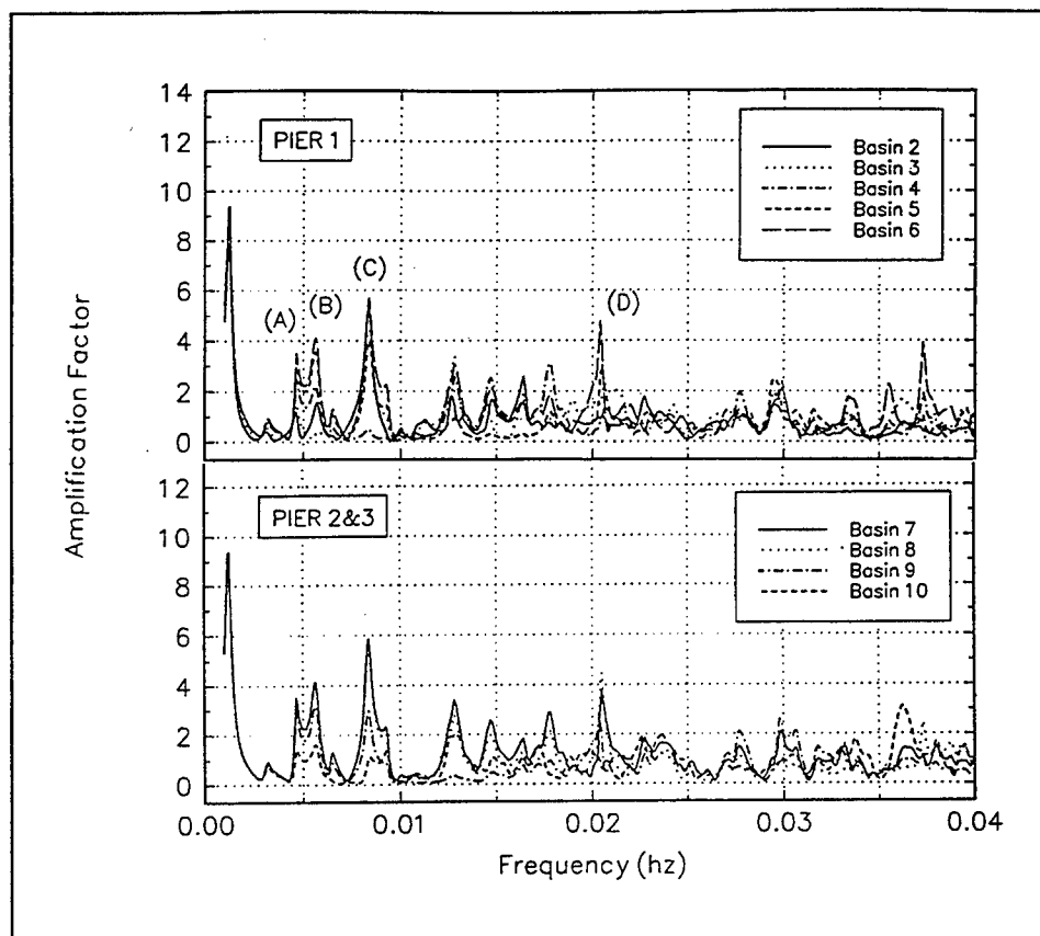
Figure 53. Long wave response, existing harbor, Piers 1-3
