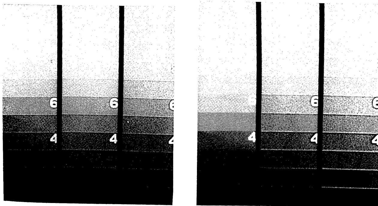
Figure 5: Radiographs of stepwedge. A: RT factors S, T, and F. This demonstrates that the RT factor affects the filtering only in the lower optical density region of the image. (Fuji algorithm settings: G0.8N\#0.6+0.0R5S,T AND F5.0^\circ . Compare this to B with RT factors of T and with RE of 0, 5, and 9. This demonstrates that the T settings affects all optical density regions.
