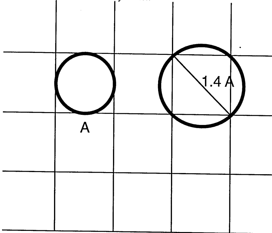
Figure 1: A sphere within a pixel has the same diameter as the pixel, but fills only 50% a cubic voxel of the same size. To fill a pixel of size A, need a sphere, if centered on pixel of size A, by Pythagorean Theorem: A\sqrt{2} .
