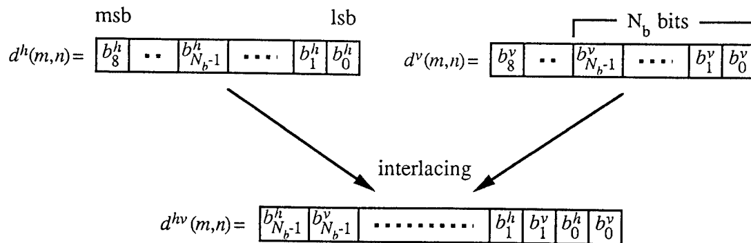
Figure 2: Interlacing the bit fields of d^h(m, n) and d^v(m, n) to form a new number d^{hv}(m, n)
