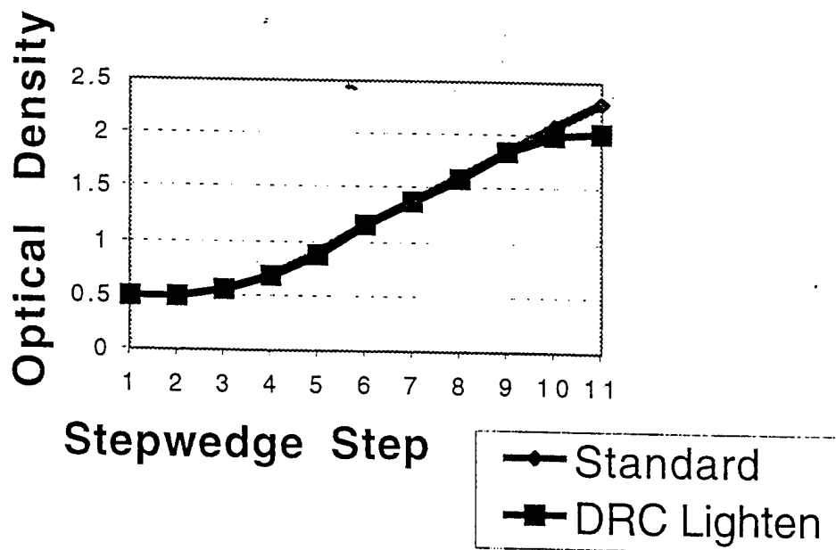
2C: DRC effect of decreasing the high optical density regions of the image.
