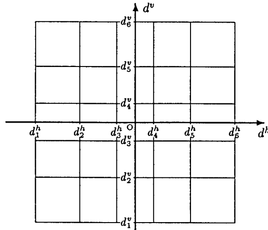
Figure 1: Partitioning the d^h - d^v plane with each region defining an initial context.
