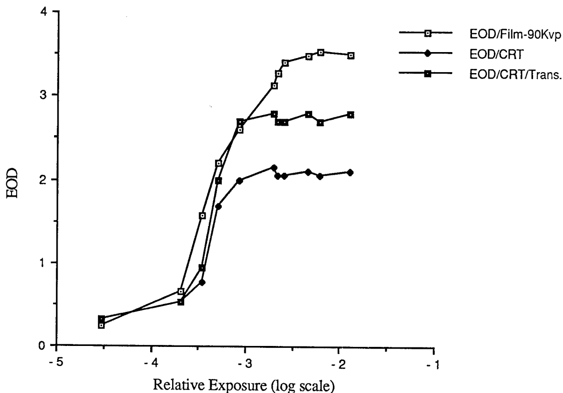
Figure 3. H&D Curves on Film, CRT, and Transfomed Gray Tone on CRT
