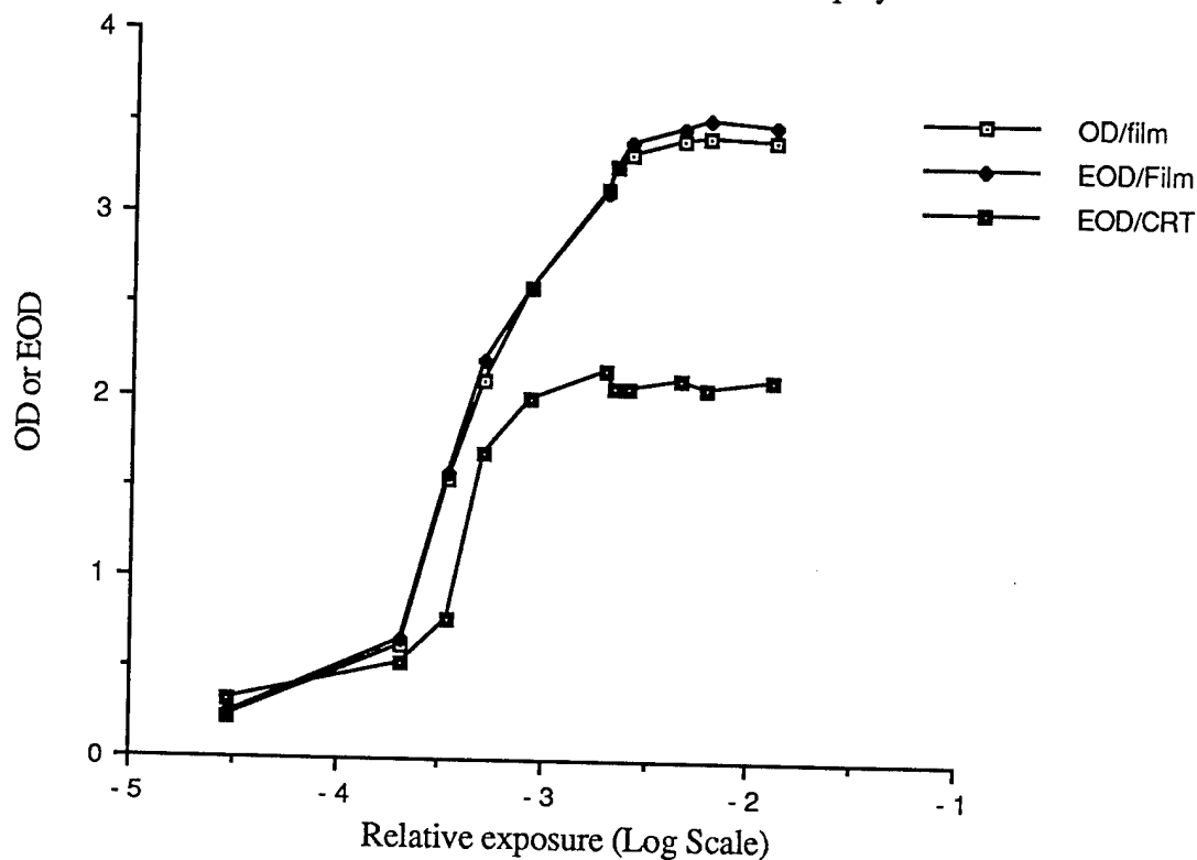
Figure 1. H&D Curves of Film and CRT Display
