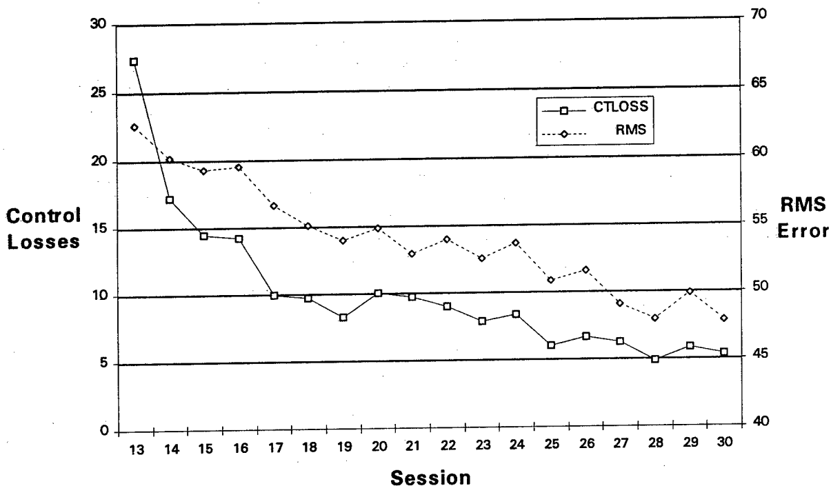
Figure 8. Dual Tracking-Individual Lambda (Control Losses and RMS Error).
