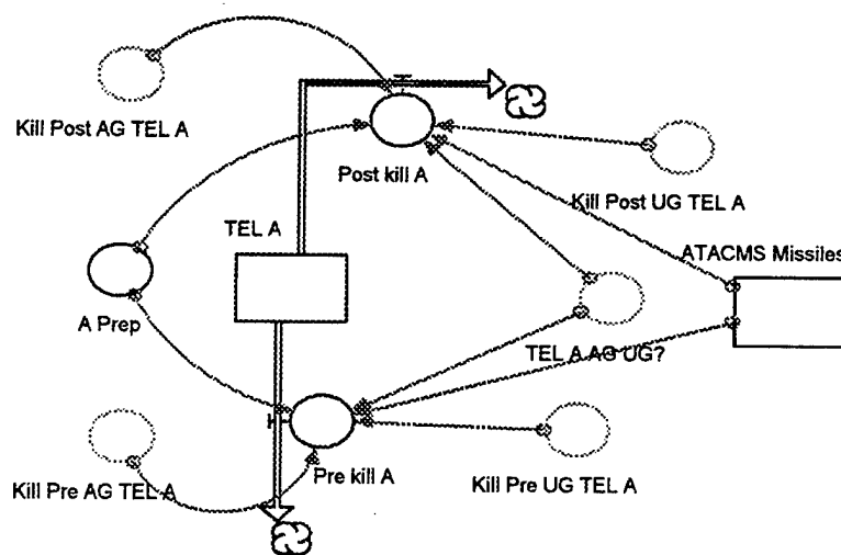
Figure 4-2. Attack Operations
