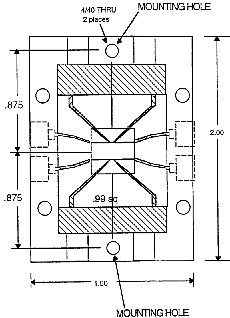
FIGURE B-4. Chip Holder Circuit and HTS Chip Mounted in Housing.
