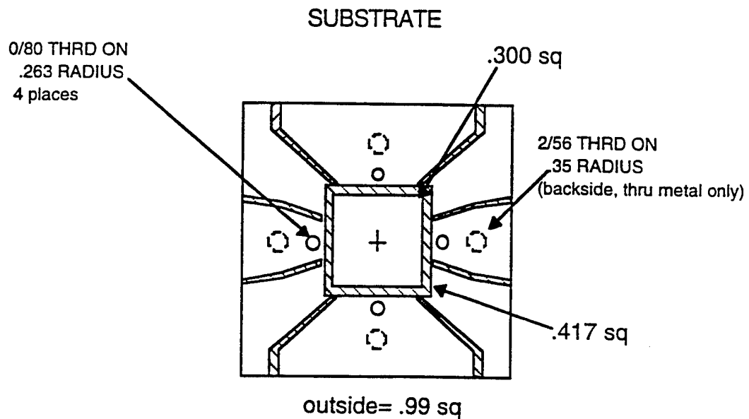
FIGURE B-3. Chip Interface Circuit (Roger's 6010LM on 0.125 Inch Aluminum).
