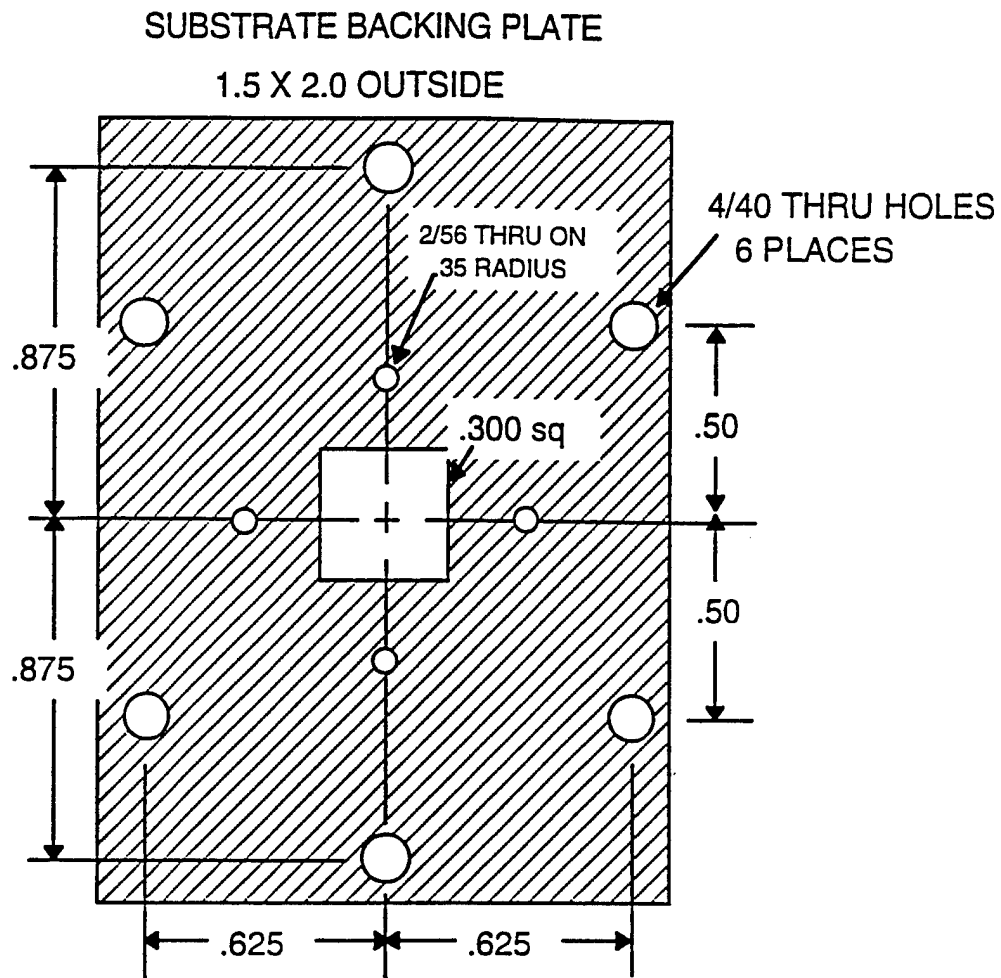
FIGURE B-2. Back Circuit Mounting Plate.
