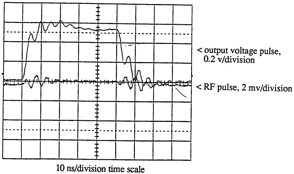
FIGURE F-11. Detected RF Pulse Out of 2-Millimeter Switch #1. 5.0 volt, 50 ns wide, 100 ns period.
