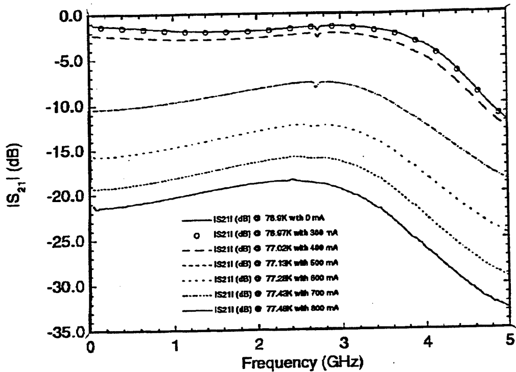
FIGURE E-2. Switch Circuit. S_{21} versus laser power supply current, 2-Millimeter circuit at 77 K.
