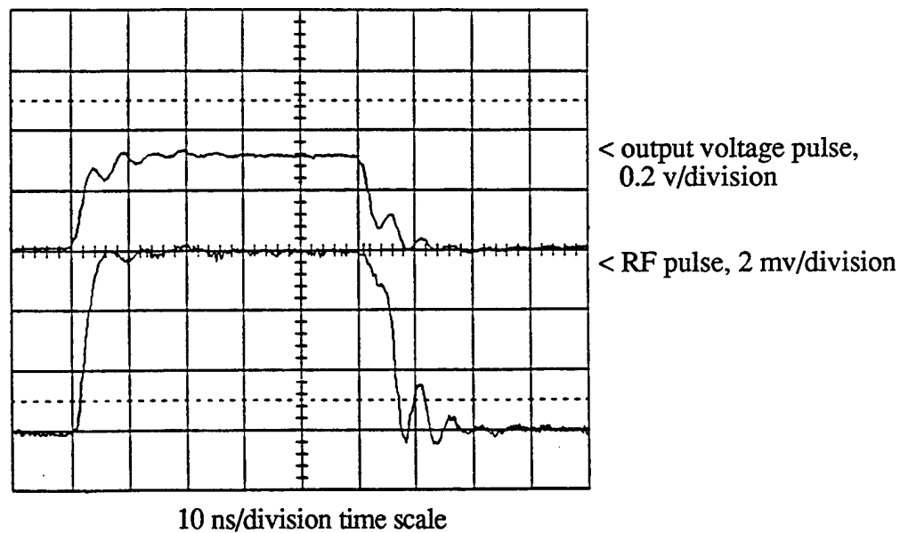
FIGURE F-7. Detected RF Pulse Out of 2- Millimeter Switch #1. 1.0 volt, 50 ns wide, 100 ns period.
