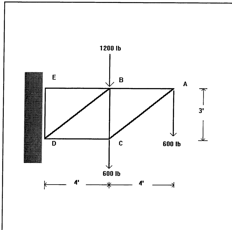
Figure C5. Complex truss
