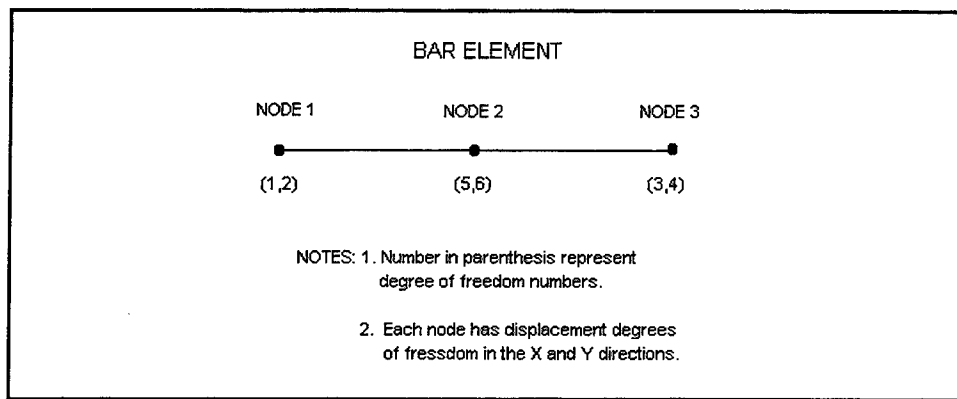
Figure 6. Bar element
