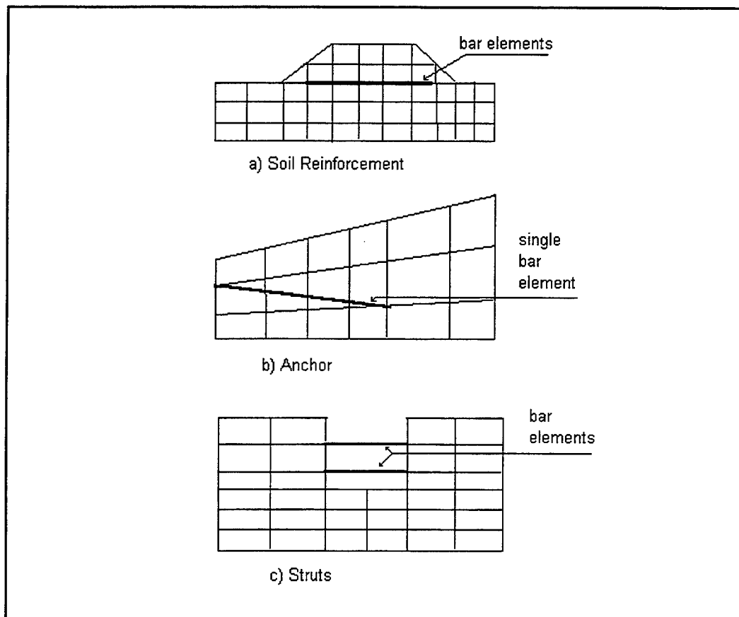
Figure 8. Bar applications
