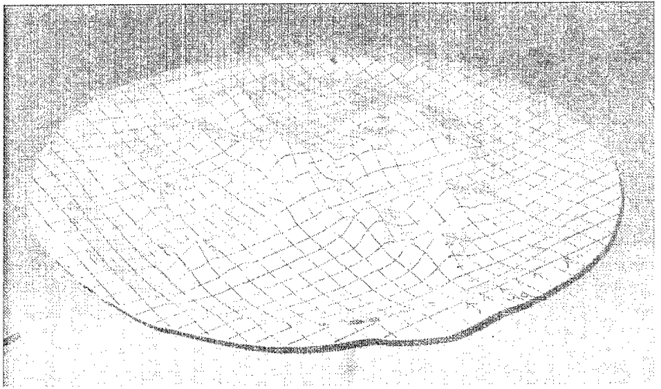
Figure 2. Condition of the reinforced PVC after a sustained load of 150 psi (1 MPa) for 24 hr
