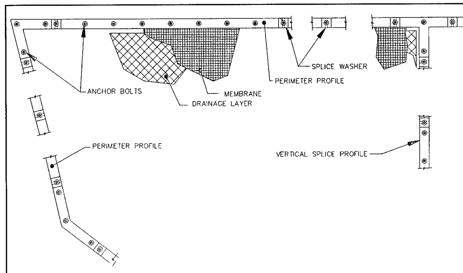
Figure 5. Assembly detail A from general scheme (Figure 4)
