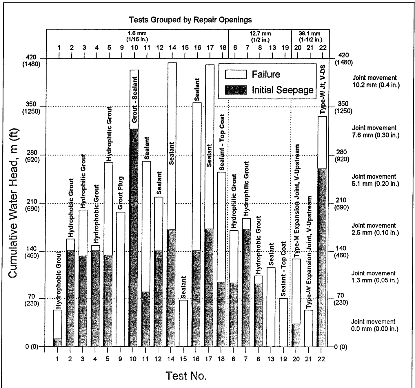
Figure 3. Cumulative sum of water heads for joint movements at times of initial seepage and failure of the repair (Tables 1 and 2 for repair details)
