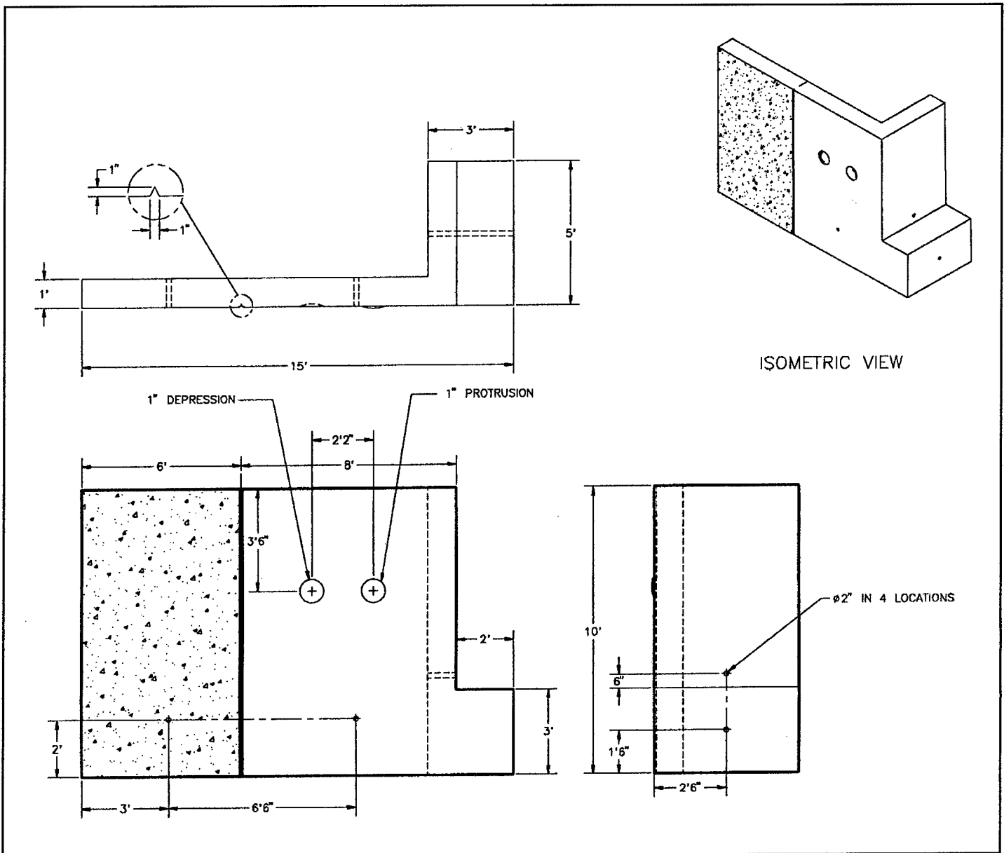
Figure 6. Test structure for constructibility demonstration
