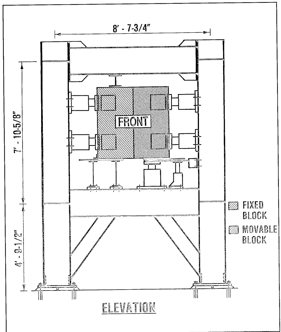
Figure 2. Simulated joint movement system (secondary waterstop test apparatus)
