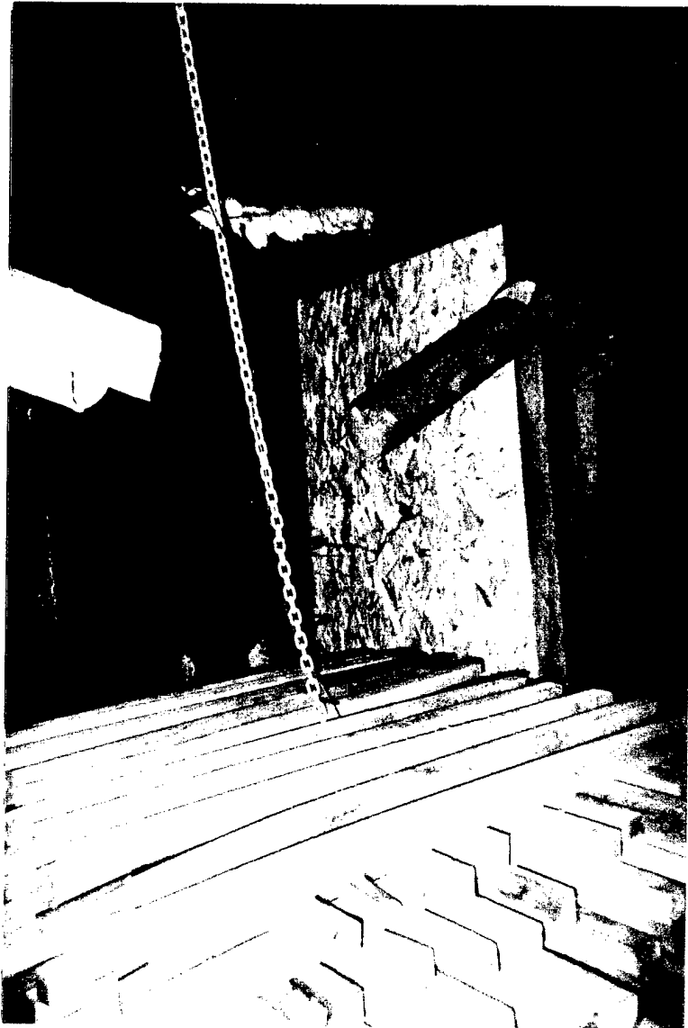
Fig. 8 – Fire source No. 2 (viewed from WTD 2-21-2)
