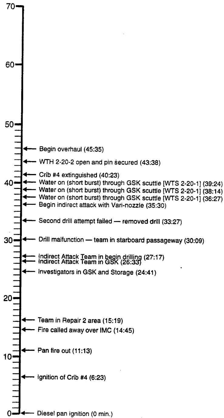
Fig. C3 — Timeline of events for Test SCBA-05
