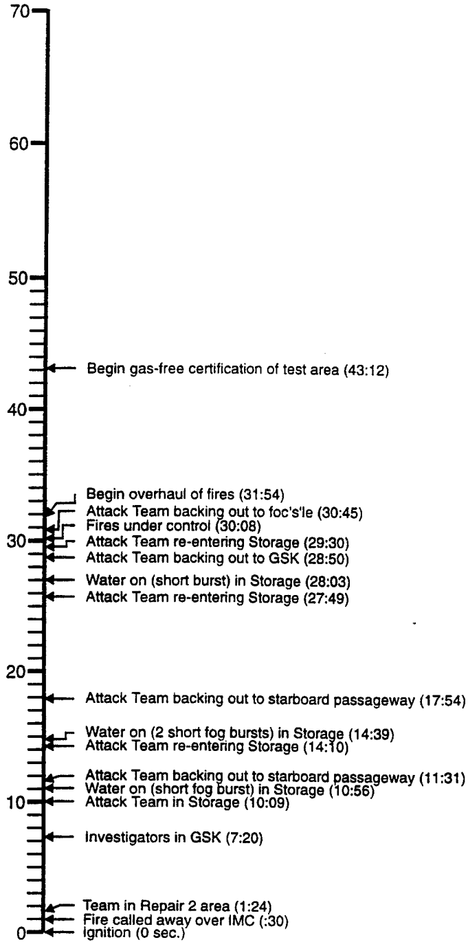
Fig. C1 — Timeline of events for Test SCBA-03
