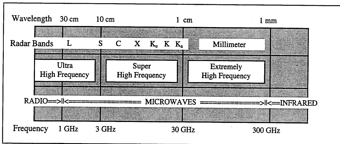
Figure 1: The Electromagnetic Frequency Spectrum
