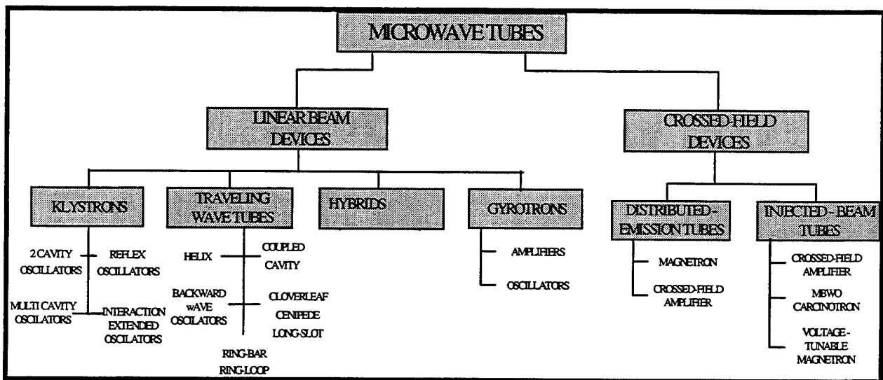
Figure 3: The Microwave Tube Family
