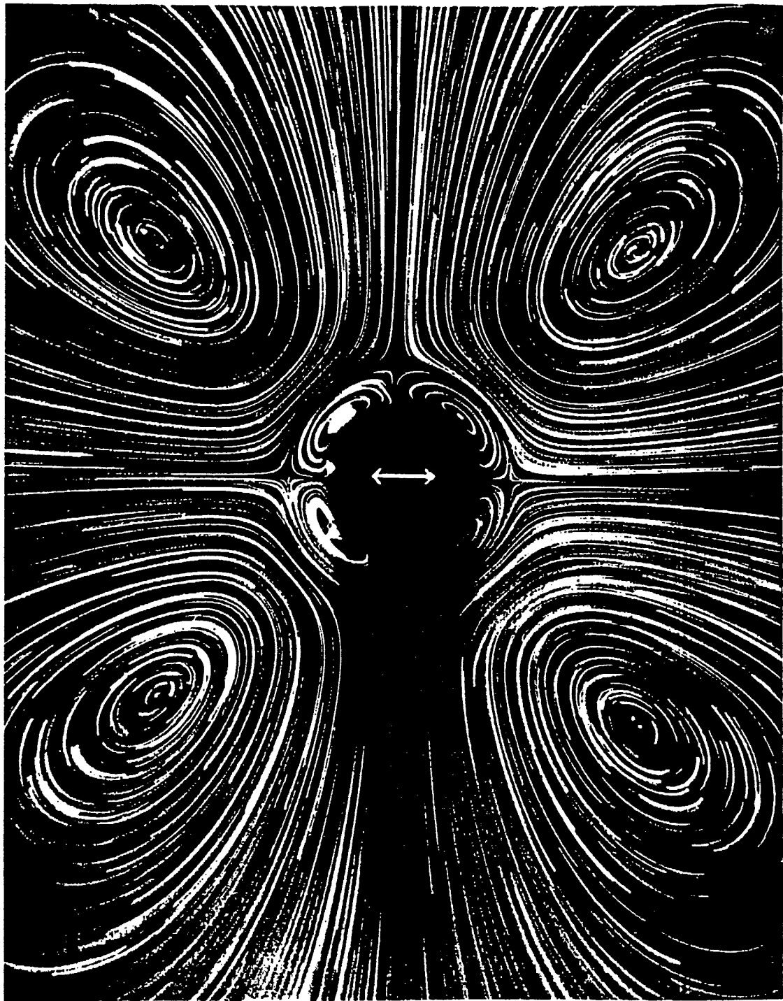
31. Secondary streaming induced by an oscillating cylinder. A long circular cylinder is oscillated normal to its axis by a loudspeaker in a mixture of water and glycerine. Suspended glass beads are illuminated in a cross plane by a stroboscope. The amplitude of oscillation is 0.17 of the
