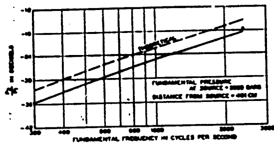
FIG. 4. Variation of 2nd harmonic magnitude with frequency of fundamental.
