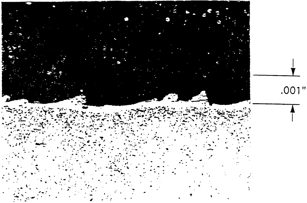
Figure 7a. Wire EDM recast layer - single-pass (magnification 500X)
