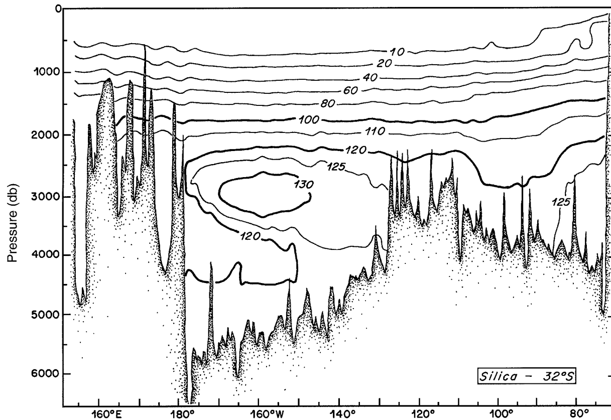
Figure II-38: A simplified section summarizing the silica distribution across 32°S, adapted from Toole et al. (1994b).
