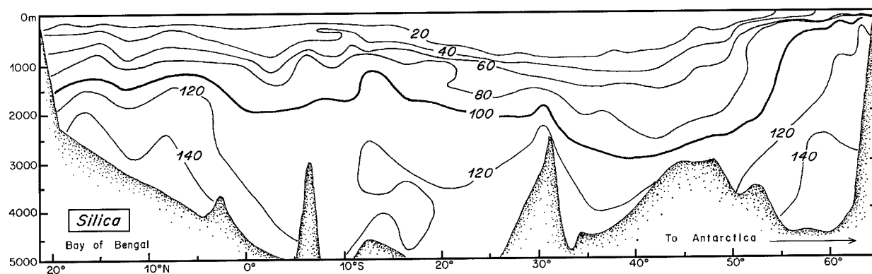
Figure II-84: A silica section from the Bay of Bengal to Antarctica, adapted from p. 414 in the Indian Ocean Atlas (Wyrtki, 1971).
