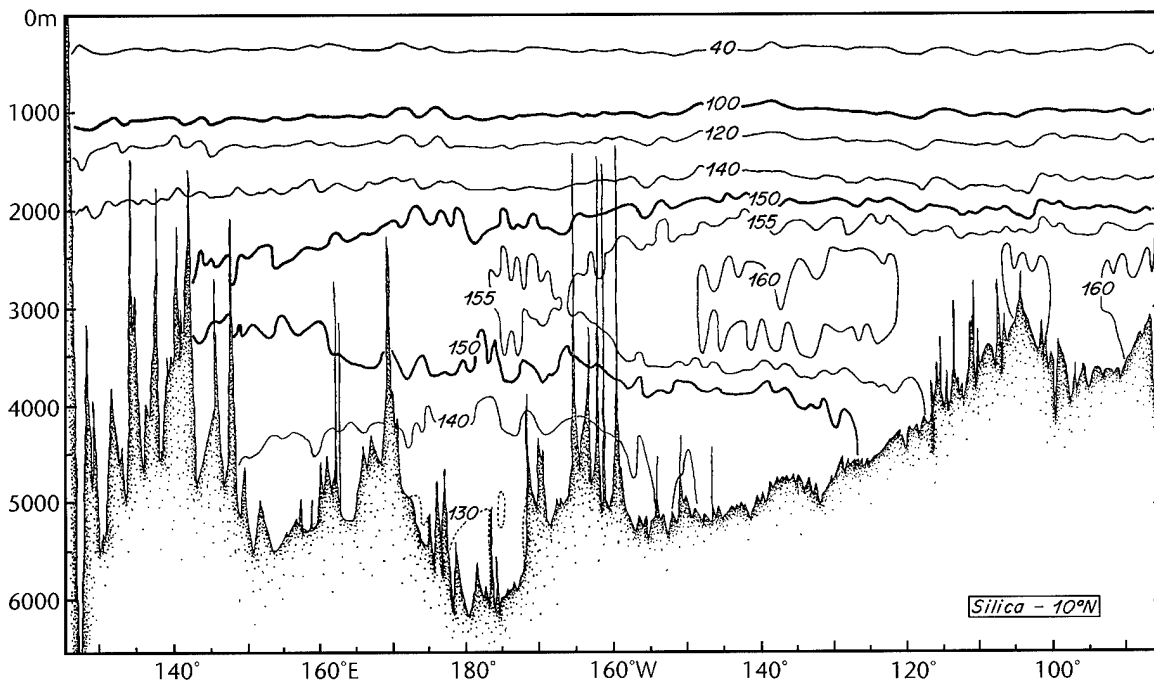
Figure II-34: A summary section for silica at 10°N in the Pacific Ocean, adapted from Wijffels et al. (1996).
