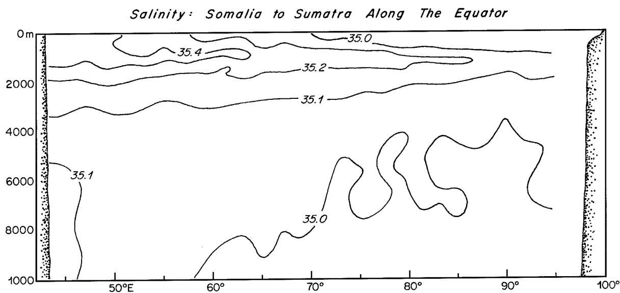
Figure II-116: A salinity section along the equator in the Indian Ocean from Somalia to Sumatra, adapted from Wyrтки (1971, p. 515).
