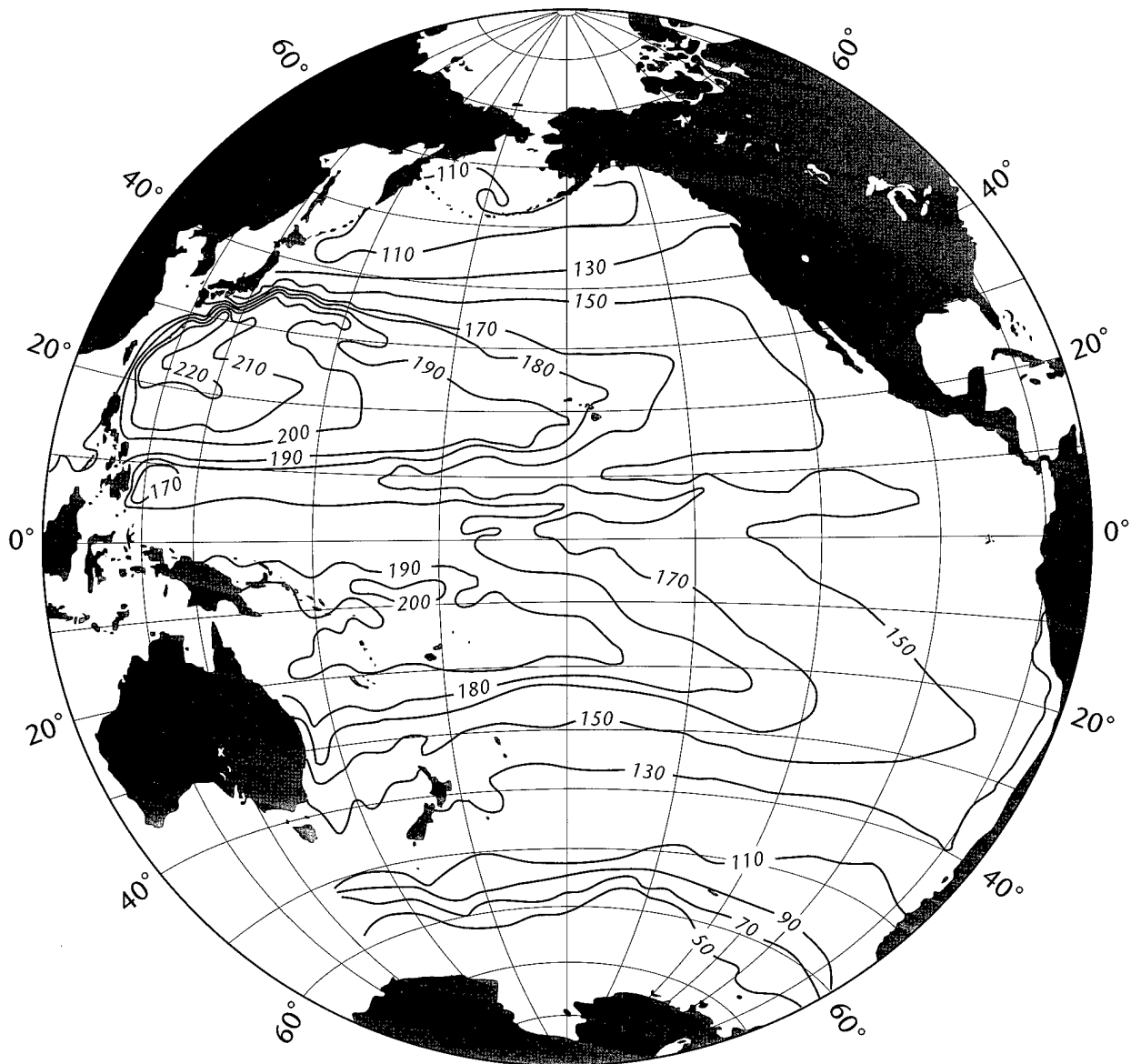
Figure II-24: Selected dynamic height (0/1000 m) contours (in dynamic centimeters) for the Pacific Ocean, adapted from Wyrtki (1974).
