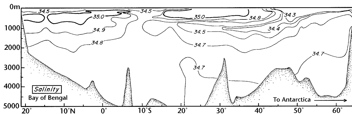
Figure II-16: A salinity section from the Bay of Bengal to Antarctica, adapted from p. 412 in the Indian Ocean Atlas (Wyrski, 1971).
