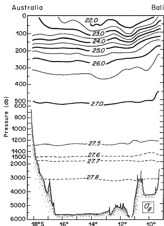
Figure II-91: Potential density parameter ( \sigma_\theta , \text{kg m}^{-3} ) section, Australia to Bali, station locations in Figure II-88, selected contours from Fieux et al. (1994).
