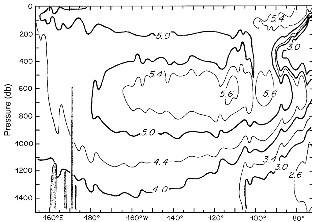
Figure II-54: Contours of \text{O}_2 for the upper 1500 db of a section across 32^\circ\text{S} , adapted with smoothing and simplification from Toole et al. (1994b).
