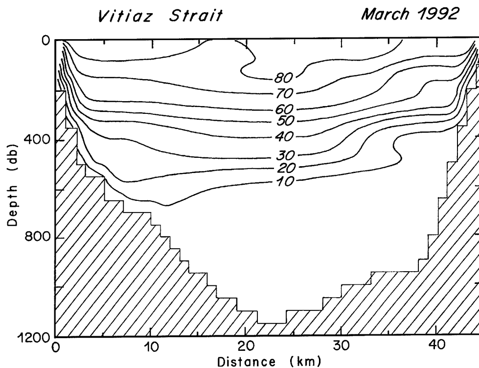
Figure II-58: Monthly averaged along- channel speeds (cm s -1 ) in Vitiaz Strait, March 1992, taken from Murray et al. (1995).
