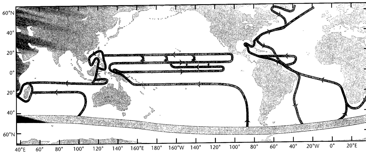
Figure II-10: An adaptation of the equivalent two-layer schematic of the upper (red) and lower (blue) layer interbasin-scale circulations as modeled by Shriver and Hurlburt (1996, their figure 7). The lower blue layer in this figure is model layer 6, and the upper layer the sum over model layers 1–5. The green line at the bottom of the figure denotes a region of wind-driven upwelling in the ACCS.
