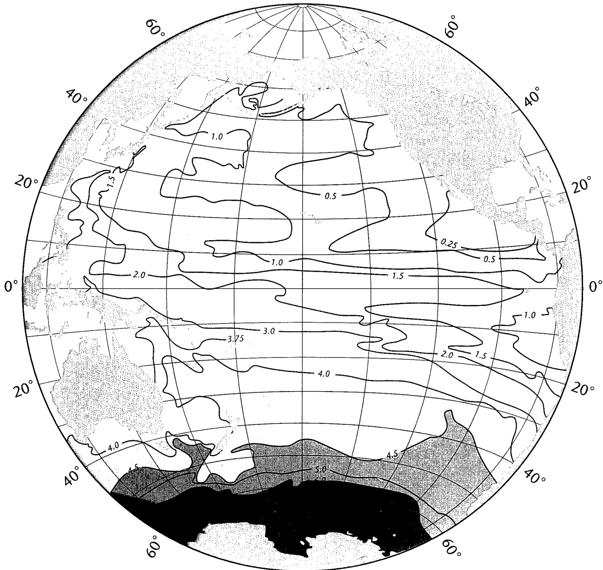
Figure II-63: Oxygen contours (ml L -1 ) on the \sigma_t horizon 27.3 (approximately), adapted from Reid (1965, his figure 25).
