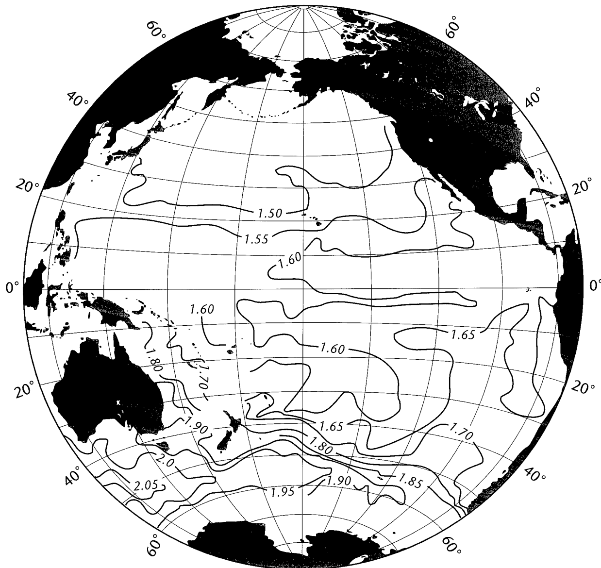
Figure II-66: Potential temperature ( ^{\circ}\text{C} ) on \sigma_2 = 36.96 (2500 m depth nominal) for the Pacific Ocean, adapted from Talley and Johnson (1994) and Talley (1995).
