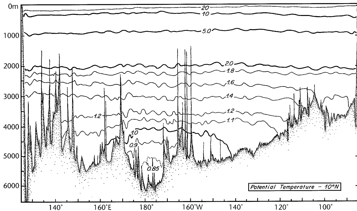
Figure II-33: A potential temperature (°C) summary section at 10°N in the Pacific Ocean, adapted from Wijffels et al. (1996).
