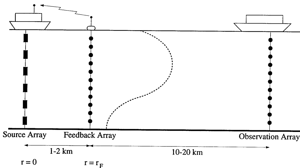
Figure 1-1: Proposed Experimental Setup
