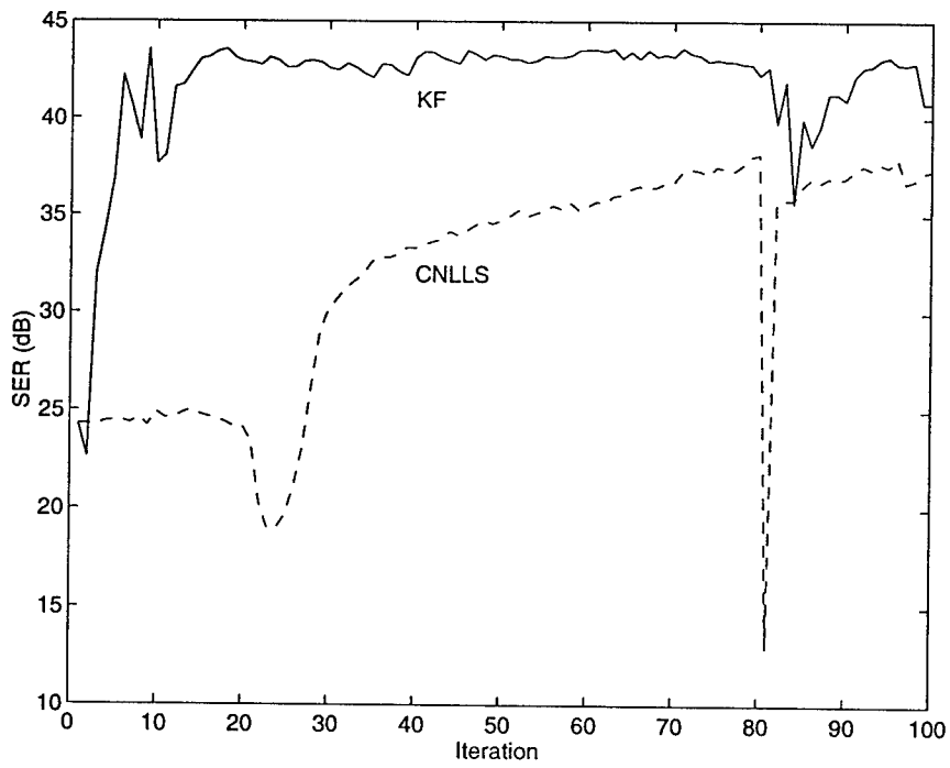
Figure 4-8: SER Performance for Mode 1 + 0.4j Mode 2 in Time-Invariant Waveguide
