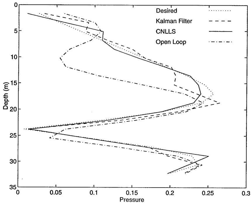
Figure 3-14: Vertical Profile of Pressure for a Typical Trial in Rock Outcropping Environment
