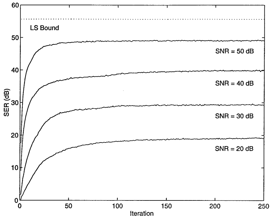
Figure 3-5: SER for CNLLS Estimator at different SNR levels
