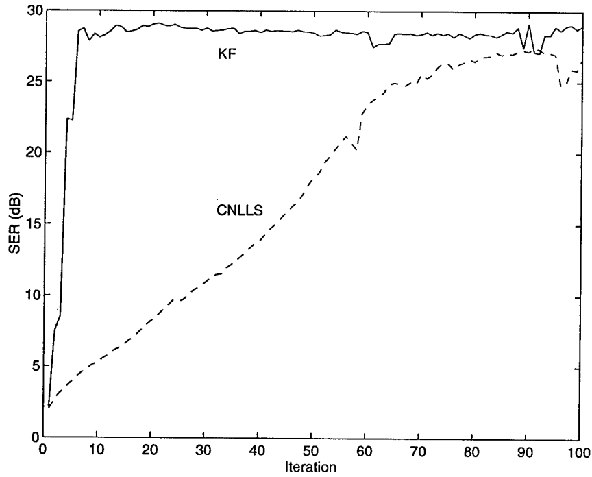
Figure 4-7: SER Performance for System Mode 4 in Time-Invariant Waveguide
