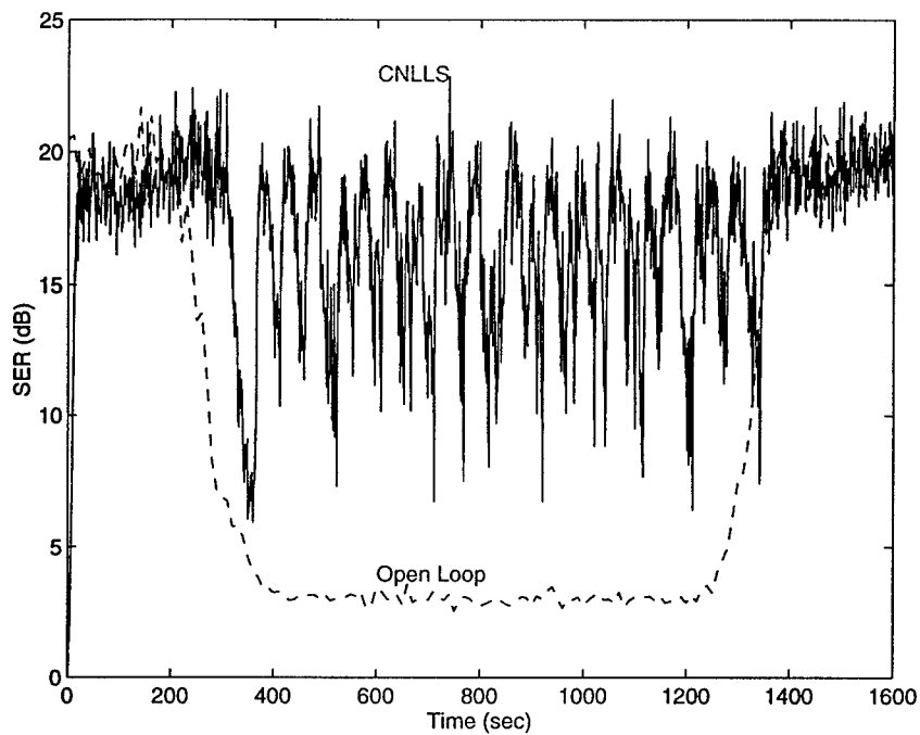
Figure 3-21: Performance of feedback control algorithm using CNLLS estimator compared with open loop controller for solitary wave propagating through feedback volume.
