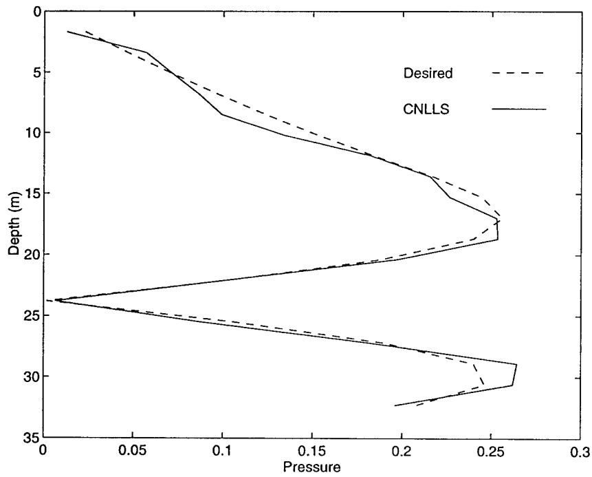
Figure 3-6: Vertical Profile of Pressure for Typical Trial of CNLLS Estimator
