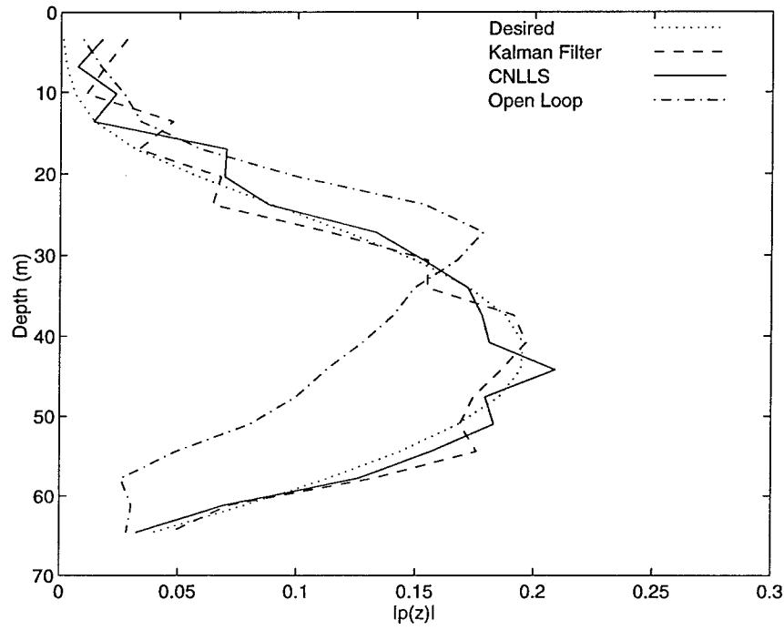
Figure 3-19: Typical Vertical Pressure Profiles for Downsloping Wedge Environment
