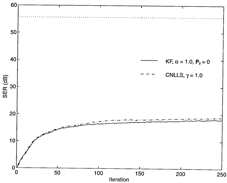
Figure 3-11: Comparison of CNLLS and Kalman filter estimators
