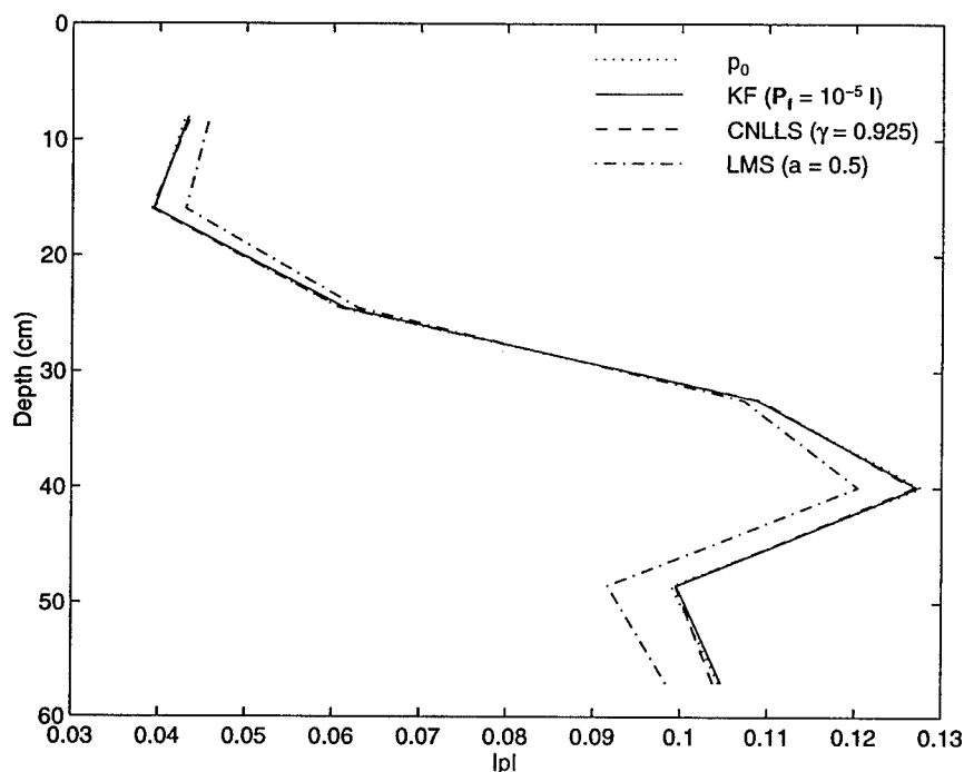
Figure 4-12: Depth Profile of Pressure Magnitude for All Channel Estimators after 100 Iterations
