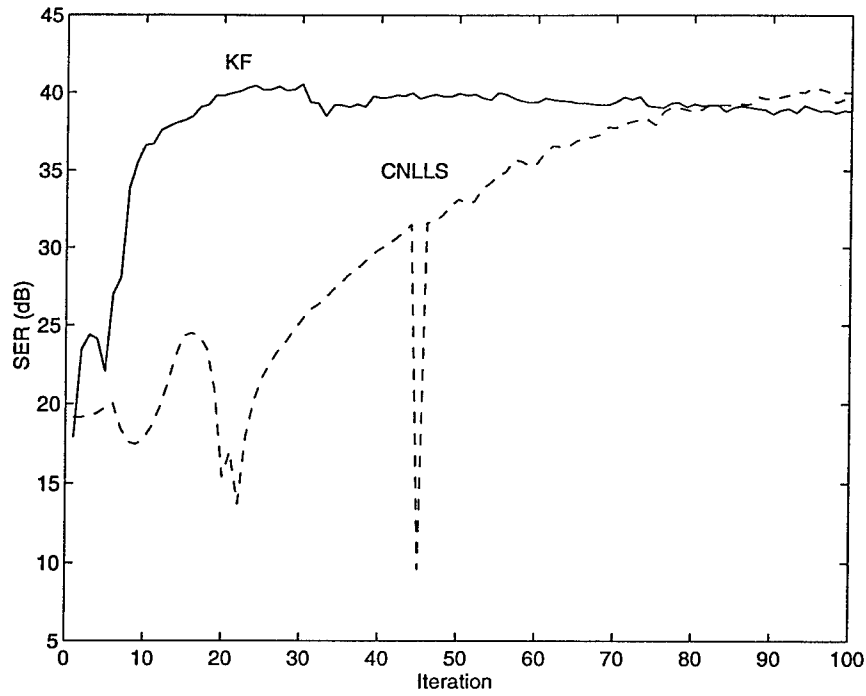
Figure 4-5: SER Performance for System Mode 2 in Time-Invariant Waveguide
