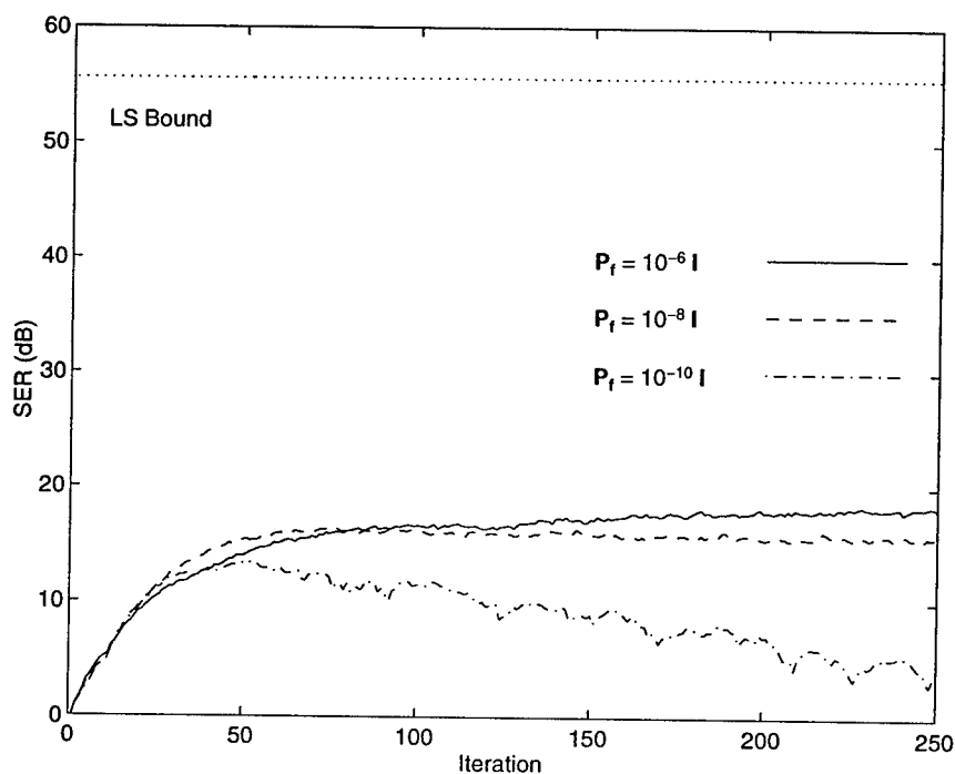
Figure 3-7: Ratio of Energy in Desired Profile to Energy in Mean Error for Kalman Filter Estimator with \alpha = 0.98
