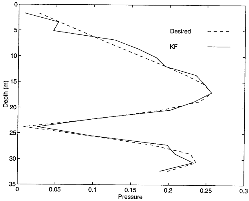
Figure 3-10: Vertical Profile of Pressure for Typical Trial of Kalman Filter Estimator with \alpha = 0.99 , P_f = 10^{-6}I .
