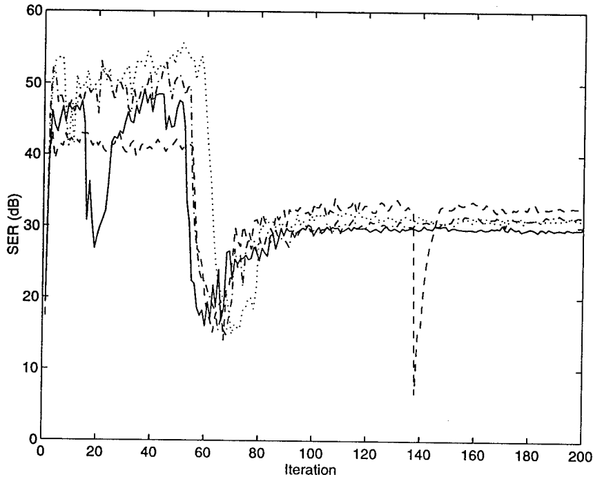
Figure 4-14: Transient Response of Kalman Filter Channel Estimator for Gradual Change in the Waveguide
