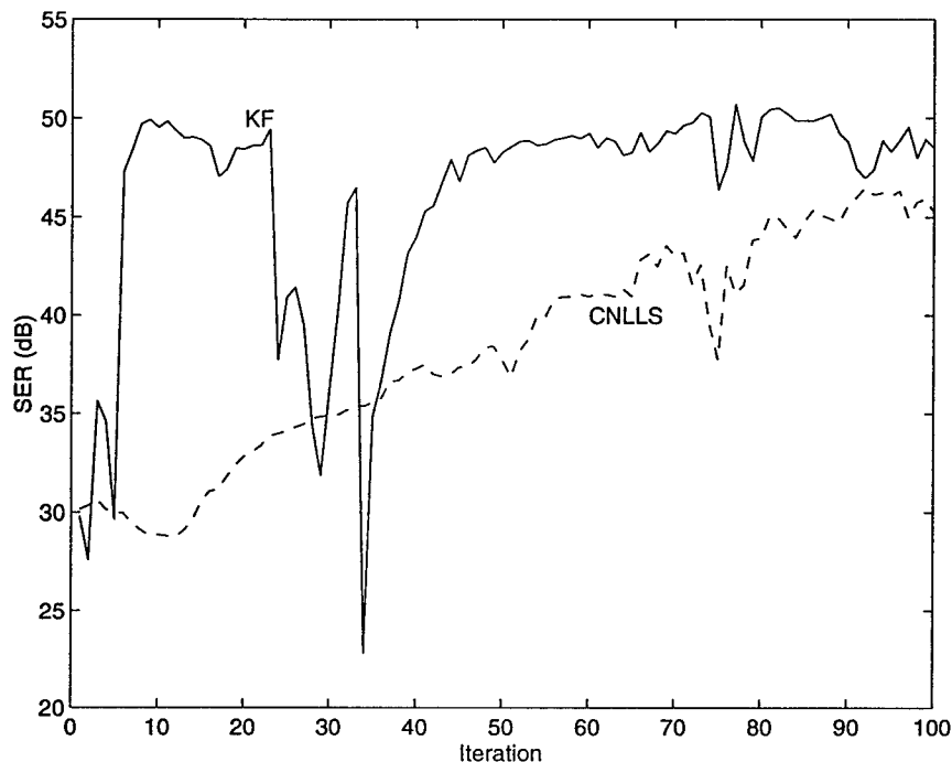
Figure 4-4: SER Performance for System Mode 1 in Time-Invariant Waveguide
