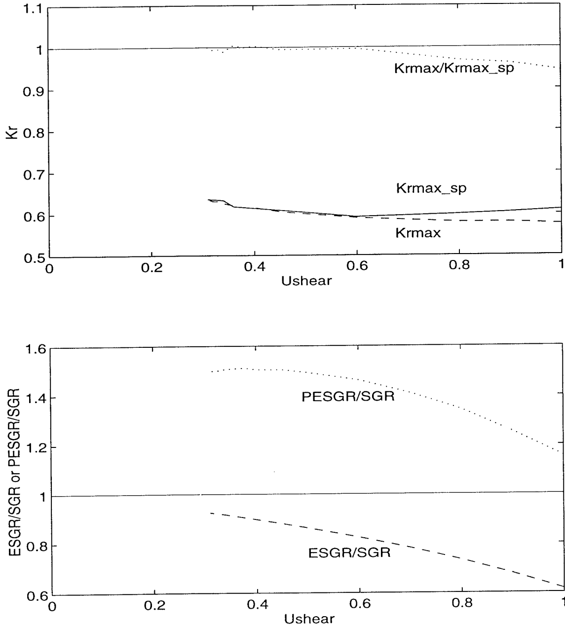
Figure 2.21: Comparison between temporal and spatial instabilities as Ushear varies. U_1 - U_2 = 0.8 and \beta = 0.05 are both fixed. The upper panel shows real parts of wavenumbers corresponding to most temporally and spatially unstable waves and their ratio, and the lower panel ESGR/SGR and PESGR/SGR .
