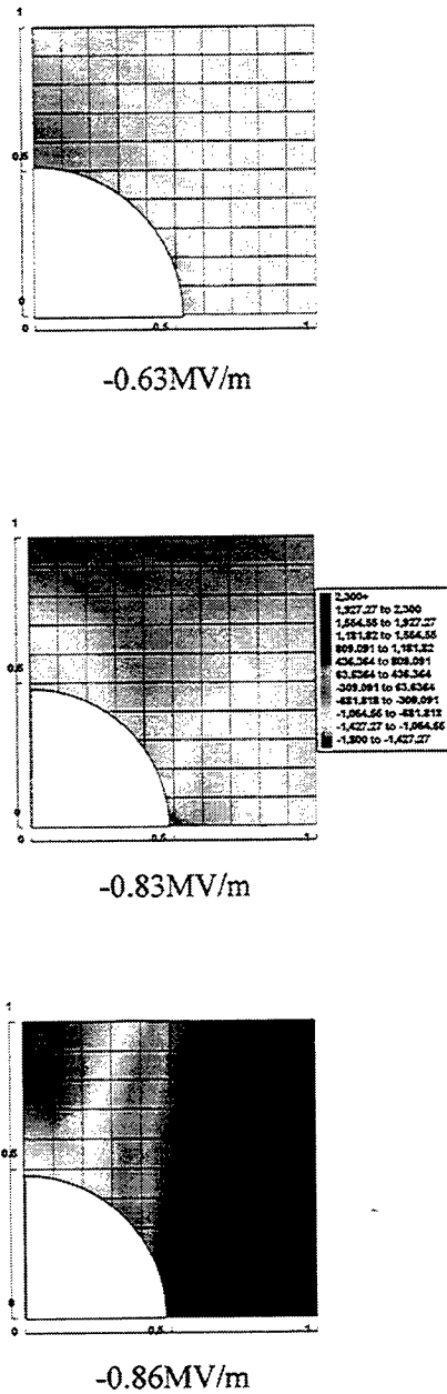
Figure 4. Contour plots of \epsilon_{33} for three different applied electric field values
