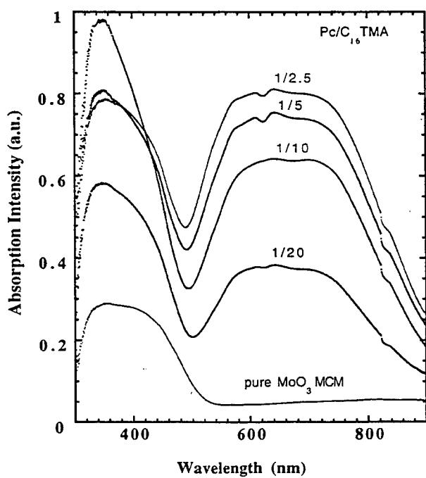
Fig. 6 (b) Optical absorption spectra for Pc-doped \text{MoO}_3 MCM
