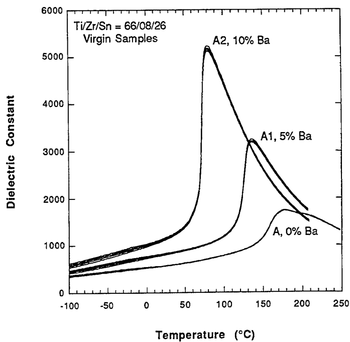
Figure 3: Temperature dependence of dielectric constant for the compositions A, A1, and A2; (cooling) virgin sample.
