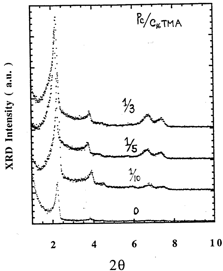
Fig. 7 (a) Low angle XRD spectra for \text{Pc}(\text{Cu}) -doped \text{SiO}_2 MCM
