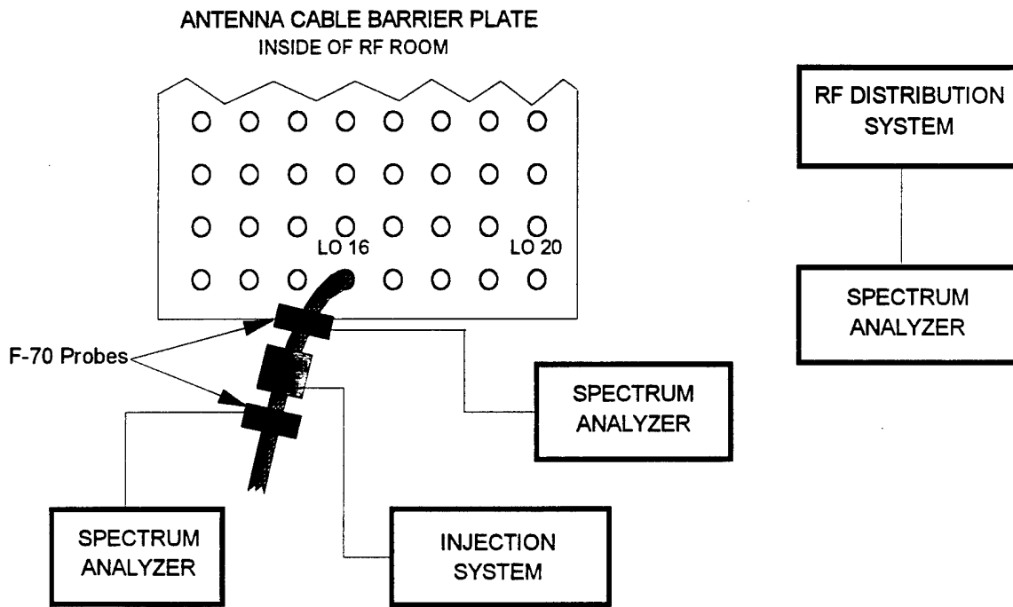
Figure 3.6-1 Block Diagram for Test 4
