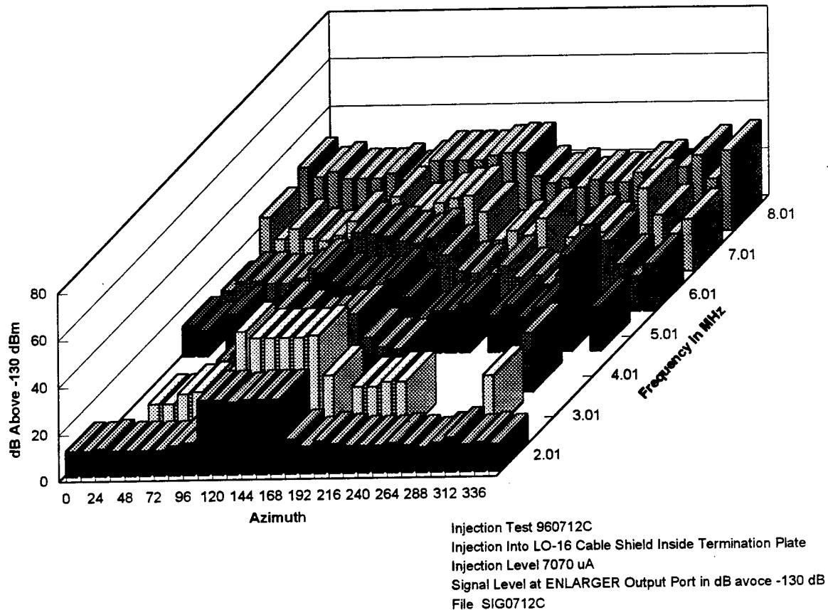
Figure 3.6-2 Low-Band EMI Leakage, Test 4
