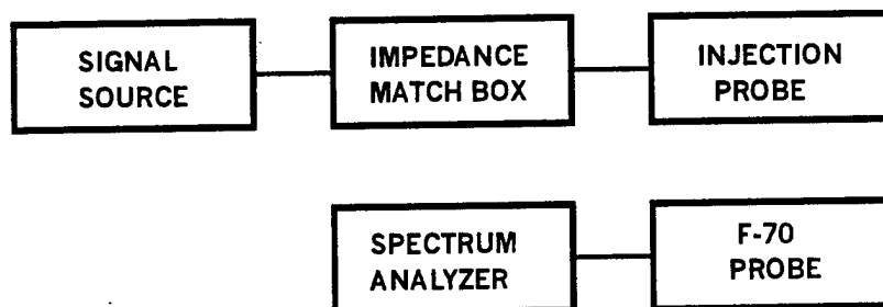
Figure 3.1-1 Injection Instrumentation
