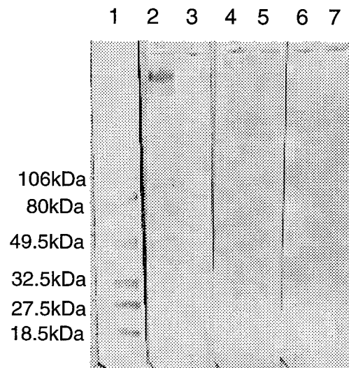
FIGURE 7: Reactivity of LCL-4 culture supernatate (antibody source) in Western blot. Lane 1: Molecular weight standards; lane 2: LCL-4 reacted with Br-2 (breast carcinoma cell line) spent medium; lane 3: LCL-4 reacted with normal fibroblast spent medium; lane 4: RPMI instead of LCL-4 culture medium as no antibody control reacted with Br-2 spent medium; lane 5: RPMI instead of LCL-4 culture medium reacted with fibroblast spent medium; lane 6: alkaline phosphatase conjugated goat anti-human IgM control (conjugate control) with spent medium of Br-2; and lane 7: same as lane 6 but against spent medium of normal fibroblasts.
