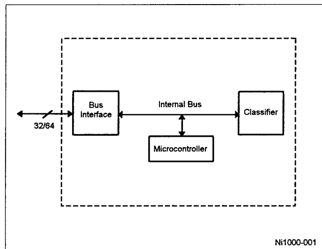
Figure 1-1. Block Diagram
