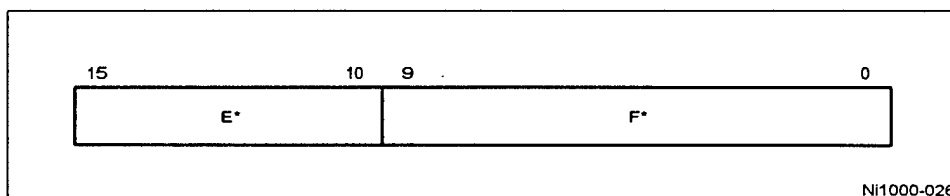
Figure 4-46. Internal 16-Bit Floating-Point Format
