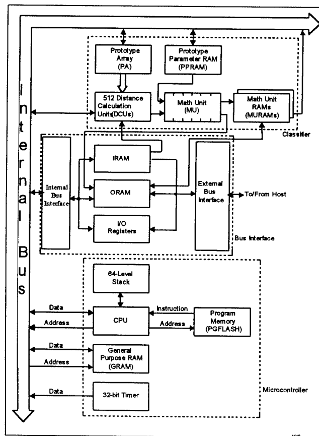
Figure 2-2. Internal Architecture
