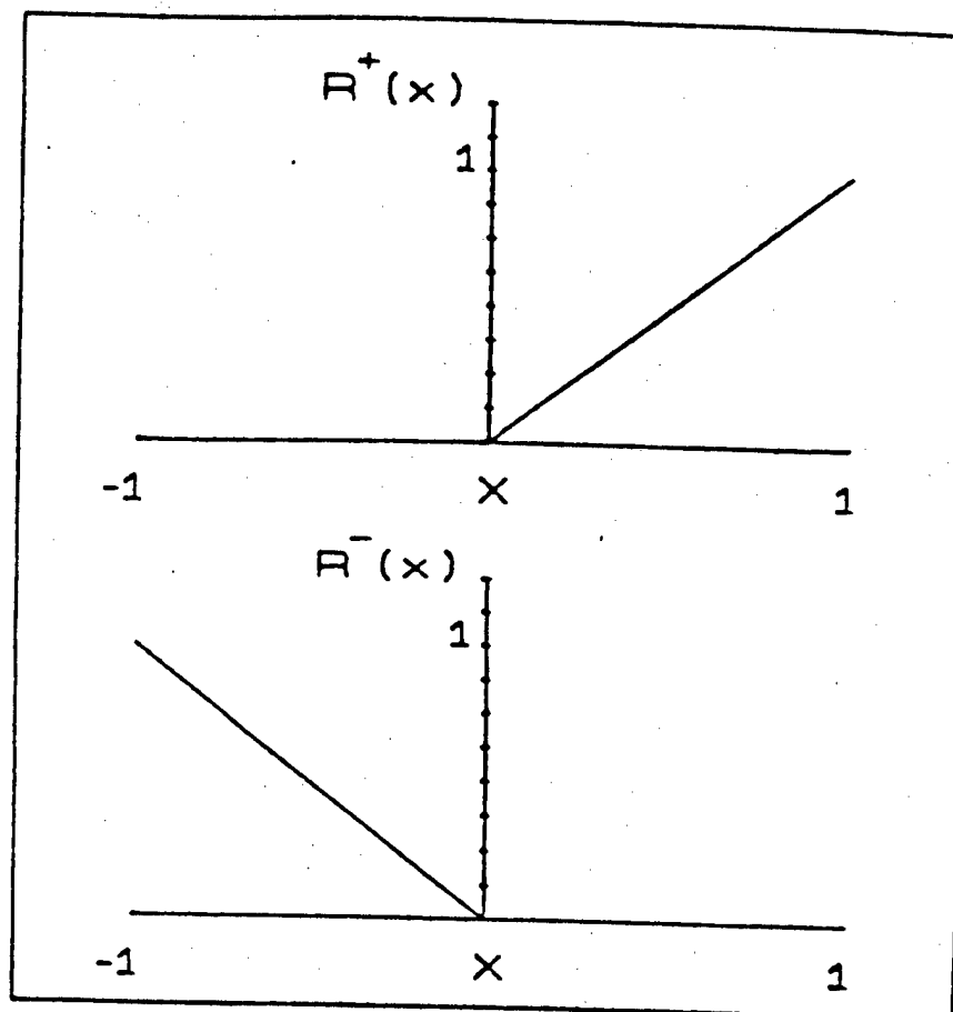
Figure 3.6 Operating characteristics of the half-wave rectifiers [7]
