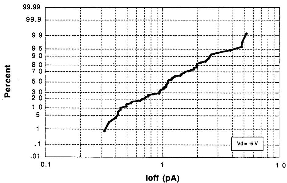
Figure 5-5. Probability distribution for minimum leakage current in W/L = 10\mu\text{m}/4\mu\text{m} transistors at 5-V drain bias.
