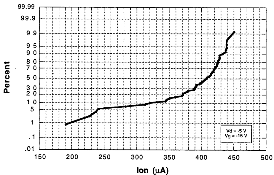
Figure 5-6. Probability distribution for drive current in W/L = 10\mu\text{m}/4\mu\text{m} transistors.
