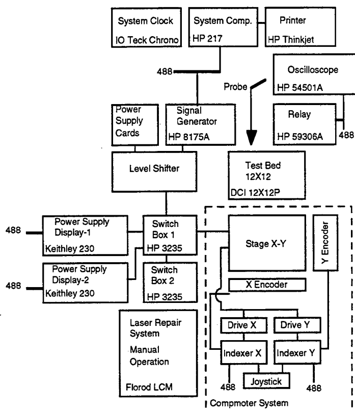
Figure 7-5. Equipment diagram for shorts and functional testing.
