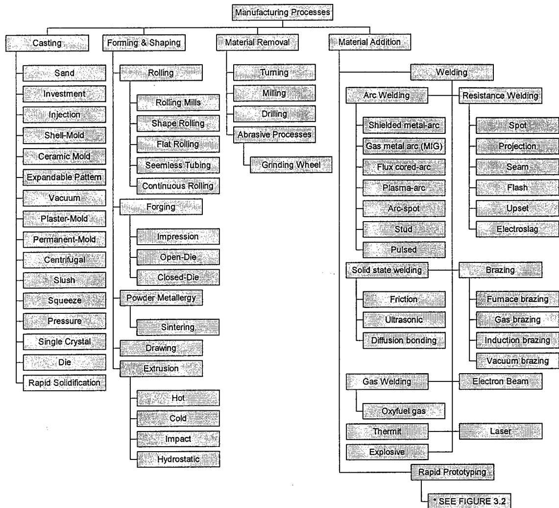
Figure 3.1 Manufacturing Process Organizational Chart
