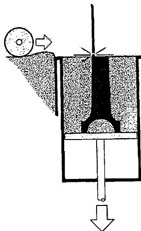
Figure 3.5 Selective Laser Sintering Process (Computer Aided Rapid Prototyping, 1996)
