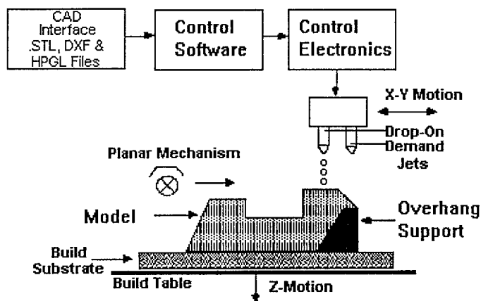
Figure 3.8 Inkjet Modeling Technology (Model-Maker 3D Modeling System, 1996)
