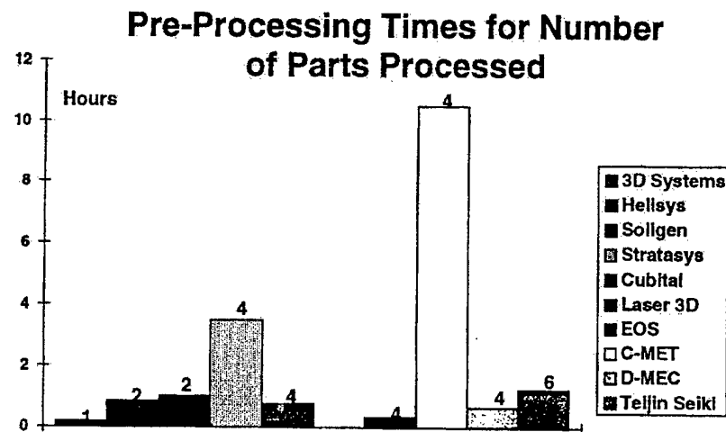
Figure 5.2 Pre-Processing Time (Aubin, 1994)
