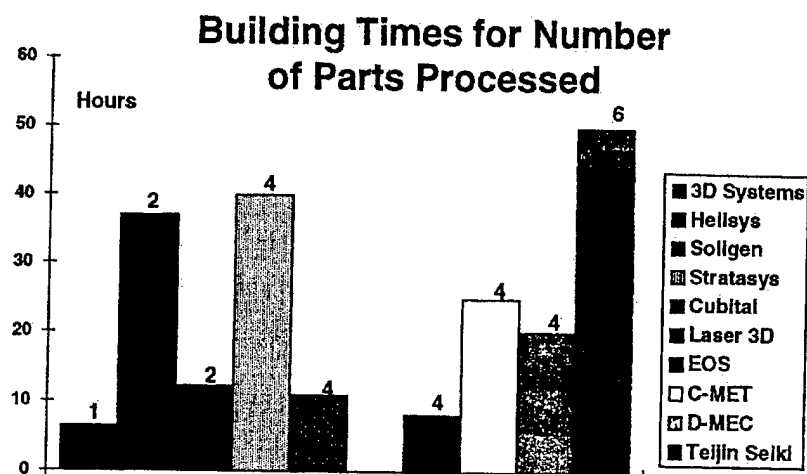
Figure 5.3 Run Time (Aubin, 1994)
