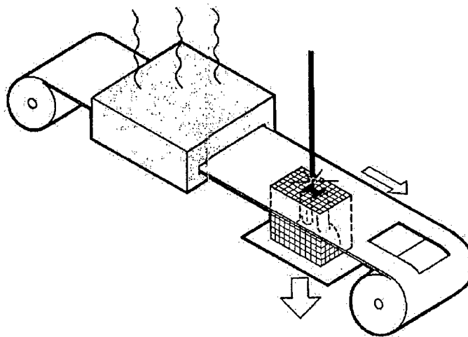
Figure 3.6 Laminated Object Manufacturing Process (Computer Aided Rapid Prototyping, 1996)
