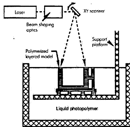
Figure 3.4 StereoLithography Process (Thomas, 1995)
