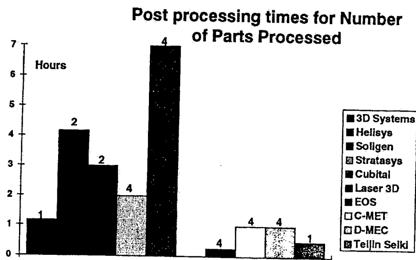
Figure 5.4 Post-Processing Time (Aubin, 1994)
