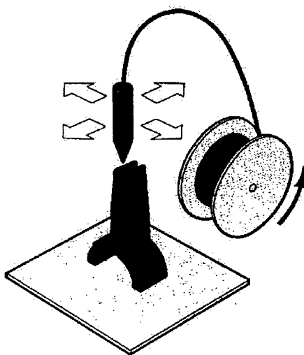
Figure 3.7 Fused Deposition Modeling Process (Computer Aided Rapid Prototyping, 1996)
