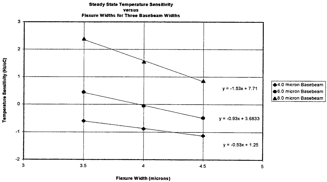
Figure 3.11: SOA FEA Temperature Sensitivity versus Flexure Width
