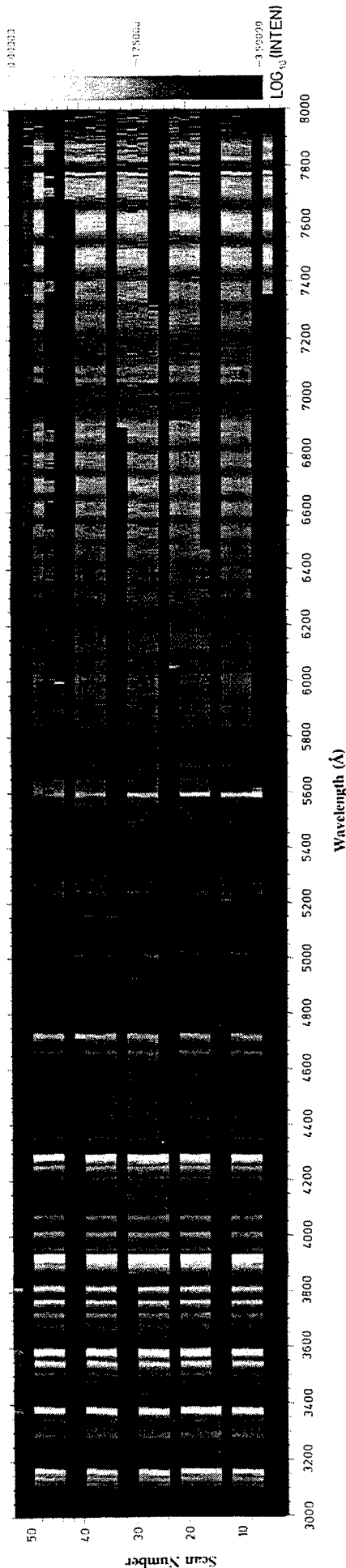
Plate 4: EXCEDE III unattenuated visible spectra (3000-8000 Å). N.B.: All spectral scans in Plates 3 and 4 have been normalized using their associated 3914 Å borosight photometers and have been referenced to the N 2 (ZP) 0-1 emission at 4278 Å.
