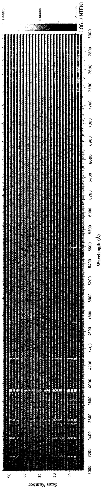
Plate 2: EXCEDE III visible spectral scans (3000-8900 Å).
