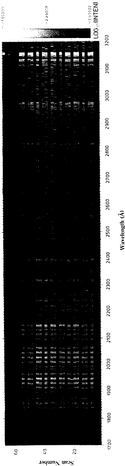
Plate 3: EXCEDE III unattenuated UV spectra (1800-3100 Å).
