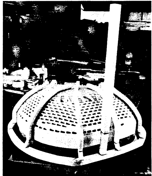
Figure 9.—Hatch plate pattern formed over sand core fixture with gating.
